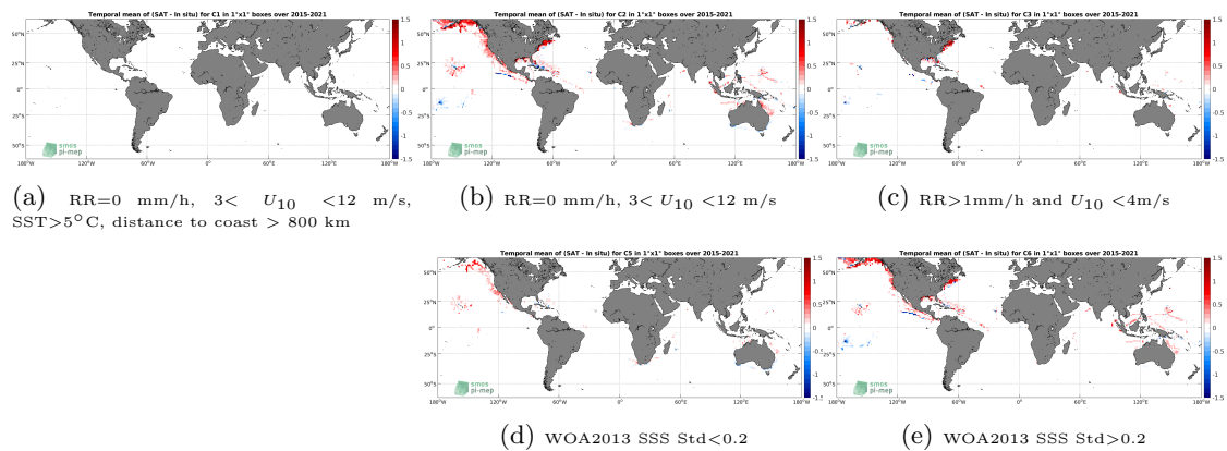
Figure 12: Temporal mean gridded over spatial boxes of size 1^\circ \times 1^\circ of \Delta\text{SSS} (SMAP SSS L3 v5.0 - Monthly (JPL) - TSG (SAMOS)) for 5 different subdatasets corresponding to:RR=0 mm/h, 3 < U_{10} < 12 m/s, SST >5^\circ\text{C} , distance to coast > 800 km (a), RR=0 mm/h, 3 < U_{10} < 12 m/s (b), RR >1 mm/h and U_{10} < 4 m/s (c), WOA2013 SSS Std <0.2 (d), WOA2013 SSS Std >0.2 (e).
