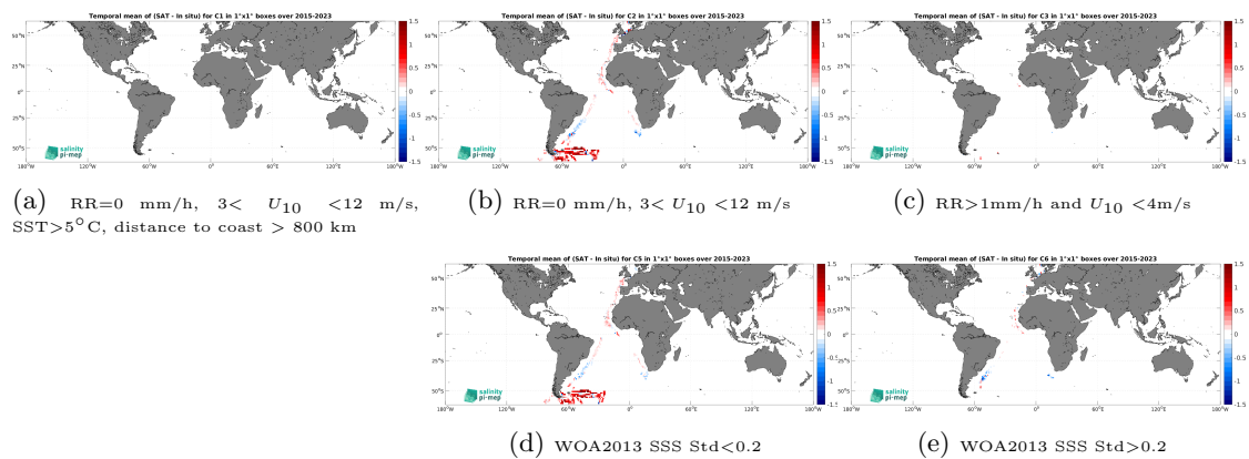
Figure 14: Temporal mean gridded over spatial boxes of size 1^\circ \times 1^\circ of \Delta\text{SSS} (SMAP SSS L3 v5.0 - Monthly (JPL) - TSG (Polarstern)) for 5 different subdatasets corresponding to:RR=0 mm/h, 3 < U_{10} < 12 m/s, SST>5°C, distance to coast > 800 km (a), RR=0 mm/h, 3 < U_{10} < 12 m/s (b), RR>1mm/h and U_{10} < 4 m/s (c), WOA2013 SSS Std<0.2 (d), WOA2013 SSS Std>0.2 (e).
