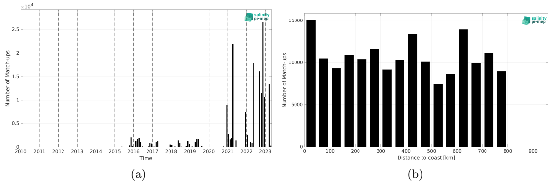
Figure 2: Number of match-ups between TSG (Polarstern) and SMAP SSS L3 v5.0 - Monthly (JPL) SSS as a function of time (a) and as function of the distance to coast (b) over the SMOS coastal zone (<800km) 60N-60S Pi-MEP region and for the full satellite product period.
