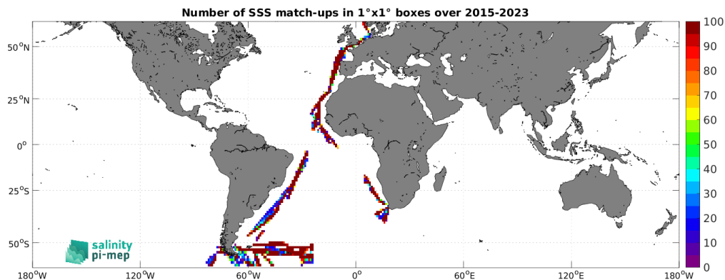
Figure 5: Number of SSS match-ups between TSG (Polarstern) SSS and the SMAP SSS L3 v5.0 - Monthly (JPL) SSS product for the SMOS coastal zone (<800km) 60N-60S Pi-MEP region over 1^\circ \times 1^\circ boxes and for the full satellite product period.
