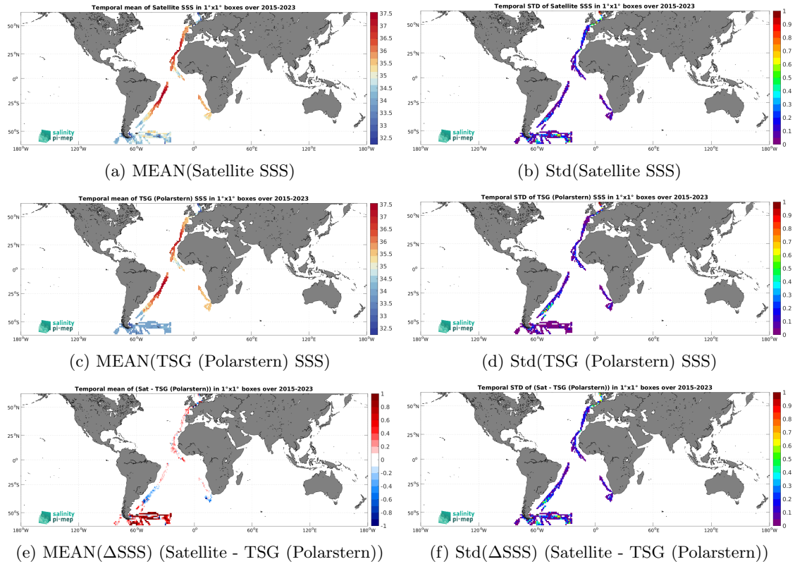
Figure 7: Temporal mean (left) and Std (right) of SSS from SMAP SSS L3 v5.0 - Monthly (JPL) (top), TSG (Polarstern) (middle), and of \Delta SSS (Satellite - TSG (Polarstern)). Only match-up pairs are used to generate these maps.
