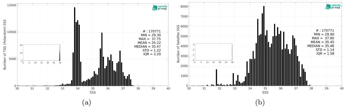
Figure 3: Histograms of SSS from TSG (Polarstern) (a) and SMAP SSS L3 v5.0 - Monthly (JPL) (b) considering all match-up pairs per bins of 0.1 over the SMOS coastal zone (<800km) 60N-60S Pi-MEP region and for the full satellite product period.
