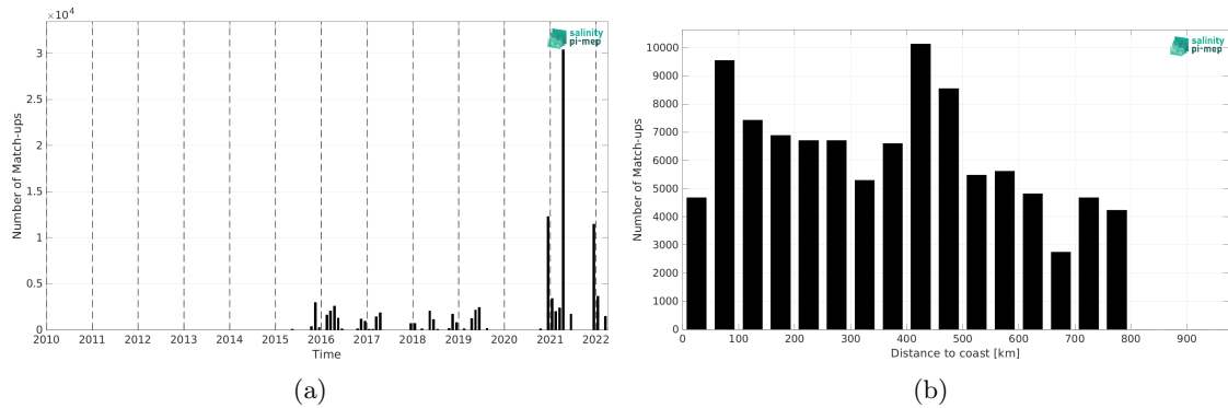
Figure 1: Number of match-ups between TSG (Polarstern) and SMAP SSS L3 v5.0 - Monthly (JPL) SSS as a function of time (a) and as function of the distance to coast (b) over the SMOS coastal zone (<800km) 60N-60S Pi-MEP region and for the full satellite product period.
