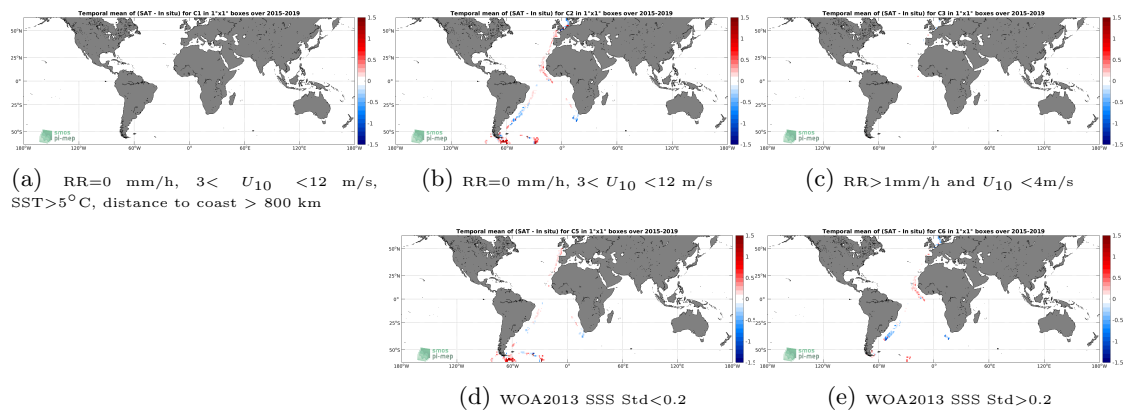
Figure 12: Temporal mean gridded over spatial boxes of size 1^\circ \times 1^\circ of \Delta SSS (SMAP SSS L3 v5.0 - Monthly (JPL) - TSG (Polarstern)) for 5 different subdatasets corresponding to: RR=0 mm/h, 3 < U_{10} < 12 m/s, SST > 5°C, distance to coast > 800 km (a), RR=0 mm/h, 3 < U_{10} < 12 m/s (b), RR > 1mm/h and U_{10} < 4 m/s (c), WOA2013 SSS Std < 0.2 (d), WOA2013 SSS Std > 0.2 (e).
