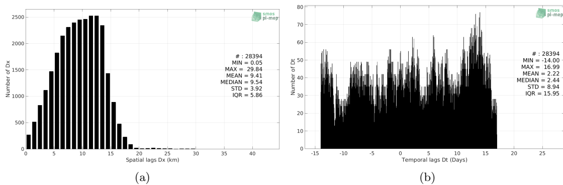
Figure 5: Histograms of the spatial (a) and temporal (b) lags between the time of the TSG (Polarstern) measurements and the date of the corresponding SMAP SSS L3 v5.0 - Monthly (JPL) SSS product.
