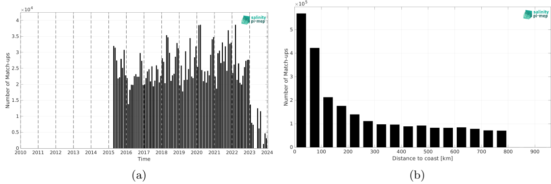
Figure 2: Number of match-ups between TSG (LEGOS-DM) and SMAP SSS L3 v5.0 - Monthly (JPL) SSS as a function of time (a) and as function of the distance to coast (b) over the SMOS coastal zone (<800km) 60N-60S Pi-MEP region and for the full satellite product period.
