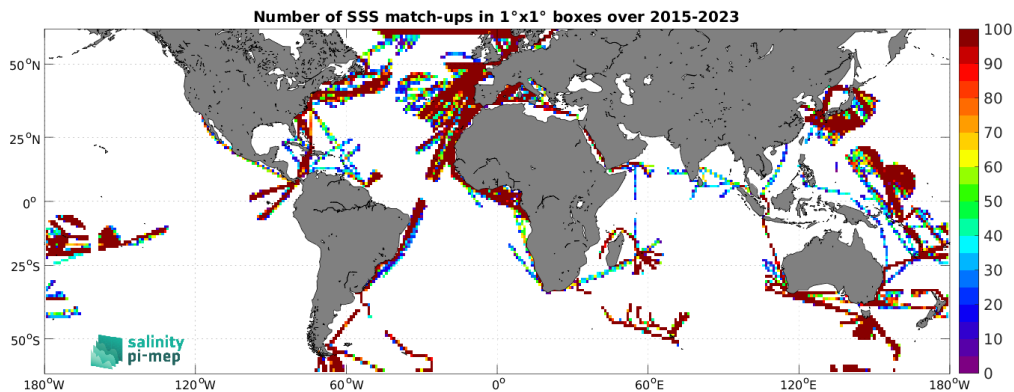
Figure 5: Number of SSS match-ups between TSG (LEGOS-DM) SSS and the SMAP SSS L3 v5.0 - Monthly (JPL) SSS product for the SMOS coastal zone (<800km) 60N-60S Pi-MEP region over 1^\circ \times 1^\circ boxes and for the full satellite product period.
