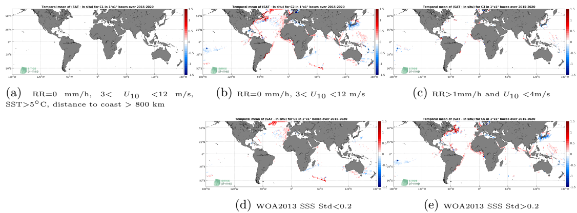
Figure 12: Temporal mean gridded over spatial boxes of size 1^\circ \times 1^\circ of \Delta SSS (SMAP SSS L3 v5.0 - Monthly (JPL) - TSG (LEGOS-DM)) for 5 different subdatasets corresponding to:RR=0 mm/h, 3 < U_{10} < 12 m/s, SST >5^\circ\text{C} , distance to coast > 800 km (a), RR=0 mm/h, 3 < U_{10} < 12 m/s (b), RR >1 mm/h and U_{10} < 4 m/s (c), WOA2013 SSS Std <0.2 (d), WOA2013 SSS Std >0.2 (e).
