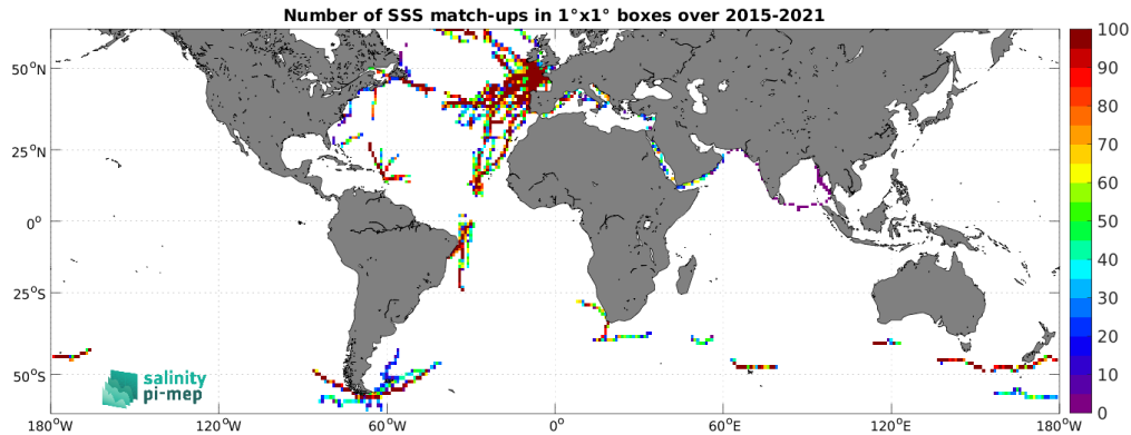
Figure 5: Number of SSS match-ups between TSG (GOSUD-Sailing-ship) SSS and the SMAP SSS L3 v5.0 - Monthly (JPL) SSS product for the SMOS coastal zone (<800km) 60N-60S Pi-MEP region over 1^{\circ} \times 1^{\circ} boxes and for the full satellite product period.
