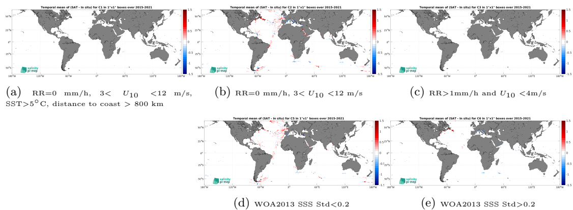
Figure 14: Temporal mean gridded over spatial boxes of size 1^\circ \times 1^\circ of \Delta SSS (SMAP SSS L3 v5.0 - Monthly (JPL) - TSG (GOSUD-Sailing-ship)) for 5 different subdatasets corresponding to: RR=0 mm/h, 3 < U_{10} < 12 m/s, SST > 5^\circ\text{C} , distance to coast > 800 km (a), RR=0 mm/h, 3 < U_{10} < 12 m/s (b), RR > 1 mm/h and U_{10} < 4 m/s (c), WOA2013 SSS Std < 0.2 (d), WOA2013 SSS Std > 0.2 (e).
