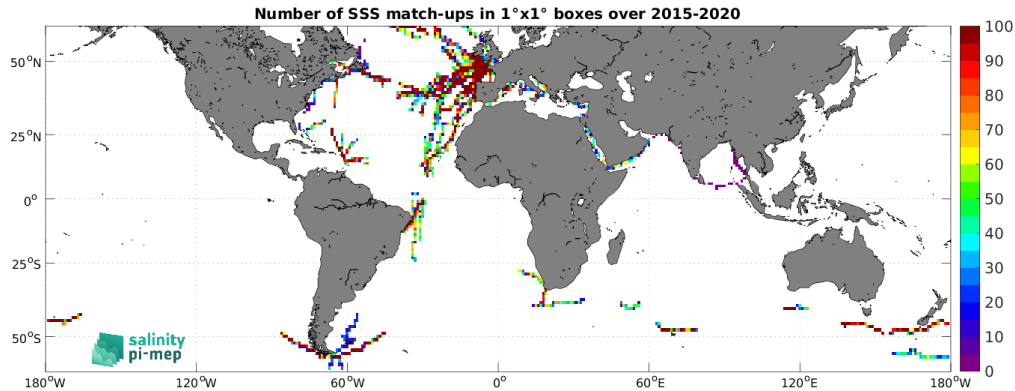
Figure 5: Number of SSS match-ups between TSG (GOSUD-Sailing-ship) SSS and the SMAP SSS L3 v5.0 - Monthly (JPL) SSS product for the SMOS coastal zone (<800km) 60N-60S Pi-MEP region over 1^\circ \times 1^\circ boxes and for the full satellite product period.
