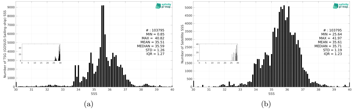
Figure 3: Histograms of SSS from TSG (GOSUD-Sailing-ship) (a) and SMAP SSS L3 v5.0 - Monthly (JPL) (b) considering all match-up pairs per bins of 0.1 over the SMOS coastal zone (<800km) 60N-60S Pi-MEP region and for the full satellite product period.
