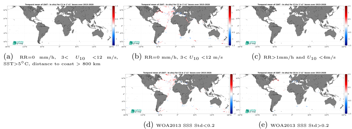
Figure 14: Temporal mean gridded over spatial boxes of size 1^\circ \times 1^\circ of \Delta\text{SSS} (SMAP SSS L3 v5.0 - Monthly (JPL) - TSG (GOSUD-Sailing-ship)) for 5 different subdatasets corresponding to: RR=0 mm/h, 3 < U_{10} < 12 m/s, SST > 5°C, distance to coast > 800 km (a), RR=0 mm/h, 3 < U_{10} < 12 m/s (b), RR > 1mm/h and U_{10} < 4 m/s (c), WOA2013 SSS Std < 0.2 (d), WOA2013 SSS Std > 0.2 (e).
