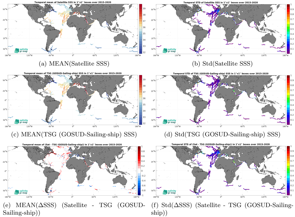
Figure 7: Temporal mean (left) and Std (right) of SSS from SMAP SSS L3 v5.0 - Monthly (JPL) (top), TSG (GOSUD-Sailing-ship) (middle), and of \Delta SSS (Satellite - TSG (GOSUD-Sailing-ship)). Only match-up pairs are used to generate these maps.
