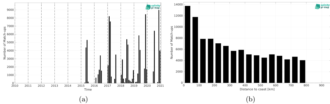
Figure 2: Number of match-ups between TSG (GOSUD-Sailing-ship) and SMAP SSS L3 v5.0 - Monthly (JPL) SSS as a function of time (a) and as function of the distance to coast (b) over the SMOS coastal zone (<800km) 60N-60S Pi-MEP region and for the full satellite product period.
