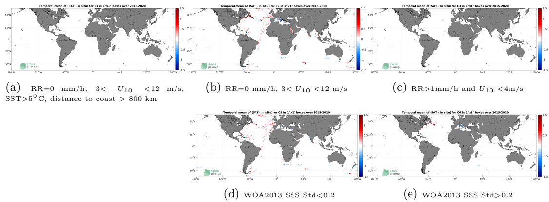
Figure 12: Temporal mean gridded over spatial boxes of size 1^\circ \times 1^\circ of \Delta SSS (SMAP SSS L3 v5.0 - Monthly (JPL) - TSG (GOSUD-Sailing-ship)) for 5 different subdatasets corresponding to:RR=0 mm/h, 3 < U_{10} < 12 m/s, SST >5^\circ C, distance to coast > 800 km (a), RR=0 mm/h, 3 < U_{10} < 12 m/s (b), RR >1 mm/h and U_{10} < 4 m/s (c), WOA2013 SSS Std <0.2 (d), WOA2013 SSS Std >0.2 (e).
