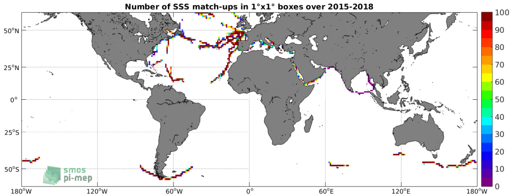
Figure 4: Number of SSS match-ups between TSG (GOSUD-Sailing-ship) SSS and the SMAP SSS L3 v5.0 - Monthly (JPL) SSS product for the SMOS coastal zone (<800km) 60N-60S Pi-MEP region over 1^{\circ} \times 1^{\circ} boxes and for the full satellite product period.
