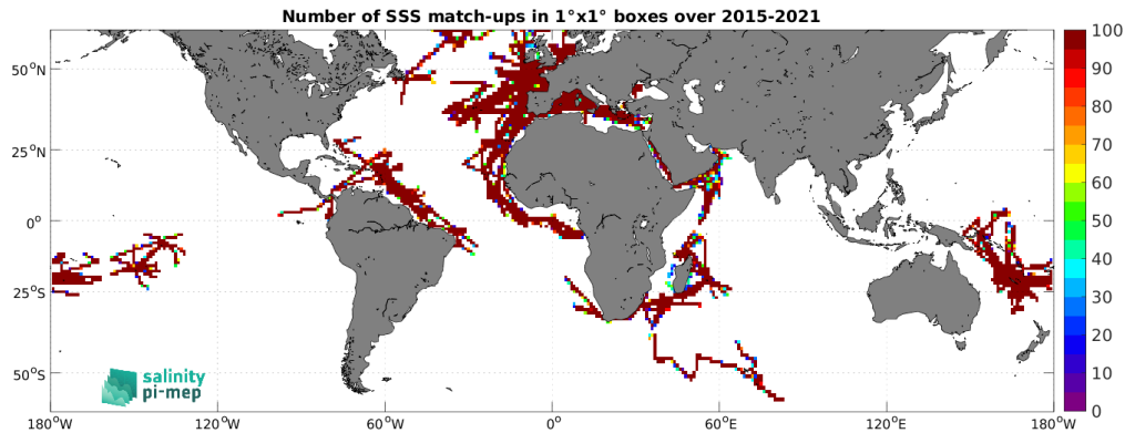
Figure 4: Number of SSS match-ups between TSG (GOSUD-Research-vessel) SSS and the SMAP SSS L3 v5.0 - Monthly (JPL) SSS product for the SMOS coastal zone ( <800\text{km} ) 60\text{N} - 60\text{S} Pi-MEP region over 1^\circ \times 1^\circ boxes and for the full satellite product period.
