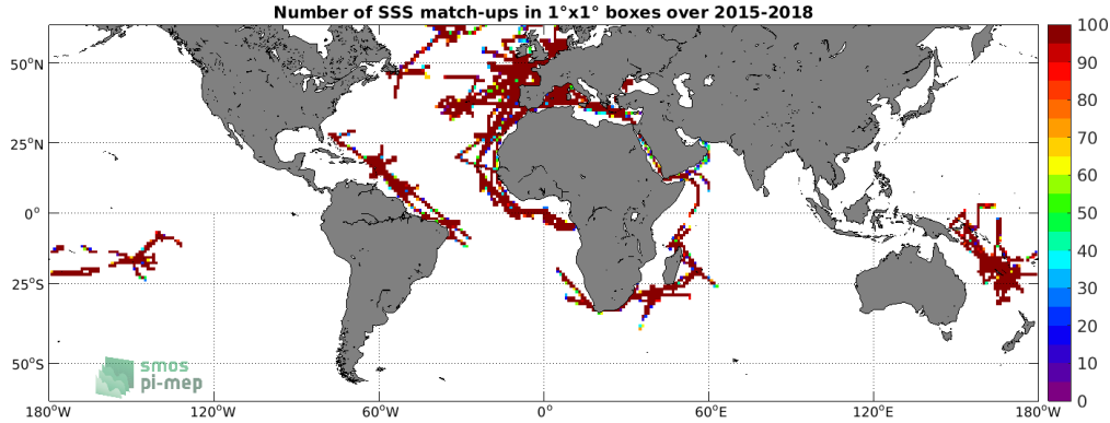
Figure 4: Number of SSS match-ups between TSG (GOSUD-Research-vessel) SSS and the SMAP SSS L3 v5.0 - Monthly (JPL) SSS product for the SMOS coastal zone (<800km) 60N-60S Pi-MEP region over 1°x1° boxes and for the full satellite product period.
