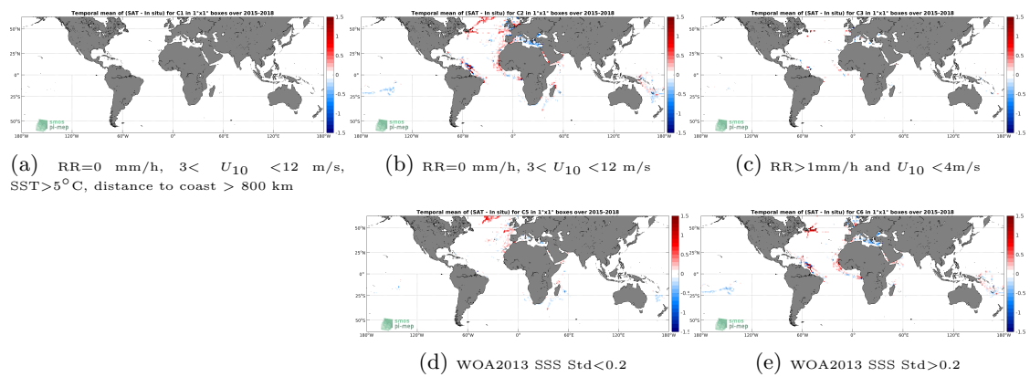
Figure 12: Temporal mean gridded over spatial boxes of size 1°x1° of \Delta SSS (SMAP SSS L3 v5.0 - Monthly (JPL) - TSG (GOSUD-Research-vessel)) for 5 different subdatasets corresponding to:RR=0 mm/h, 3 < U_{10} < 12 m/s, SST>5°C, distance to coast > 800 km (a), RR=0 mm/h, 3 < U_{10} < 12 m/s (b), RR>1mm/h and U_{10} < 4 m/s (c), WOA2013 SSS Std<0.2 (d), WOA2013 SSS Std>0.2 (e).
