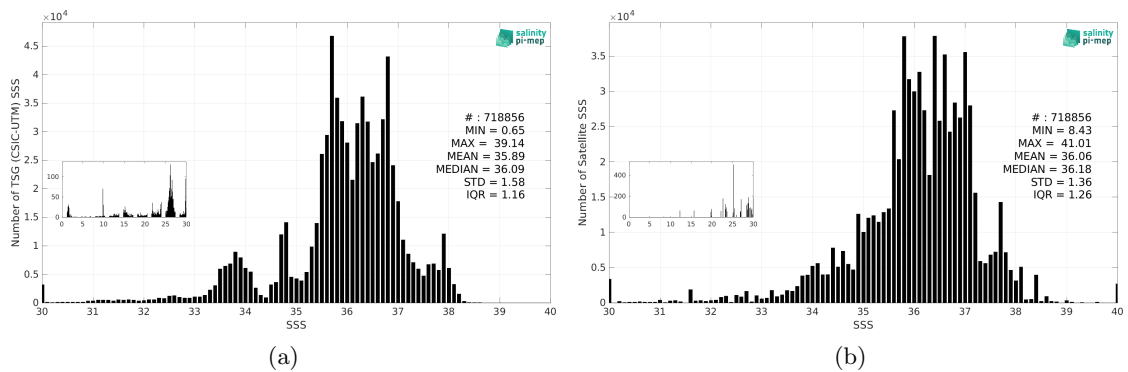
Figure 3: Histograms of SSS from TSG (CSIC-UTM) (a) and SMAP SSS L3 v5.0 - Monthly (JPL) (b) considering all match-up pairs per bins of 0.1 over the SMOS coastal zone (<800km) 60N-60S Pi-MEP region and for the full satellite product period.
