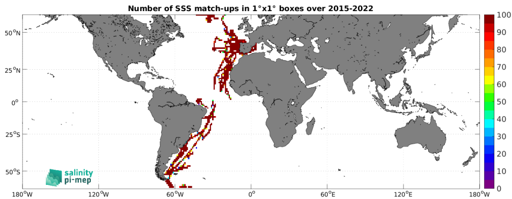
Figure 5: Number of SSS match-ups between TSG (CSIC-UTM) SSS and the SMAP SSS L3 v5.0 - Monthly (JPL) SSS product for the SMOS coastal zone (<800km) 60N-60S Pi-MEP region over 1^\circ \times 1^\circ boxes and for the full satellite product period.
