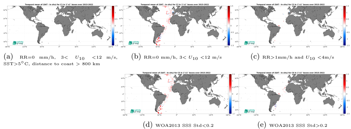
Figure 14: Temporal mean gridded over spatial boxes of size 1^\circ \times 1^\circ of \Delta\text{SSS} (SMAP SSS L3 v5.0 - Monthly (JPL) - TSG (CSIC-UTM)) for 5 different subdatasets corresponding to:RR=0 mm/h, 3 < U_{10} < 12 m/s, SST > 5^\circ\text{C} , distance to coast > 800 km (a), RR=0 mm/h, 3 < U_{10} < 12 m/s (b), RR > 1 mm/h and U_{10} < 4 m/s (c), WOA2013 SSS Std < 0.2 (d), WOA2013 SSS Std > 0.2 (e).
