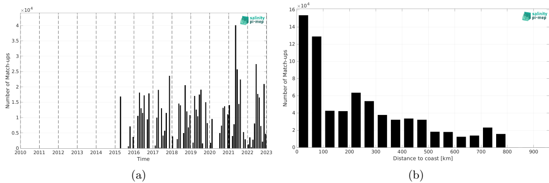
Figure 2: Number of match-ups between TSG (CSIC-UTM) and SMAP SSS L3 v5.0 - Monthly (JPL) SSS as a function of time (a) and as function of the distance to coast (b) over the SMOS coastal zone (<800km) 60N-60S Pi-MEP region and for the full satellite product period.
