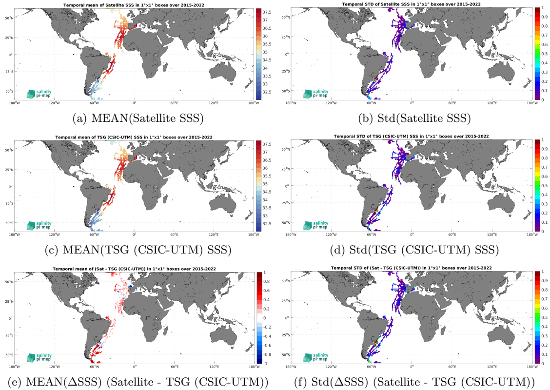
Figure 7: Temporal mean (left) and Std (right) of SSS from SMAP SSS L3 v5.0 - Monthly (JPL) (top), TSG (CSIC-UTM) (middle), and of \Delta SSS (Satellite - TSG (CSIC-UTM)). Only match-up pairs are used to generate these maps.
