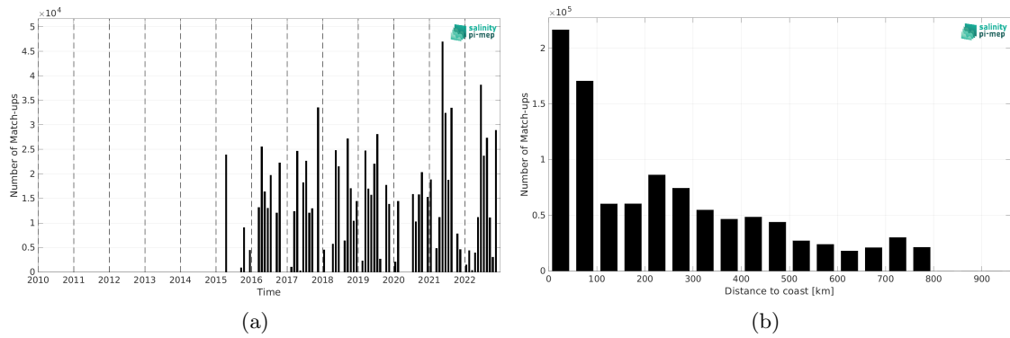
Figure 1: Number of match-ups between TSG (CSIC-UTM) and SMAP SSS L3 v5.0 - Monthly (JPL) SSS as a function of time (a) and as function of the distance to coast (b) over the SMOS coastal zone (<800km) 60N-60S Pi-MEP region and for the full satellite product period.
