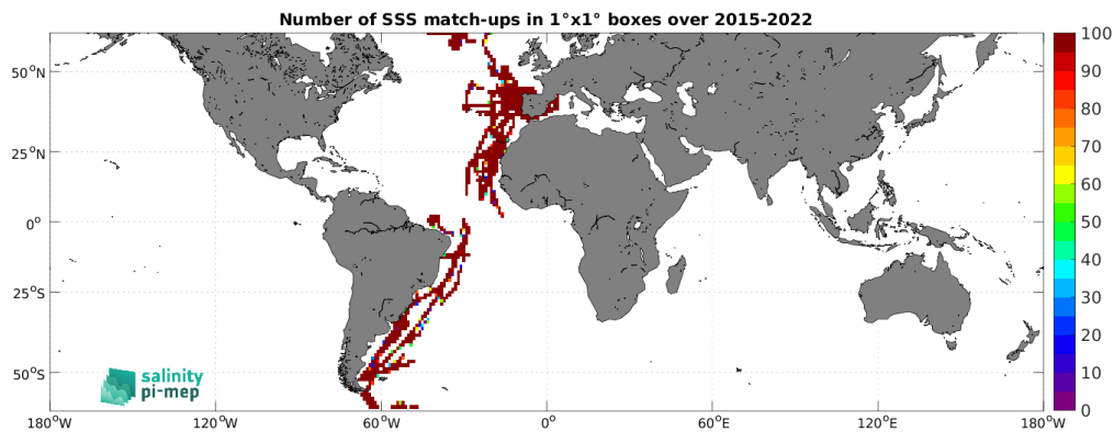
Figure 4: Number of SSS match-ups between TSG (CSIC-UTM) SSS and the SMAP SSS L3 v5.0 - Monthly (JPL) SSS product for the SMOS coastal zone (<800km) 60N-60S Pi-MEP region over 1^\circ \times 1^\circ boxes and for the full satellite product period.
