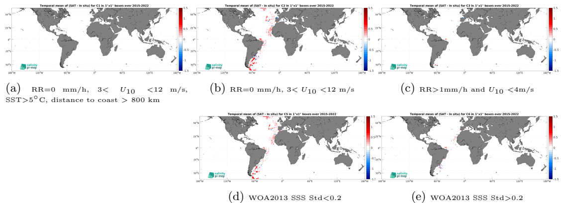
Figure 12: Temporal mean gridded over spatial boxes of size 1^\circ \times 1^\circ of \Delta SSS (SMAP SSS L3 v5.0 - Monthly (JPL) - TSG (CSIC-UTM)) for 5 different subdatasets corresponding to:RR=0 mm/h, 3 < U_{10} < 12 m/s, SST >5^\circ\text{C} , distance to coast > 800 km (a), RR=0 mm/h, 3 < U_{10} < 12 m/s (b), RR >1 mm/h and U_{10} < 4 m/s (c), WOA2013 SSS Std <0.2 (d), WOA2013 SSS Std >0.2 (e).
