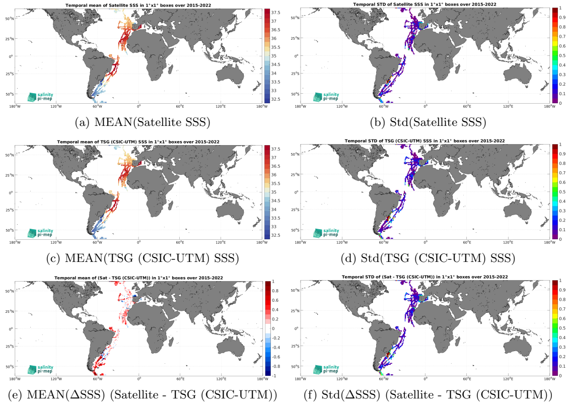
Figure 6: Temporal mean (left) and Std (right) of SSS from SMAP SSS L3 v5.0 - Monthly (JPL) (top), TSG (CSIC-UTM) (middle), and of \Delta SSS (Satellite - TSG (CSIC-UTM)). Only match-up pairs are used to generate these maps.
