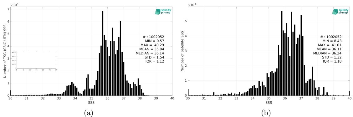
Figure 2: Histograms of SSS from TSG (CSIC-UTM) (a) and SMAP SSS L3 v5.0 - Monthly (JPL) (b) considering all match-up pairs per bins of 0.1 over the SMOS coastal zone (<800km) 60N-60S Pi-MEP region and for the full satellite product period.
