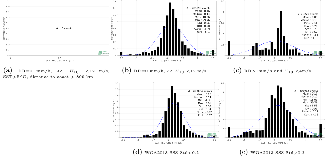
Figure 13: Normalized histogram of \Delta SSS (SMAP SSS L3 v5.0 - Monthly (JPL) - TSG (CSIC-UTM)) for 5 different subdatasets corresponding to: RR=0 mm/h, 3 < U_{10} < 12 m/s, SST > 5°C, distance to coast > 800 km (a), RR=0 mm/h, 3 < U_{10} < 12 m/s (b), RR > 1mm/h and U_{10} < 4 m/s (c), WOA2013 SSS Std < 0.2 (d), WOA2013 SSS Std > 0.2 (e).
