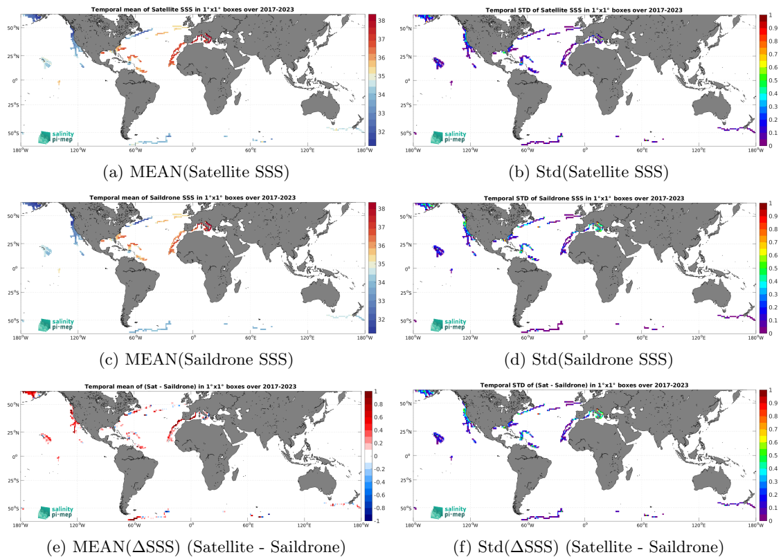
Figure 7: Temporal mean (left) and Std (right) of SSS from SMAP SSS L3 v5.0 - Monthly (JPL) (top), Saildrone (middle), and of \Delta SSS (Satellite - Saildrone). Only match-up pairs are used to generate these maps.
