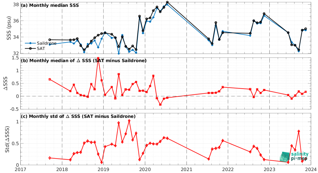
Figure 8: Time series of the monthly median SSS (top), median of \Delta SSS (Satellite - Saildrone) and Std of \Delta SSS (Satellite - Saildrone) over the SMOS coastal zone ( <800\text{km} ) 60\text{N} - 60\text{S} Pi-MEP region considering all match-ups collected by the Pi-MEP.
