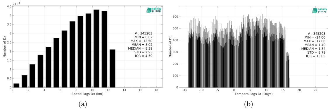
Figure 6: Histograms of the spatial (a) and temporal (b) lags between the location/time of the Saildrone measurement and the date of the corresponding SMAP SSS L3 v5.0 - Monthly (JPL) SSS pixel.
