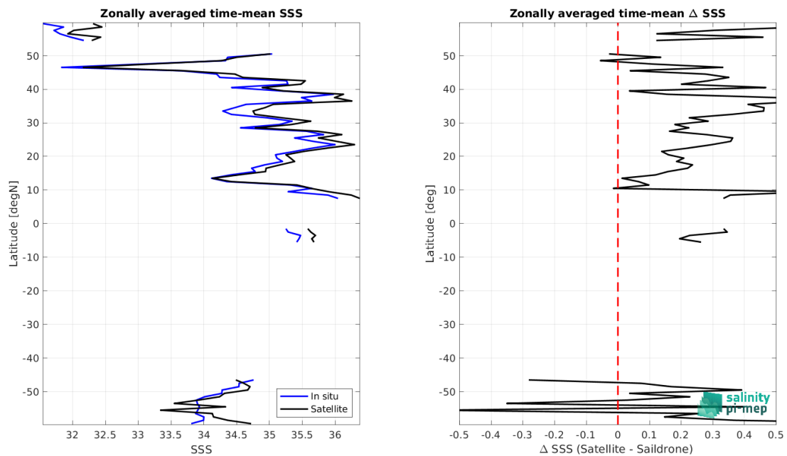
Figure 9: Left panel: Zonal mean SSS from SMAP SSS L3 v5.0 - Monthly (JPL) satellite product (black) and from Sairdrone (blue). Right panel: Zonal mean of \Delta SSS (Satellite - Sairdrone) for all the collected Pi-MEP match-up pairs estimated over the full satellite product period.
