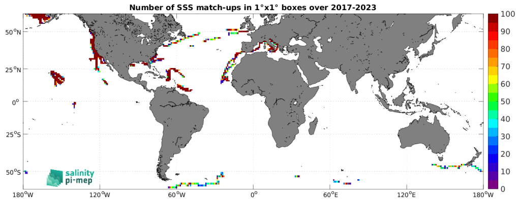
Figure 5: Number of SSS match-ups between Saildrone SSS and the SMAP SSS L3 v5.0 - Monthly (JPL) SSS product for the SMOS coastal zone (<800km) 60N-60S Pi-MEP region over 1^\circ \times 1^\circ boxes and for the full satellite product period.
