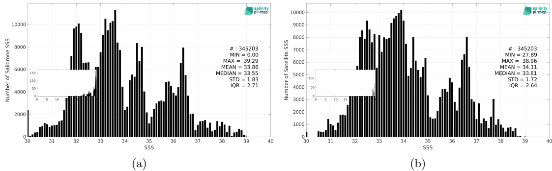
Figure 3: Histograms of SSS from Saildrone (a) and SMAP SSS L3 v5.0 - Monthly (JPL) (b) considering all match-up pairs per bins of 0.1 over the SMOS coastal zone (<800km) 60N-60S Pi-MEP region and for the full satellite product period.
