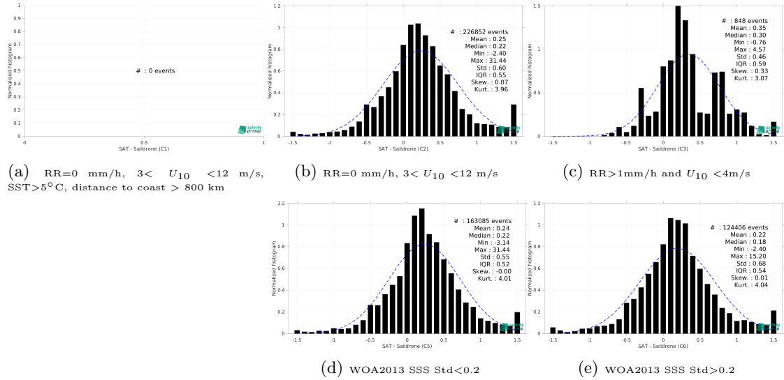
Figure 15: Normalized histogram of \Delta SSS (SMAP SSS L3 v5.0 - Monthly (JPL) - Sairdrone) for 5 different subdatasets corresponding to: RR=0 mm/h, 3 < U_{10} < 12 m/s, SST > 5°C, distance to coast > 800 km (a), RR=0 mm/h, 3 < U_{10} < 12 m/s (b), RR > 1mm/h and U_{10} < 4 m/s (c), WOA2013 SSS Std < 0.2 (d), WOA2013 SSS Std > 0.2 (e).
