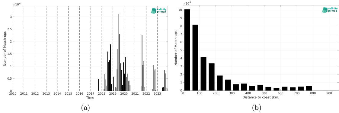
Figure 2: Number of match-ups between Saildrone and SMAP SSS L3 v5.0 - Monthly (JPL) SSS as a function of time (a) and as function of the distance to coast (b) over the SMOS coastal zone (<800km) 60N-60S Pi-MEP region and for the full satellite product period.
