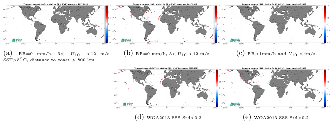
Figure 14: Temporal mean gridded over spatial boxes of size 1^\circ \times 1^\circ of \Delta SSS (SMAP SSS L3 v5.0 - Monthly (JPL) - Saildrone) for 5 different subdatasets corresponding to:RR=0 mm/h, 3 < U_{10} < 12 m/s, SST>5°C, distance to coast > 800 km (a), RR=0 mm/h, 3 < U_{10} < 12 m/s (b), RR>1mm/h and U_{10} < 4 m/s (c), WOA2013 SSS Std<0.2 (d), WOA2013 SSS Std>0.2 (e).
