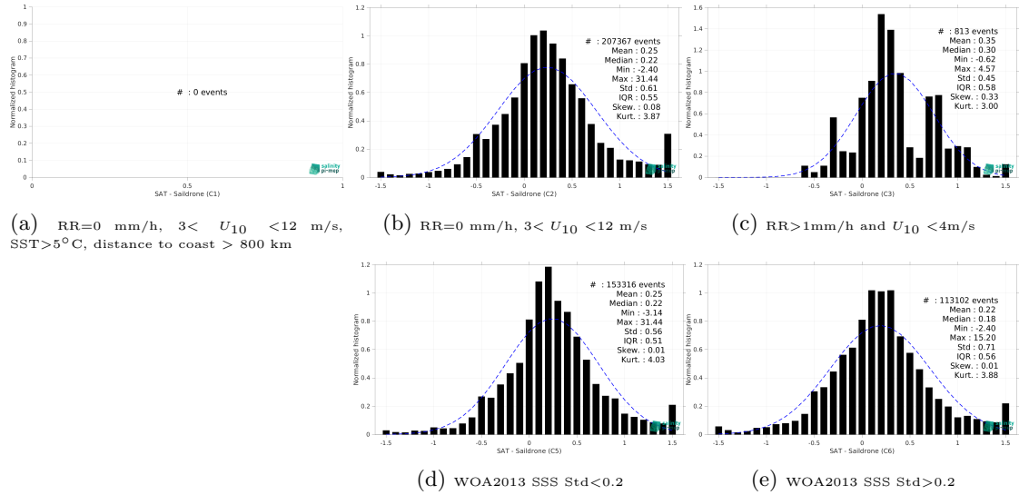
Figure 15: Normalized histogram of \Delta SSS (SMAP SSS L3 v5.0 - Monthly (JPL) - Saldrone) for 5 different subdatasets corresponding to: RR=0 mm/h, 3 < U_{10} < 12 m/s, SST > 5°C, distance to coast > 800 km (a), RR=0 mm/h, 3 < U_{10} < 12 m/s (b), RR > 1mm/h and U_{10} < 4 m/s (c), WOA2013 SSS Std < 0.2 (d), WOA2013 SSS Std > 0.2 (e).
