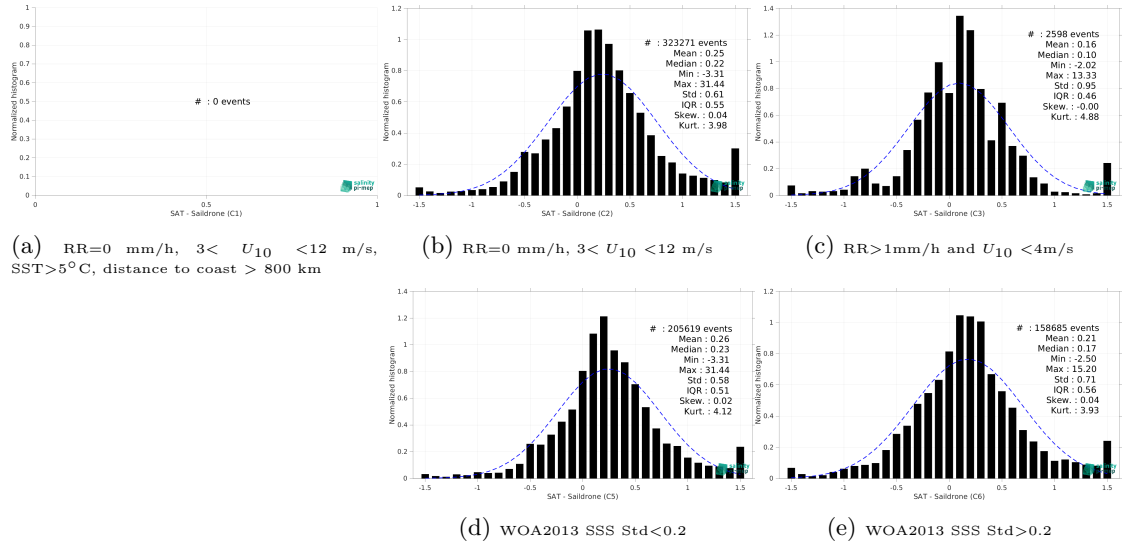
Figure 13: Normalized histogram of \Delta SSS (SMAP SSS L3 v5.0 - Monthly (JPL) - Sairdrone) for 5 different subdatasets corresponding to: RR=0 mm/h, 3 < U_{10} < 12 m/s, SST > 5°C, distance to coast > 800 km (a), RR=0 mm/h, 3 < U_{10} < 12 m/s (b), RR > 1mm/h and U_{10} < 4 m/s (c), WOA2013 SSS Std < 0.2 (d), WOA2013 SSS Std > 0.2 (e).
