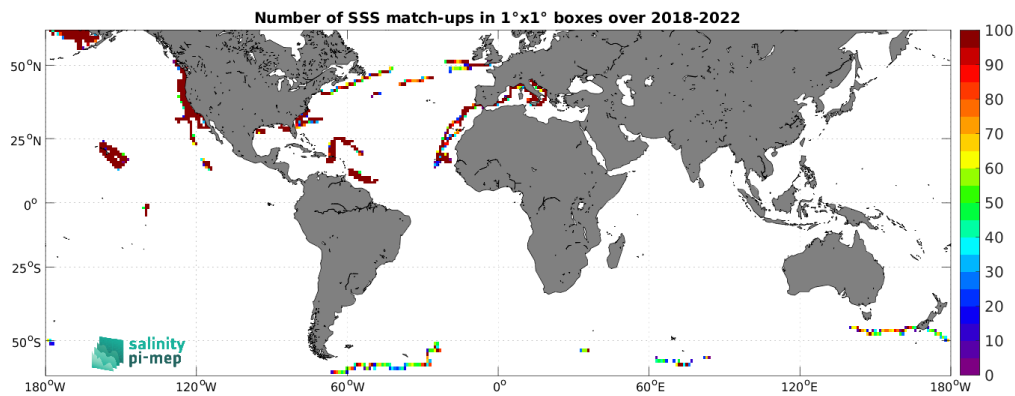
Figure 4: Number of SSS match-ups between Saildrone SSS and the SMAP SSS L3 v5.0 - Monthly (JPL) SSS product for the SMOS coastal zone (<800km) 60N-60S Pi-MEP region over 1^\circ \times 1^\circ boxes and for the full satellite product period.
