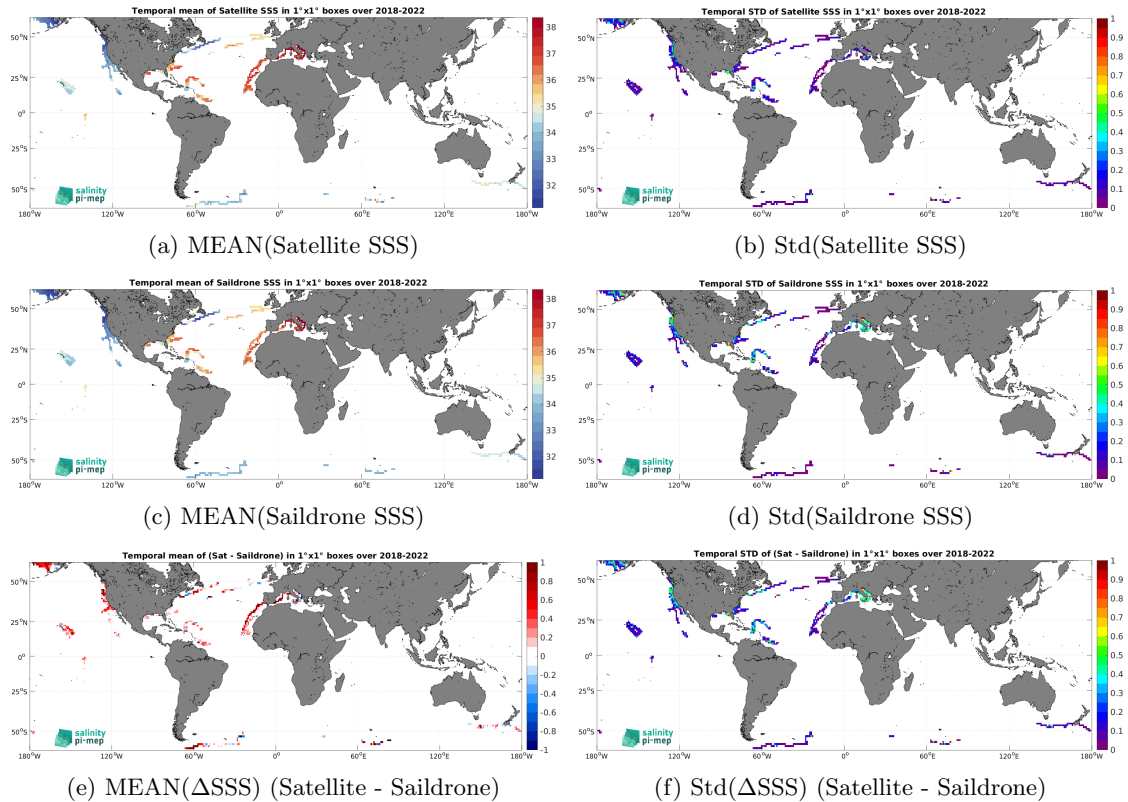
Figure 6: Temporal mean (left) and Std (right) of SSS from SMAP SSS L3 v5.0 - Monthly (JPL) (top), Saildrone (middle), and of \Delta SSS (Satellite - Saildrone). Only match-up pairs are used to generate these maps.
