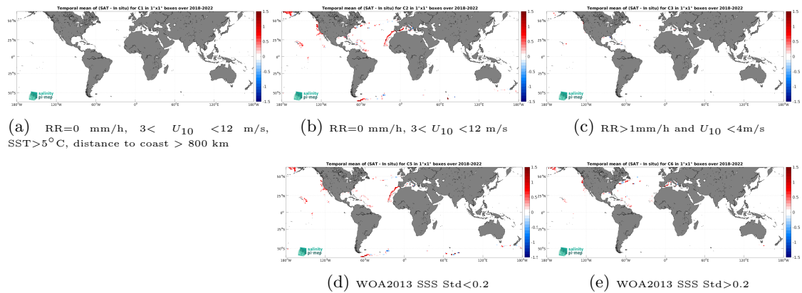
Figure 12: Temporal mean gridded over spatial boxes of size 1^\circ \times 1^\circ of \Delta SSS (SMAP SSS L3 v5.0 - Monthly (JPL) - Saildrone) for 5 different subdatasets corresponding to:RR=0 mm/h, 3 < U_{10} < 12 m/s, SST >5^\circ\text{C} , distance to coast > 800 km (a), RR=0 mm/h, 3 < U_{10} < 12 m/s (b), RR >1 mm/h and U_{10} < 4 m/s (c), WOA2013 SSS Std <0.2 (d), WOA2013 SSS Std >0.2 (e).
