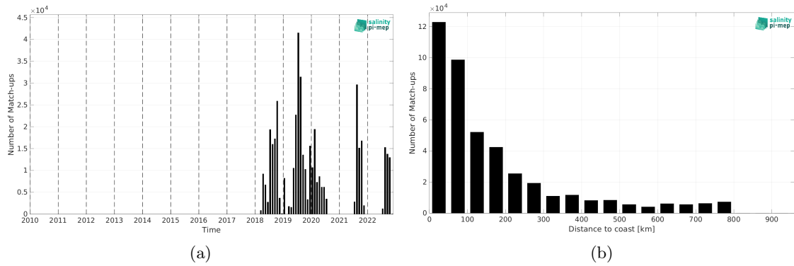
Figure 1: Number of match-ups between Saildrone and SMAP SSS L3 v5.0 - Monthly (JPL) SSS as a function of time (a) and as function of the distance to coast (b) over the SMOS coastal zone (<800km) 60N-60S Pi-MEP region and for the full satellite product period.
