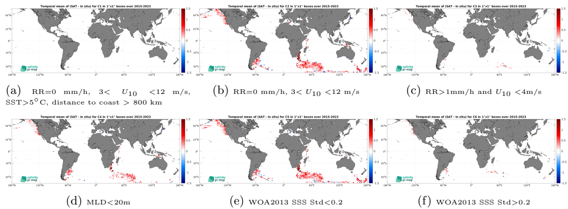
Figure 14: Temporal mean gridded over spatial boxes of size 1^\circ \times 1^\circ of \Delta SSS (SMAP SSS L3 v5.0 - Monthly (JPL) - Marine mammals) for 6 different subdatasets corresponding to:RR=0 mm/h, 3 < U_{10} < 12 m/s, SST >5^\circ C, distance to coast > 800 km (a), RR=0 mm/h, 3 < U_{10} < 12 m/s (b), RR >1 mm/h and U_{10} < 4 m/s (c),MLD <20 m (d),WOA2013 SSS Std <0.2 (e),WOA2013 SSS Std >0.2 (f).
