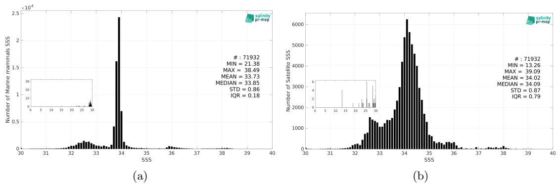
Figure 3: Histograms of SSS from Marine mammals (a) and SMAP SSS L3 v5.0 - Monthly (JPL) (b) considering all match-up pairs per bins of 0.1 over the SMOS coastal zone (<800km) 60N-60S Pi-MEP region and for the full satellite product period.
