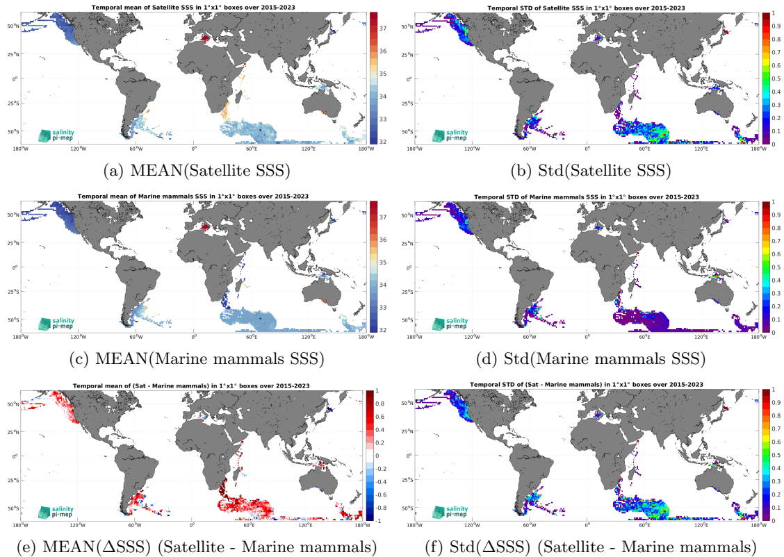
Figure 7: Temporal mean (left) and Std (right) of SSS from SMAP SSS L3 v5.0 - Monthly (JPL) (top), Marine mammals (middle), and of \Delta SSS (Satellite - Marine mammals). Only match-up pairs are used to generate these maps.
