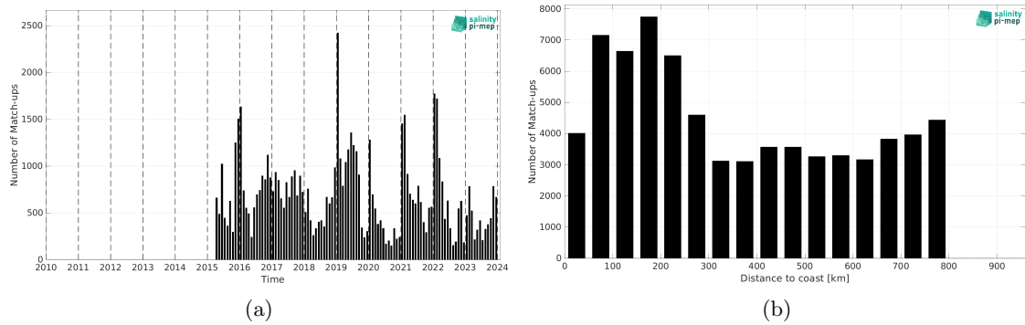
Figure 2: Number of match-ups between Marine mammals and SMAP SSS L3 v5.0 - Monthly (JPL) SSS as a function of time (a) and as function of the distance to coast (b) over the SMOS coastal zone (<800km) 60N-60S Pi-MEP region and for the full satellite product period.
