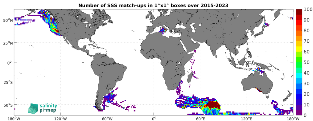
Figure 5: Number of SSS match-ups between Marine mammals SSS and the SMAP SSS L3 v5.0 - Monthly (JPL) SSS product for the SMOS coastal zone (<800km) 60N-60S Pi-MEP region over 1^\circ \times 1^\circ boxes and for the full satellite product period.
