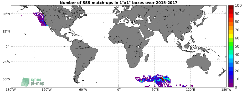
Figure 4: Number of SSS match-ups between Sea mammals SSS and the SMAP SSS L3 v5.0 - Monthly (JPL) SSS product for the SMOS coastal zone (<800km) 60N-60S Pi-MEP region over 1°x1° boxes and for the full satellite product period.
