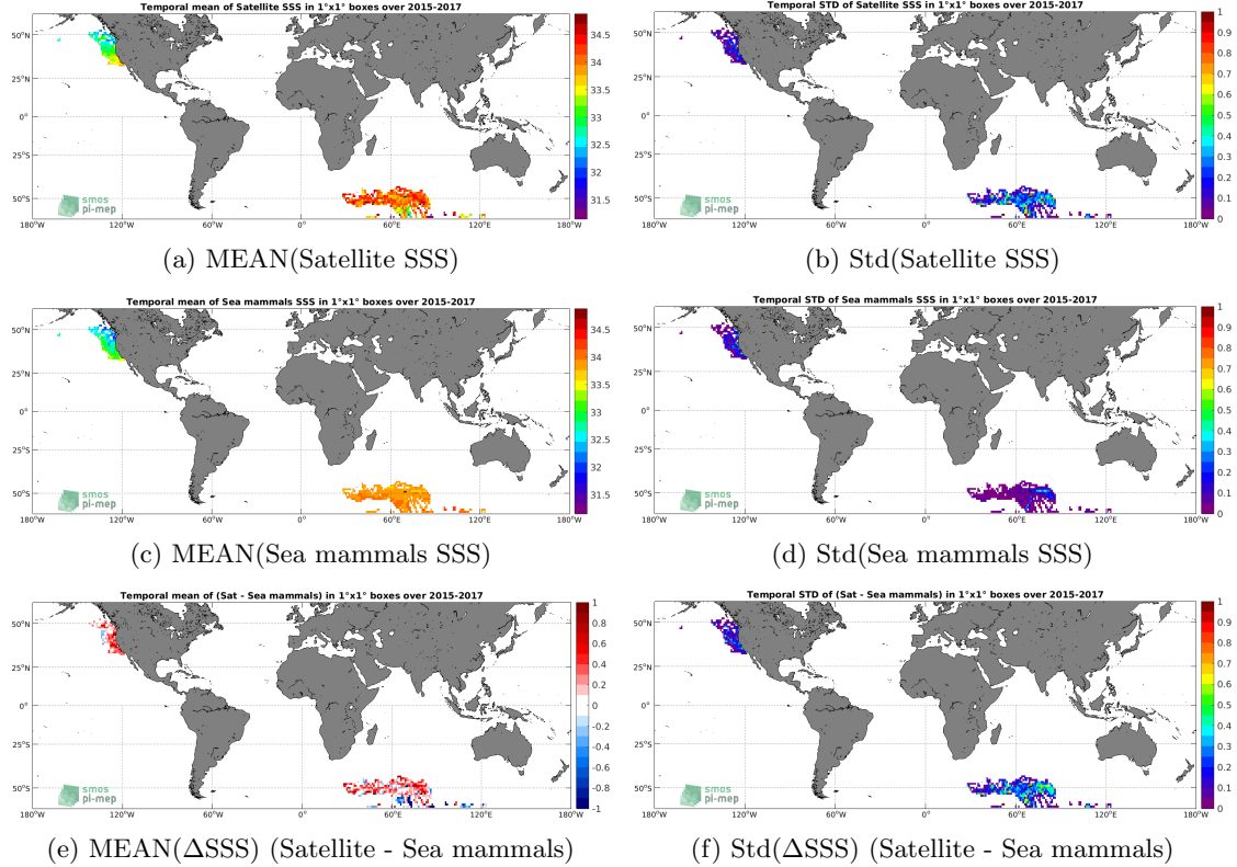
Figure 6: Temporal mean (left) and Std (right) of SSS from SMAP SSS L3 v5.0 - Monthly (JPL) (top), Sea mammals (middle), and of \Delta SSS (Satellite - Sea mammals). Only match-up pairs are used to generate these maps.
