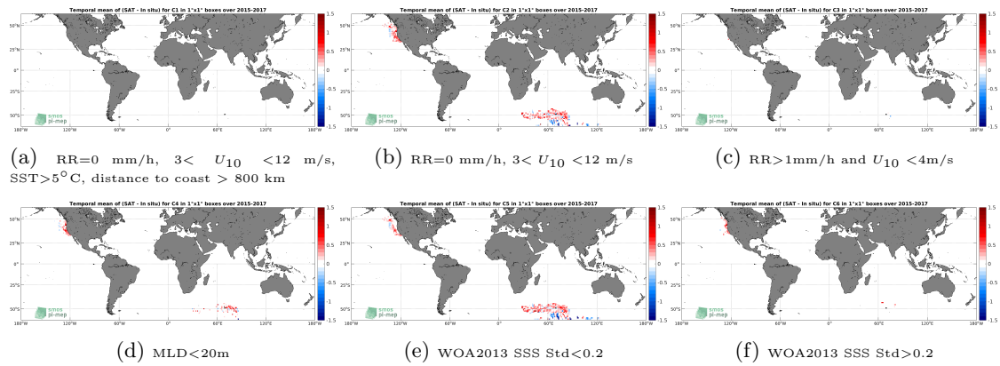
Figure 12: Temporal mean gridded over spatial boxes of size 1^\circ \times 1^\circ of \Delta SSS (SMAP SSS L3 v5.0 - Monthly (JPL) - Sea mammals) for 6 different subdatasets corresponding to:RR=0 mm/h, 3 < U_{10} < 12 m/s, SST > 5^\circ\text{C} , distance to coast > 800 km (a), RR=0 mm/h, 3 < U_{10} < 12 m/s (b), RR > 1 mm/h and U_{10} < 4 m/s (c),MLD < 20 m (d),WOA2013 SSS Std < 0.2 (e),WOA2013 SSS Std > 0.2 (f).
