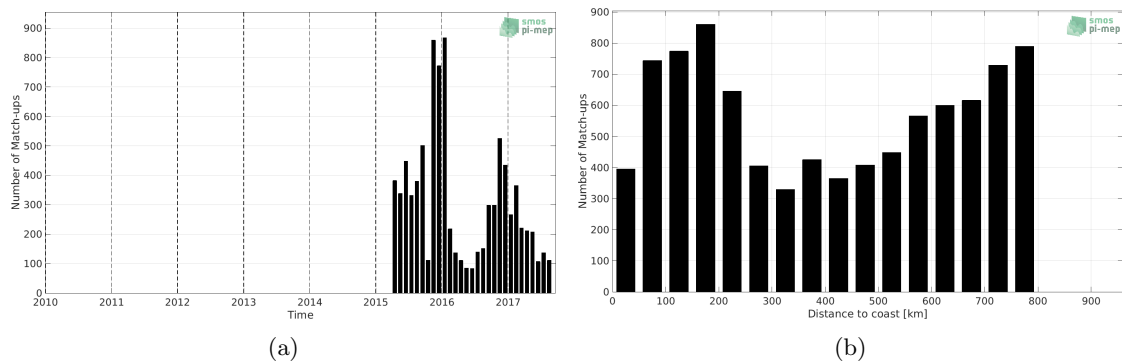
Figure 1: Number of match-ups between Sea mammals and SMAP SSS L3 v5.0 - Monthly (JPL) SSS as a function of time (a) and as function of the distance to coast (b) over the SMOS coastal zone (<800km) 60N-60S Pi-MEP region and for the full satellite product period.
