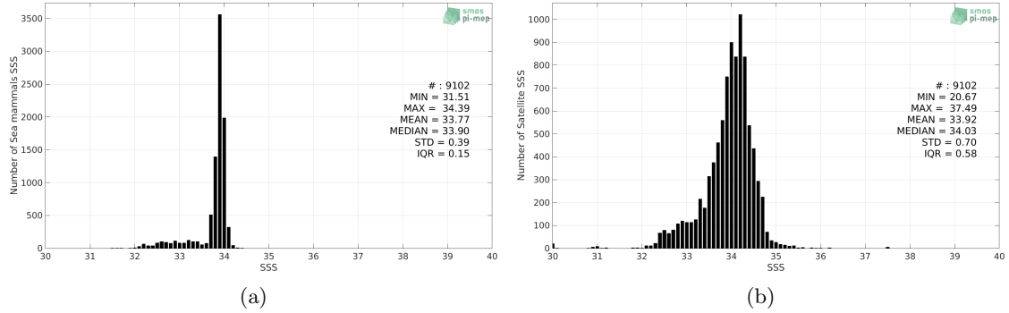
Figure 2: Histograms of SSS from Sea mammals (a) and SMAP SSS L3 v5.0 - Monthly (JPL) (b) considering all match-up pairs per bins of 0.1 over the SMOS coastal zone (<800km) 60N-60S Pi-MEP region and for the full satellite product period.
