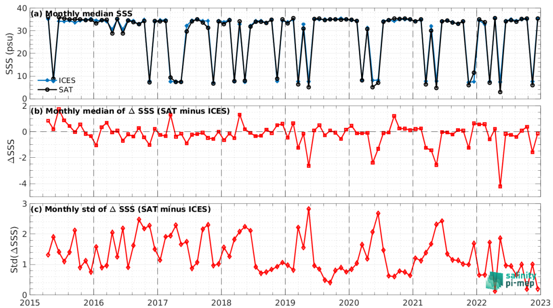
Figure 8: Time series of the monthly median SSS (top), median of \Delta SSS (Satellite - ICES) and Std of \Delta SSS (Satellite - ICES) over the SMOS coastal zone (<800km) 60N-60S Pi-MEP region considering all match-ups collected by the Pi-MEP.
