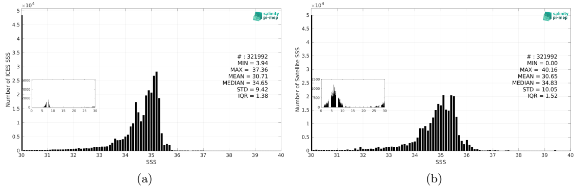
Figure 3: Histograms of SSS from ICES (a) and SMAP SSS L3 v5.0 - Monthly (JPL) (b) considering all match-up pairs per bins of 0.1 over the SMOS coastal zone (<800km) 60N-60S Pi-MEP region and for the full satellite product period.
