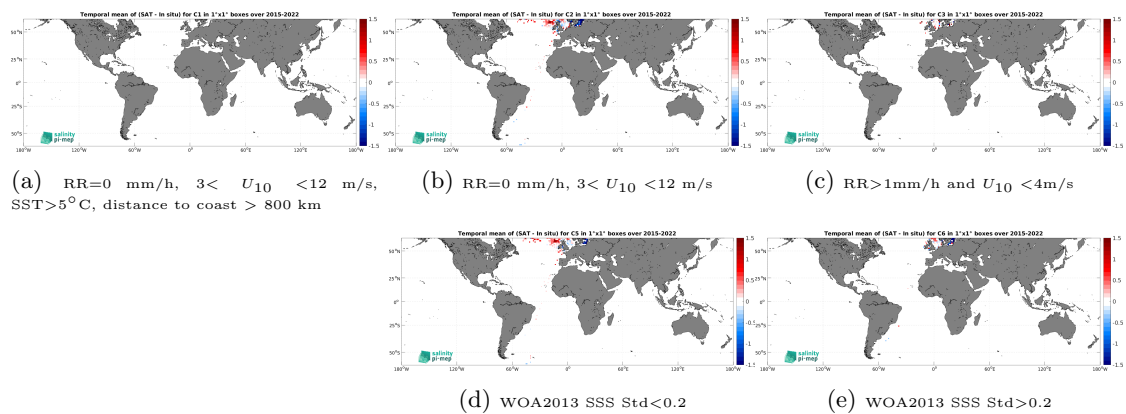
Figure 14: Temporal mean gridded over spatial boxes of size 1^\circ \times 1^\circ of \Delta\text{SSS} (SMAP SSS L3 v5.0 - Monthly (JPL) - ICES) for 5 different subdatasets corresponding to:RR=0 mm/h, 3 < U_{10} < 12 m/s, SST >5^\circ\text{C} , distance to coast > 800 km (a), RR=0 mm/h, 3 < U_{10} < 12 m/s (b), RR >1 mm/h and U_{10} < 4 m/s (c), WOA2013 SSS Std <0.2 (d), WOA2013 SSS Std >0.2 (e).
