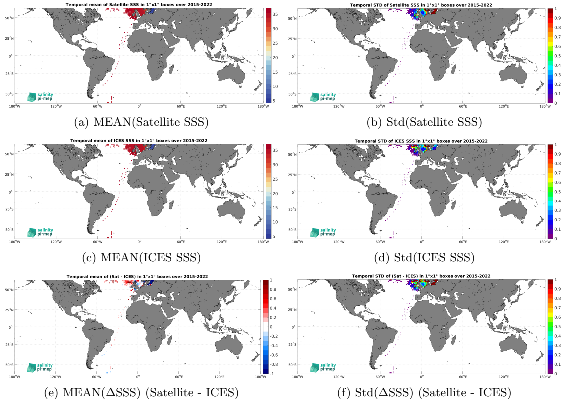
Figure 7: Temporal mean (left) and Std (right) of SSS from SMAP SSS L3 v5.0 - Monthly (JPL) (top), ICES (middle), and of \Delta SSS (Satellite - ICES). Only match-up pairs are used to generate these maps.
