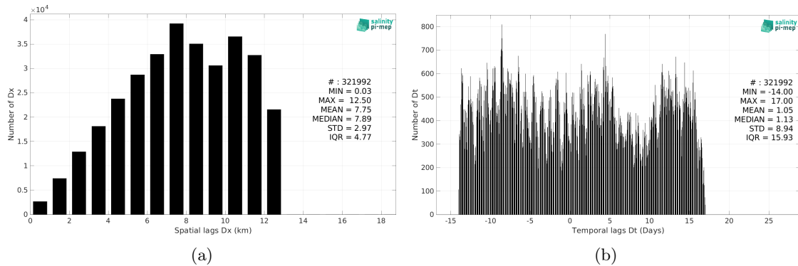
Figure 6: Histograms of the spatial (a) and temporal (b) lags between the location/time of the ICES measurement and the date of the corresponding SMAP SSS L3 v5.0 - Monthly (JPL) SSS pixel.
