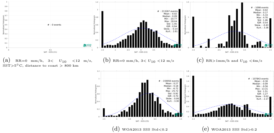
Figure 15: Normalized histogram of \Delta SSS (SMAP SSS L3 v5.0 - Monthly (JPL) - ICES) for 5 different subdatasets corresponding to: RR=0 mm/h, 3 < U_{10} < 12 m/s, SST > 5°C, distance to coast > 800 km (a), RR=0 mm/h, 3 < U_{10} < 12 m/s (b), RR > 1mm/h and U_{10} < 4 m/s (c), WOA2013 SSS Std < 0.2 (d), WOA2013 SSS Std > 0.2 (e).
