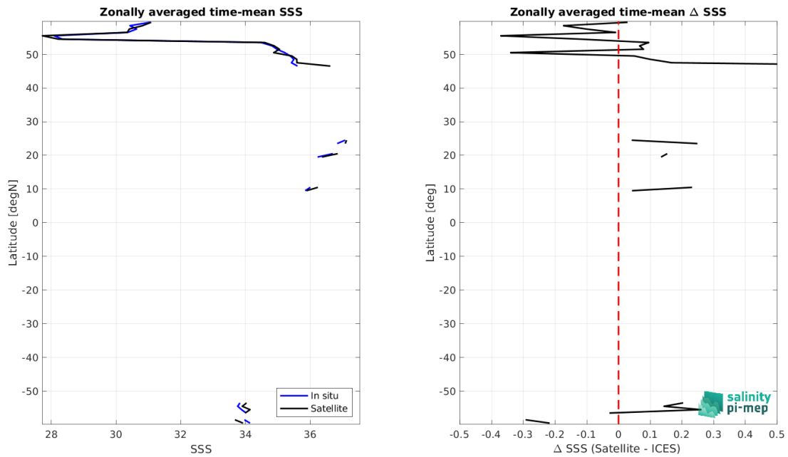
Figure 9: Left panel: Zonal mean SSS from SMAP SSS L3 v5.0 - Monthly (JPL) satellite product (black) and from ICES (blue). Right panel: Zonal mean of \Delta SSS (Satellite - ICES) for all the collected Pi-MEP match-up pairs estimated over the full satellite product period.
