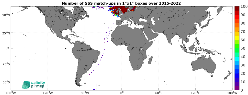
Figure 5: Number of SSS match-ups between ICES SSS and the SMAP SSS L3 v5.0 - Monthly (JPL) SSS product for the SMOS coastal zone (<800km) 60N-60S Pi-MEP region over 1^\circ \times 1^\circ boxes and for the full satellite product period.
