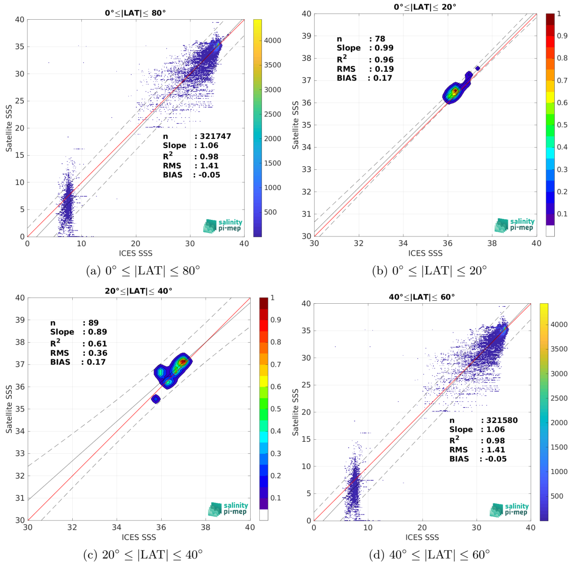
Figure 10: Contour maps of the concentration of SMAP SSS L3 v5.0 - Monthly (JPL) SSS (y-axis) versus ICES SSS (x-axis) at match-up pairs for different latitude bands. For each plot, the red line shows x=y . The black thin and dashed lines indicate a linear fit through the data cloud and the \pm 95\% confidence levels, respectively. The number match-up pairs n , the slope and R^2 coefficient of the linear fit, the root mean square (RMS) and the mean bias between satellite and in situ data are indicated for each latitude band in each plots.
