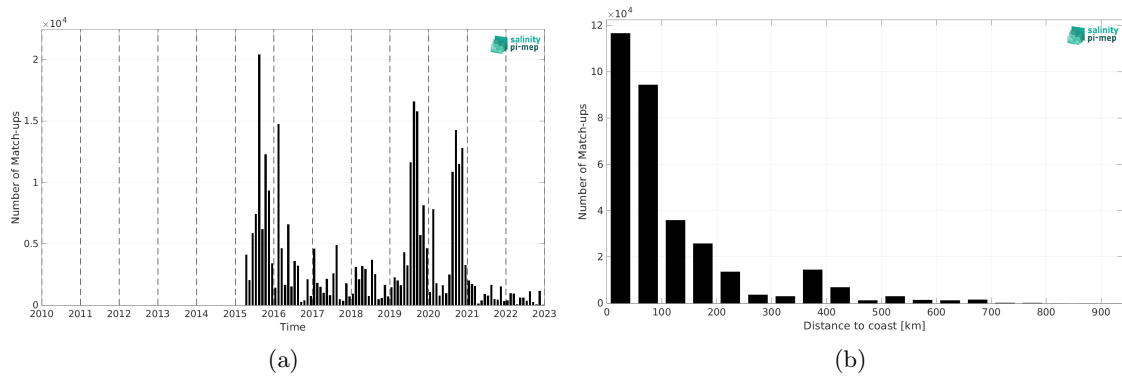
Figure 2: Number of match-ups between ICES and SMAP SSS L3 v5.0 - Monthly (JPL) SSS as a function of time (a) and as function of the distance to coast (b) over the SMOS coastal zone (<800km) 60N-60S Pi-MEP region and for the full satellite product period.
