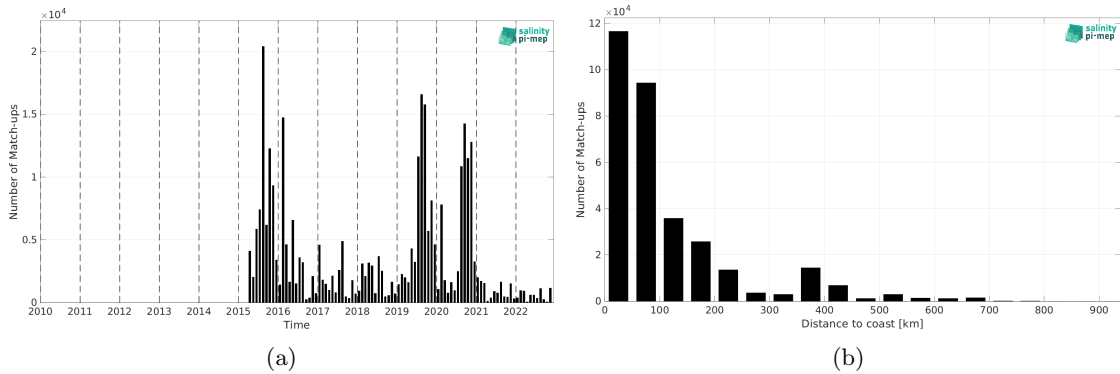
Figure 2: Number of match-ups between ICES and SMAP SSS L3 v5.0 - Monthly (JPL) SSS as a function of time (a) and as function of the distance to coast (b) over the SMOS coastal zone ( < 800\text{km} ) 60\text{N}-60\text{S} Pi-MEP region and for the full satellite product period.
