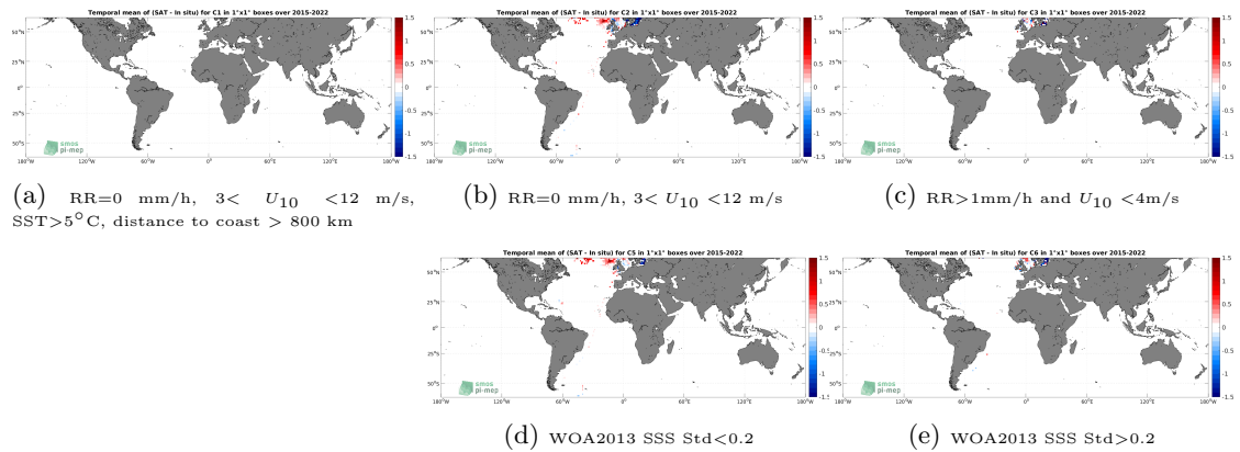
Figure 12: Temporal mean gridded over spatial boxes of size 1^\circ \times 1^\circ of \Delta SSS (SMAP SSS L3 v5.0 - Monthly (JPL) - ICES) for 5 different subdatasets corresponding to:RR=0 mm/h, 3 < U_{10} < 12 m/s, SST >5^\circ\text{C} , distance to coast > 800 km (a), RR=0 mm/h, 3 < U_{10} < 12 m/s (b), RR >1 mm/h and U_{10} < 4 m/s (c), WOA2013 SSS Std <0.2 (d), WOA2013 SSS Std >0.2 (e).
