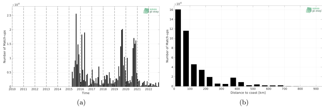
Figure 1: Number of match-ups between ICES and SMAP SSS L3 v5.0 - Monthly (JPL) SSS as a function of time (a) and as function of the distance to coast (b) over the SMOS coastal zone (<800km) 60N-60S Pi-MEP region and for the full satellite product period.
