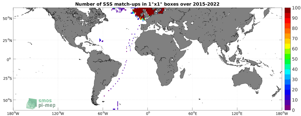
Figure 4: Number of SSS match-ups between ICES SSS and the SMAP SSS L3 v5.0 - Monthly (JPL) SSS product for the SMOS coastal zone (<800km) 60N-60S Pi-MEP region over 1^\circ \times 1^\circ boxes and for the full satellite product period.
