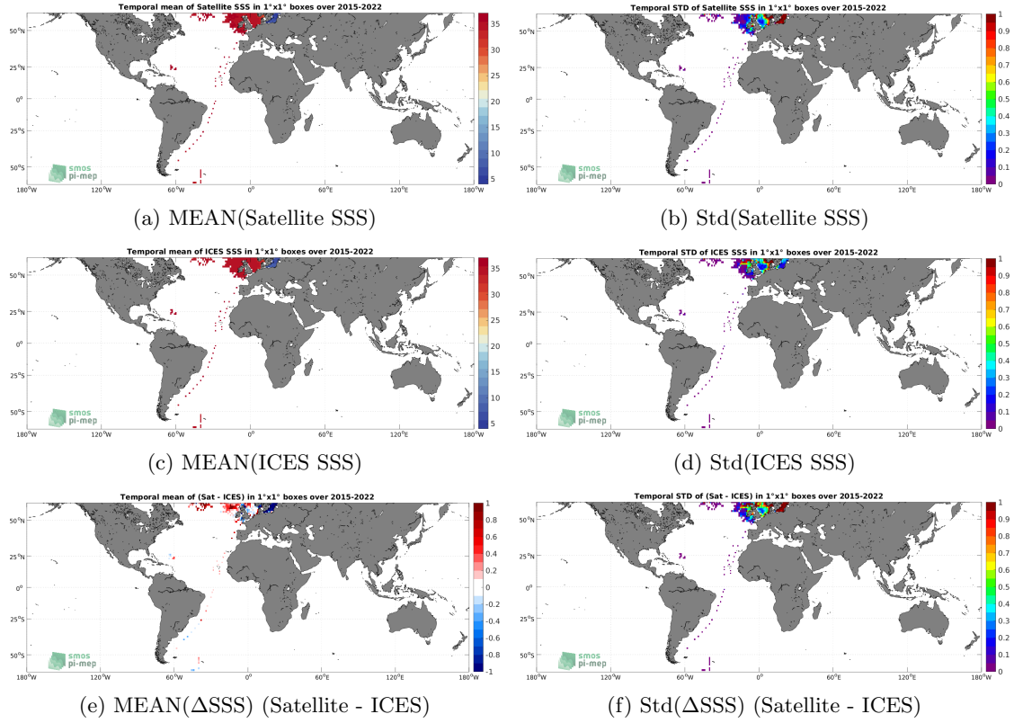
Figure 6: Temporal mean (left) and Std (right) of SSS from SMAP SSS L3 v5.0 - Monthly (JPL) (top), ICES (middle), and of \Delta SSS (Satellite - ICES). Only match-up pairs are used to generate these maps.
