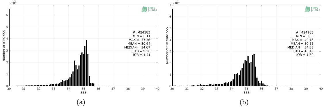
Figure 2: Histograms of SSS from ICES (a) and SMAP SSS L3 v5.0 - Monthly (JPL) (b) considering all match-up pairs per bins of 0.1 over the SMOS coastal zone (<800km) 60N-60S Pi-MEP region and for the full satellite product period.
