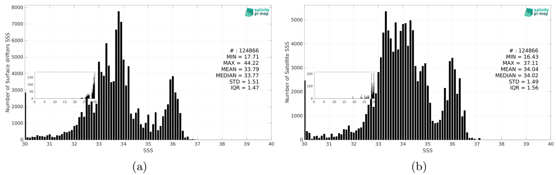
Figure 3: Histograms of SSS from Surface drifters (a) and SMAP SSS L3 v5.0 - Monthly (JPL) (b) considering all match-up pairs per bins of 0.1 over the SMOS coastal zone (<800km) 60N-60S Pi-MEP region and for the full satellite product period.
