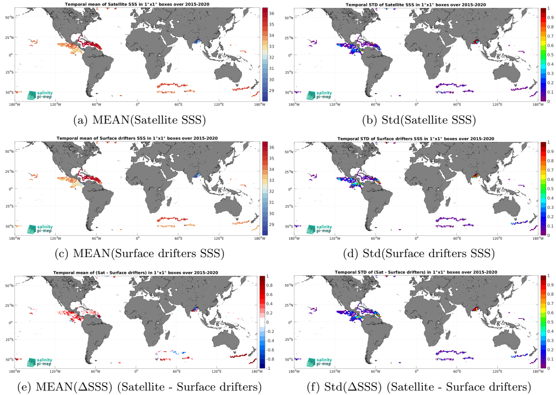
Figure 6: Temporal mean (left) and Std (right) of SSS from SMAP SSS L3 v5.0 - Monthly (JPL) (top), Surface drifters (middle), and of \Delta SSS (Satellite - Surface drifters). Only match-up pairs are used to generate these maps.
