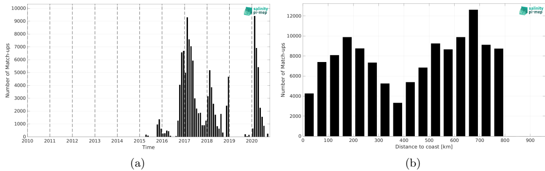
Figure 2: Number of match-ups between Surface drifters and SMAP SSS L3 v5.0 - Monthly (JPL) SSS as a function of time (a) and as function of the distance to coast (b) over the SMOS coastal zone (<800km) 60N-60S Pi-MEP region and for the full satellite product period.
