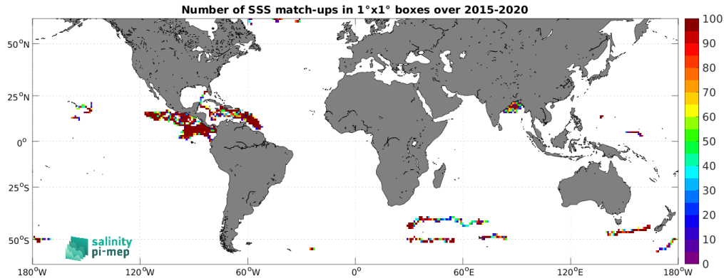
Figure 4: Number of SSS match-ups between Surface drifters SSS and the SMAP SSS L3 v5.0 - Monthly (JPL) SSS product for the SMOS coastal zone (<800km) 60N-60S Pi-MEP region over 1^\circ \times 1^\circ boxes and for the full satellite product period.
