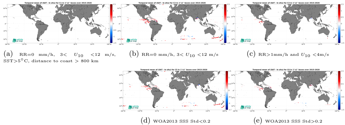
Figure 13: Temporal mean gridded over spatial boxes of size 1^\circ \times 1^\circ of \Delta SSS (SMAP SSS L3 v5.0 - Monthly (JPL) - Surface drifters) for 5 different subdatasets corresponding to:RR=0 mm/h, 3 < U_{10} < 12 m/s, SST >5^\circ C, distance to coast > 800 km (a), RR=0 mm/h, 3 < U_{10} < 12 m/s (b), RR >1 mm/h and U_{10} < 4 m/s (c), WOA2013 SSS Std <0.2 (d), WOA2013 SSS Std >0.2 (e).
