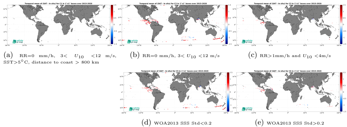
Figure 13: Temporal mean gridded over spatial boxes of size 1^\circ \times 1^\circ of \Delta\text{SSS} (SMAP SSS L3 v5.0 - Monthly (JPL) - Surface drifters) for 5 different subdatasets corresponding to:RR=0 mm/h, 3 < U_{10} < 12 m/s, SST >5^\circ\text{C} , distance to coast > 800 km (a), RR=0 mm/h, 3 < U_{10} < 12 m/s (b), RR >1 mm/h and U_{10} < 4 m/s (c), WOA2013 SSS Std <0.2 (d), WOA2013 SSS Std >0.2 (e).
