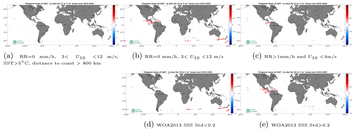
Figure 11: Temporal mean gridded over spatial boxes of size 1^\circ \times 1^\circ of \Delta SSS (SMAP SSS L3 v5.0 - Monthly (JPL) - Surface drifters) for 5 different subdatasets corresponding to:RR=0 mm/h, 3 < U_{10} < 12 m/s, SST >5^\circ\text{C} , distance to coast > 800 km (a), RR=0 mm/h, 3 < U_{10} < 12 m/s (b), RR >1 mm/h and U_{10} < 4 m/s (c), WOA2013 SSS Std <0.2 (d), WOA2013 SSS Std >0.2 (e).
