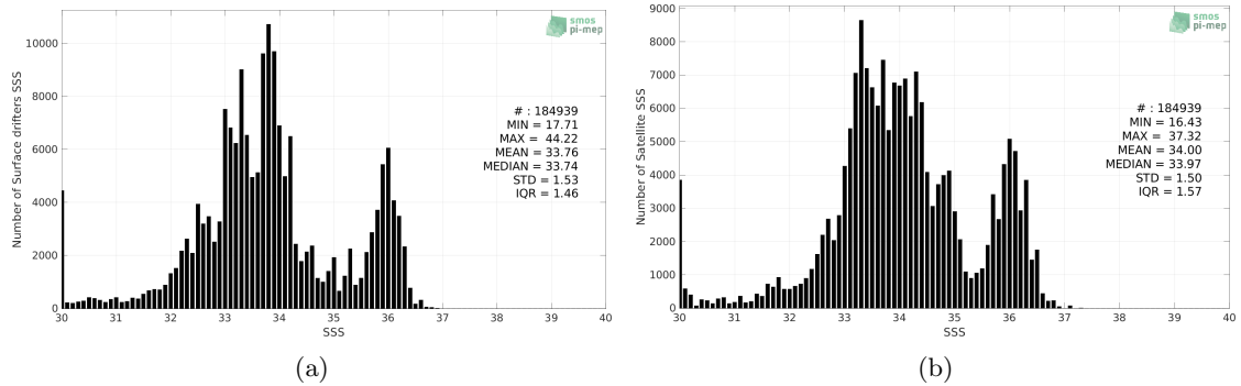
Figure 2: Histograms of SSS from Surface drifters (a) and SMAP SSS L3 v5.0 - Monthly (JPL) (b) considering all match-up pairs per bins of 0.1 over the SMOS coastal zone (<800km) 60N-60S Pi-MEP region and for the full satellite product period.
