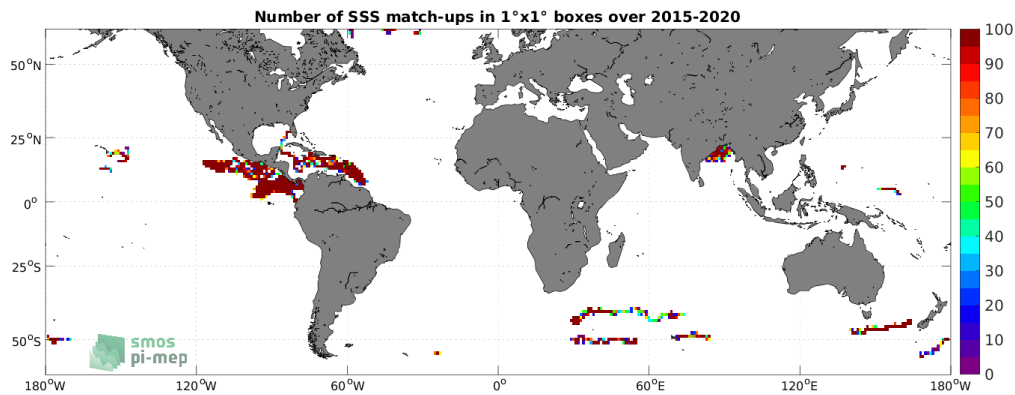
Figure 3: Number of SSS match-ups between Surface drifters SSS and the SMAP SSS L3 v5.0 - Monthly (JPL) SSS product for the SMOS coastal zone (<800km) 60N-60S Pi-MEP region over 1^\circ \times 1^\circ boxes and for the full satellite product period.
