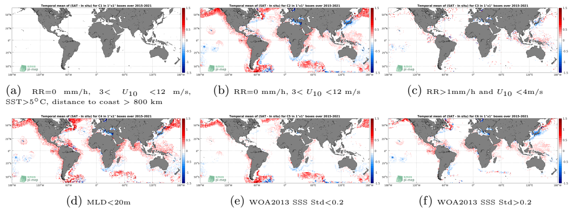
Figure 12: Temporal mean gridded over spatial boxes of size 1^\circ \times 1^\circ of \Delta SSS (SMAP SSS L3 v5.0 - Monthly (JPL) - Argo) for 6 different subdatasets corresponding to: RR=0 mm/h, 3 < U_{10} < 12 m/s, SST > 5°C, distance to coast > 800 km (a), RR=0 mm/h, 3 < U_{10} < 12 m/s (b), RR > 1mm/h and U_{10} < 4 m/s (c), MLD < 20m (d), WOA2013 SSS Std < 0.2 (e), WOA2013 SSS Std > 0.2 (f).
