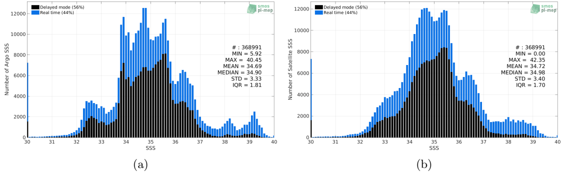
Figure 2: Histograms of SSS from Argo (a) and SMAP SSS L3 v5.0 - Monthly (JPL) (b) considering all match-up pairs per bins of 0.1 over the SMOS coastal zone (<800km) 60N-60S Pi-MEP region and for the full satellite product period.
