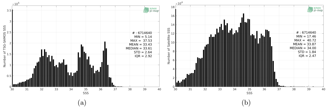
Figure 2: Histograms of SSS from TSG-SAMOS (a) and SMAP-L3-JPL-V4.3-8DAY-RUNNING-60KM (b) considering all match-up pairs per bins of 0.1 over the SMOS coastal zone ( \approx 800\text{km} ) 60N-60S Pi-MEP region and for the full satellite product period.
