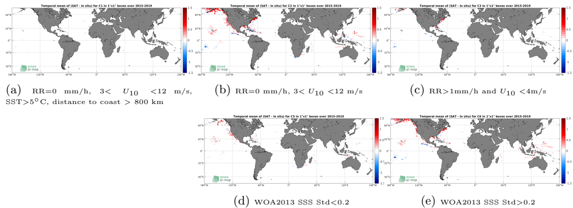
Figure 12: Temporal mean gridded over spatial boxes of size 1^\circ \times 1^\circ of \Delta SSS (SMAP-L3-JPL-V4.3-8DAY-RUNNING-60KM - TSG-SAMOS) for 5 different subdatasets corresponding to: RR=0 mm/h, 3 < U_{10} < 12 m/s, SST > 5^\circ C , distance to coast > 800 km (a), RR=0 mm/h, 3 < U_{10} < 12 m/s (b), RR > 1 mm/h and U_{10} < 4 m/s (c), WOA2013 SSS Std < 0.2 (d), WOA2013 SSS Std > 0.2 (e).
