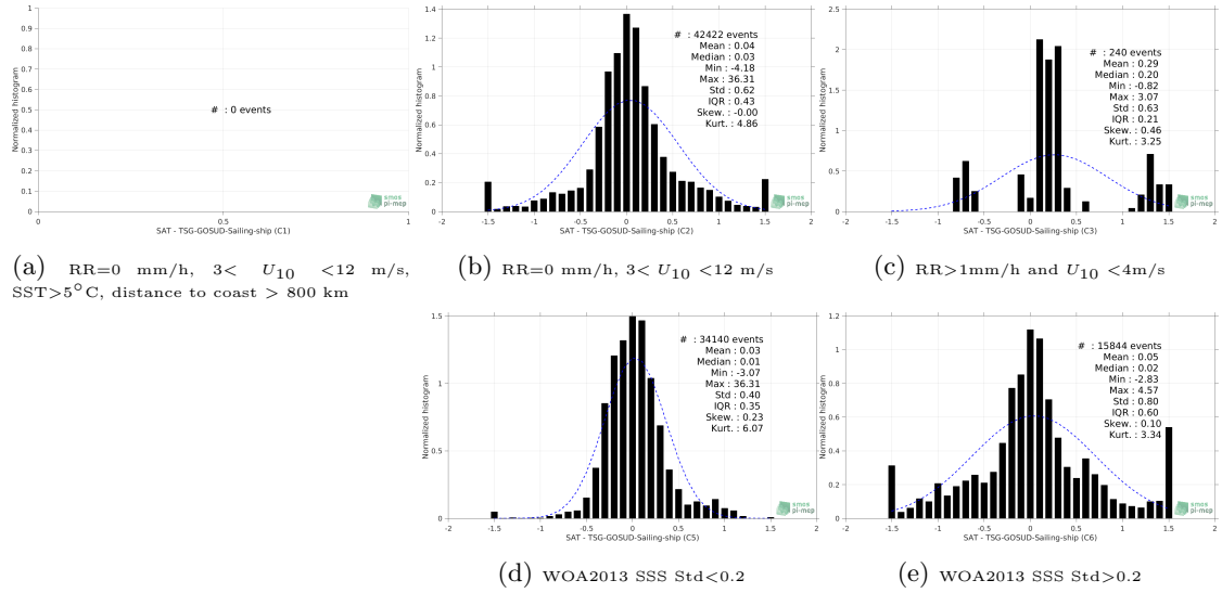
Figure 13: Normalized histogram of \Delta SSS (SMAP-L3-JPL-V4.3-8DAY-RUNNING-60KM - TSG-GOSUD-Sailing-ship) for 5 different subdatasets corresponding to: RR=0 mm/h, 3 < U_{10} < 12 m/s, SST>5°C, distance to coast > 800 km (a), RR=0 mm/h, 3 < U_{10} < 12 m/s (b), RR>1mm/h and U_{10} < 4 m/s (c), WOA2013 SSS Std<0.2 (d), WOA2013 SSS Std>0.2 (e).
