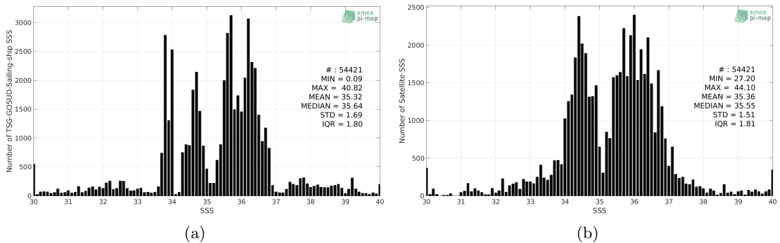
Figure 2: Histograms of SSS from TSG-GOSUD-Sailing-ship (a) and SMAP-L3-JPL-V4.3-8DAY-RUNNING-60KM (b) considering all match-up pairs per bins of 0.1 over the SMOS coastal zone (<800km) 60N-60S Pi-MEP region and for the full satellite product period.
