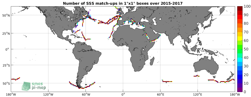
Figure 4: Number of SSS match-ups between TSG-GOSUD-Sailing-ship SSS and the SMAP-L3-JPL-V4.3-8DAY-RUNNING-60KM SSS product for the SMOS coastal zone (<800km) 60N-60S Pi-MEP region over 1°x1° boxes and for the full satellite product period.
