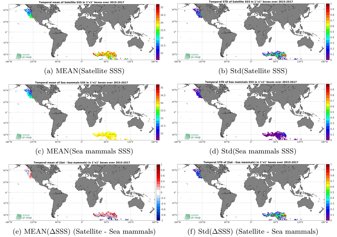
Figure 6: Temporal mean (left) and Std (right) of SSS from SMAP-L3-JPL-V4.3-8DAY-RUNNING-60KM (top), Sea mammals (middle), and of \Delta SSS (Satellite - Sea mammals). Only match-up pairs are used to generate these maps.
