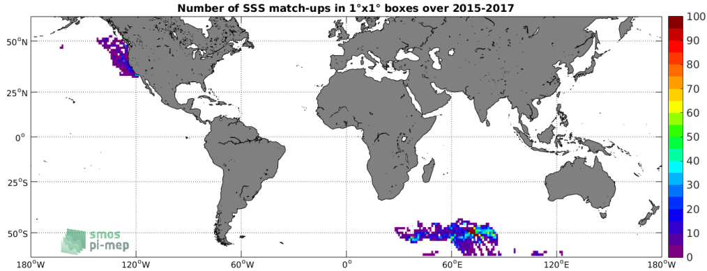
Figure 4: Number of SSS match-ups between Sea mammals SSS and the SMAP-L3-JPL-V4.3-8DAY-RUNNING-60KM SSS product for the SMOS coastal zone (<800km) 60N-60S Pi-MEP region over 1^\circ \times 1^\circ boxes and for the full satellite product period.
