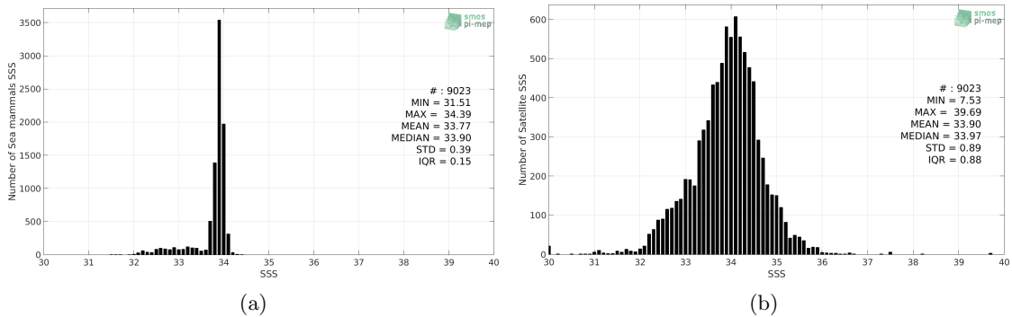
Figure 2: Histograms of SSS from Sea mammals (a) and SMAP-L3-JPL-V4.3-8DAY-RUNNING-60KM (b) considering all match-up pairs per bins of 0.1 over the SMOS coastal zone (<800km) 60N-60S Pi-MEP region and for the full satellite product period.
