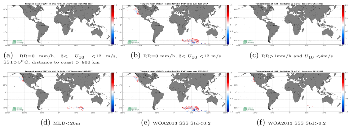
Figure 12: Temporal mean gridded over spatial boxes of size 1^\circ \times 1^\circ of \Delta SSS (SMAP-L3-JPL-V4.3-8DAY-RUNNING-60KM - Sea mammals) for 6 different subdatasets corresponding to: RR=0 mm/h, 3 < U_{10} < 12 m/s, SST > 5^\circ\text{C} , distance to coast > 800 km (a), RR=0 mm/h, 3 < U_{10} < 12 m/s (b), RR > 1 mm/h and U_{10} < 4 m/s (c),MLD < 20 m (d),WOA2013 SSS Std < 0.2 (e),WOA2013 SSS Std > 0.2 (f).
