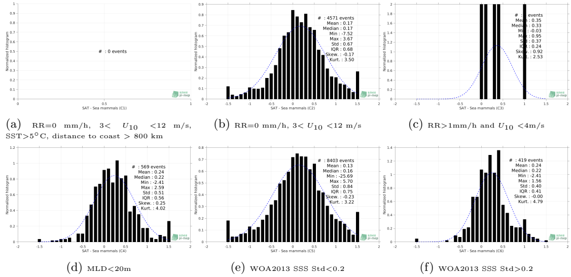
Figure 13: Normalized histogram of \Delta SSS (SMAP-L3-JPL-V4.3-8DAY-RUNNING-60KM - Sea mammals) for 6 different subdatasets corresponding to: RR=0 mm/h, 3 < U_{10} < 12 m/s, SST>5°C, distance to coast > 800 km (a), RR=0 mm/h, 3 < U_{10} < 12 m/s (b), RR>1mm/h and U_{10} < 4 m/s (c), MLD<20m (d), WOA2013 SSS Std<0.2 (e), WOA2013 SSS Std>0.2 (f).
