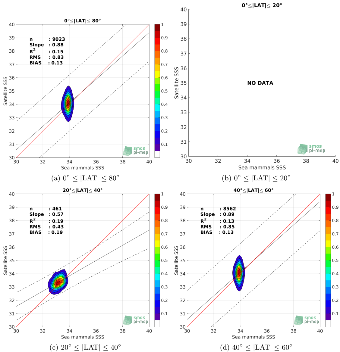
Figure 9: Contour maps of the concentration of SMAP-L3-JPL-V4.3-8DAY-RUNNING-60KM SSS (y-axis) versus Sea mammals SSS (x-axis) at match-up pairs for different latitude bands. For each plot, the red line shows x=y . The black thin and dashed lines indicate a linear fit through the data cloud and the \pm 95\% confidence levels, respectively. The number match-up pairs n , the slope and R^2 coefficient of the linear fit, the root mean square (RMS) and the mean bias between satellite and in situ data are indicated for each latitude band in each plots.
