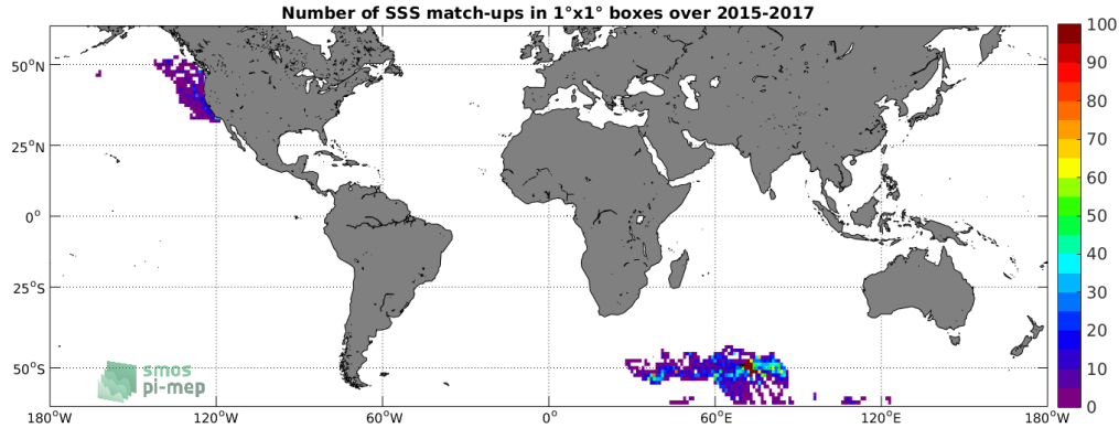
Figure 4: Number of SSS match-ups between Sea mammals SSS and the SMAP-L3-JPL-V4.3-8DAY-RUNNING-60KM SSS product for the SMOS coastal zone ( \approx 800\text{km} ) 60N-60S Pi-MEP region over 1^\circ \times 1^\circ boxes and for the full satellite product period.
