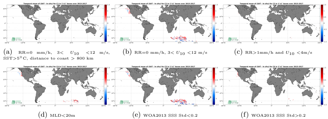
Figure 12: Temporal mean gridded over spatial boxes of size 1^\circ \times 1^\circ of \Delta SSS (SMAP-L3-JPL-V4.3-8DAY-RUNNING-60KM - Sea mammals) for 6 different subdatasets corresponding to:RR=0 mm/h, 3 < U_{10} < 12 m/s, SST > 5^\circ\text{C} , distance to coast > 800 km (a), RR=0 mm/h, 3 < U_{10} < 12 m/s (b), RR > 1 mm/h and U_{10} < 4 m/s (c),MLD < 20 m (d),WOA2013 SSS Std < 0.2 (e),WOA2013 SSS Std > 0.2 (f).
