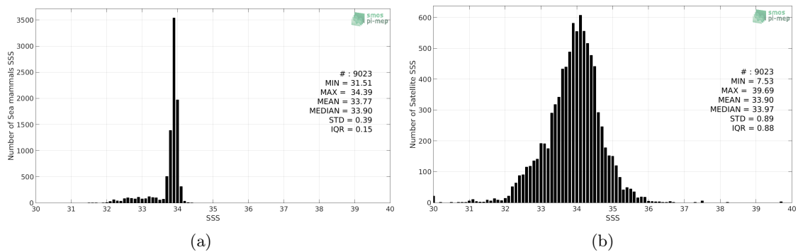
Figure 2: Histograms of SSS from Sea mammals (a) and SMAP-L3-JPL-V4.3-8DAY-RUNNING-60KM (b) considering all match-up pairs per bins of 0.1 over the SMOS coastal zone ( \geq 800\text{km} ) 60N-60S Pi-MEP region and for the full satellite product period.
