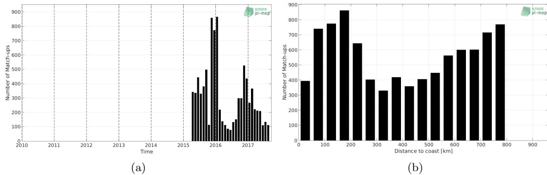
Figure 1: Number of match-ups between Sea mammals and SMAP-L3-JPL-V4.3-8DAY-RUNNING-60KM SSS as a function of time (a) and as function of the distance to coast (b) over the SMOS coastal zone ( \approx 800 km) 60N-60S Pi-MEP region and for the full satellite product period.
