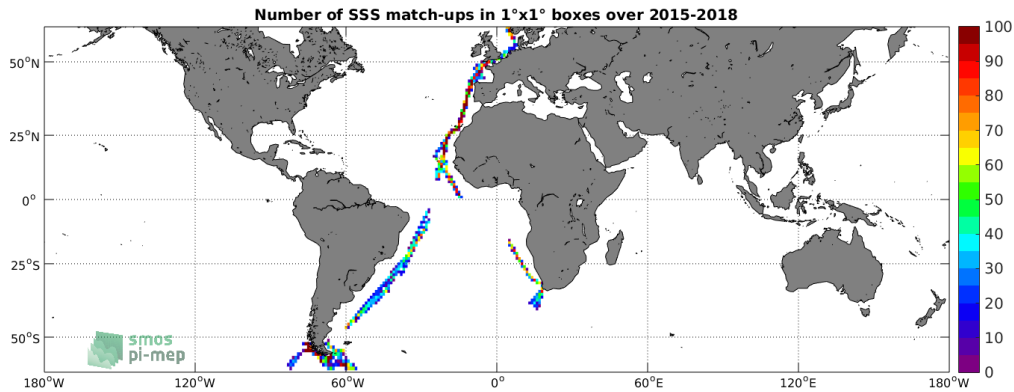
Figure 4: Number of SSS match-ups between TSG-POLARSTERN SSS and the SMAP-L3-JPL-V4.2-MONTHLY-60KM SSS product for the SMOS coastal zone ( \approx 800\text{km} ) 60N-60S Pi-MEP region over 1^\circ \times 1^\circ boxes and for the full satellite product period.
