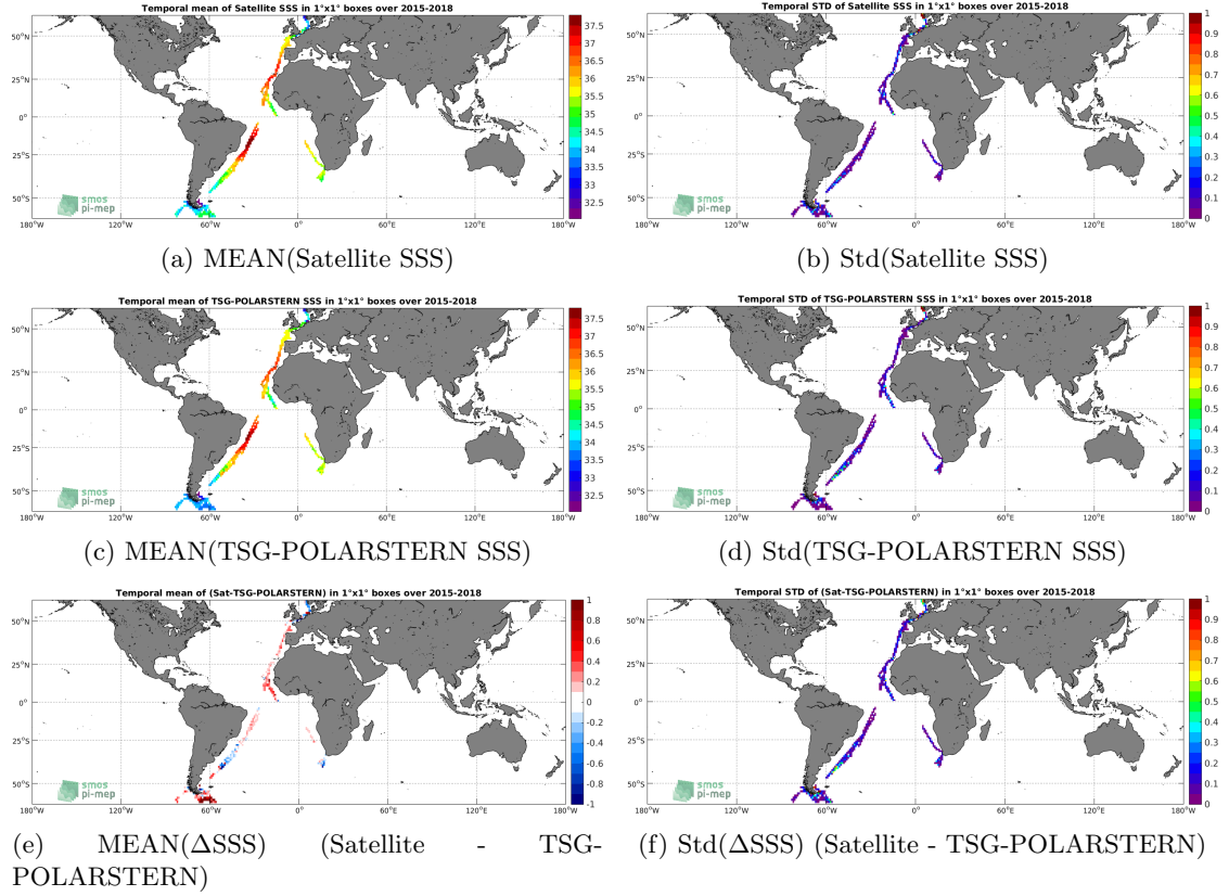
Figure 6: Temporal mean (left) and Std (right) of SSS from SMAP-L3-JPL-V4.2-MONTHLY-60KM (top), TSG-POLARSTERN (middle), and of \Delta SSS (Satellite - TSG-POLARSTERN). Only match-up pairs are used to generate these maps.
