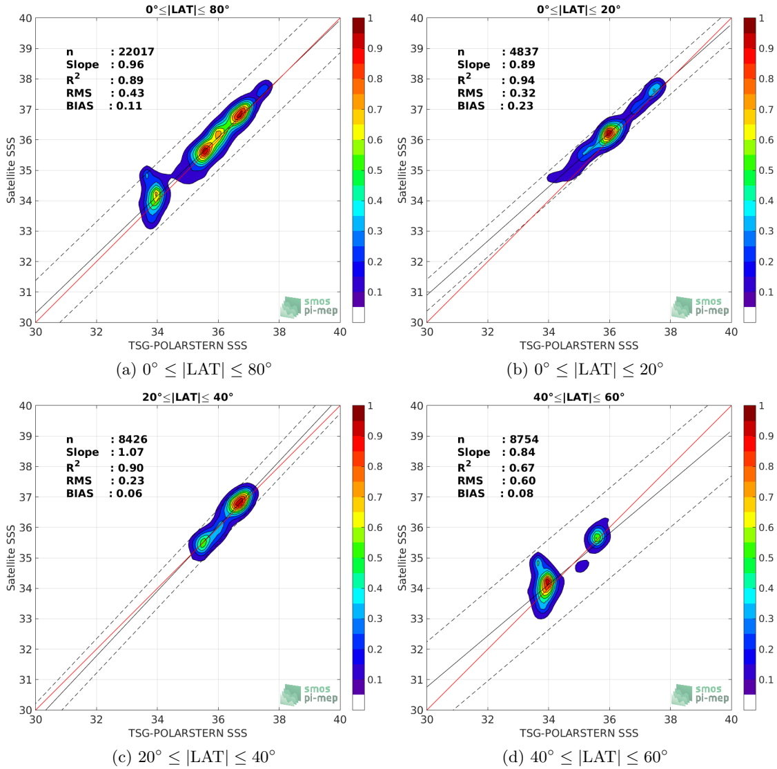
Figure 9: Contour maps of the concentration of SMAP-L3-JPL-V4.2-MONTHLY-60KM SSS (y-axis) versus TSG-POLARSTERN SSS (x-axis) at match-up pairs for different latitude bands. For each plot, the red line shows x=y . The black thin and dashed lines indicate a linear fit through the data cloud and the \pm 95\% confidence levels, respectively. The number match-up pairs n , the slope and R^2 coefficient of the linear fit, the root mean square (RMS) and the mean bias between satellite and in situ data are indicated for each latitude band in each plots.
