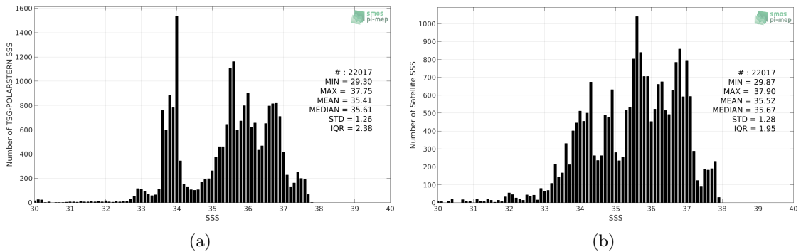
Figure 2: Histograms of SSS from TSG-POLARSTERN (a) and SMAP-L3-JPL-V4.2-MONTHLY-60KM (b) considering all match-up pairs per bins of 0.1 over the SMOS coastal zone ( \geq 800\text{km} ) 60N-60S Pi-MEP region and for the full satellite product period.
