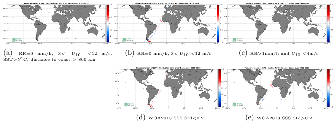
Figure 12: Temporal mean gridded over spatial boxes of size 1^\circ \times 1^\circ of \Delta SSS (SMAP-L3-JPL-V4.2-MONTHLY-60KM - TSG-POLARSTERN) for 5 different subdatasets corresponding to:RR=0 mm/h, 3 < U_{10} < 12 m/s, SST >5^\circ C, distance to coast > 800 km (a), RR=0 mm/h, 3 < U_{10} < 12 m/s (b), RR >1 mm/h and U_{10} < 4 m/s (c), WOA2013 SSS Std <0.2 (d), WOA2013 SSS Std >0.2 (e).
