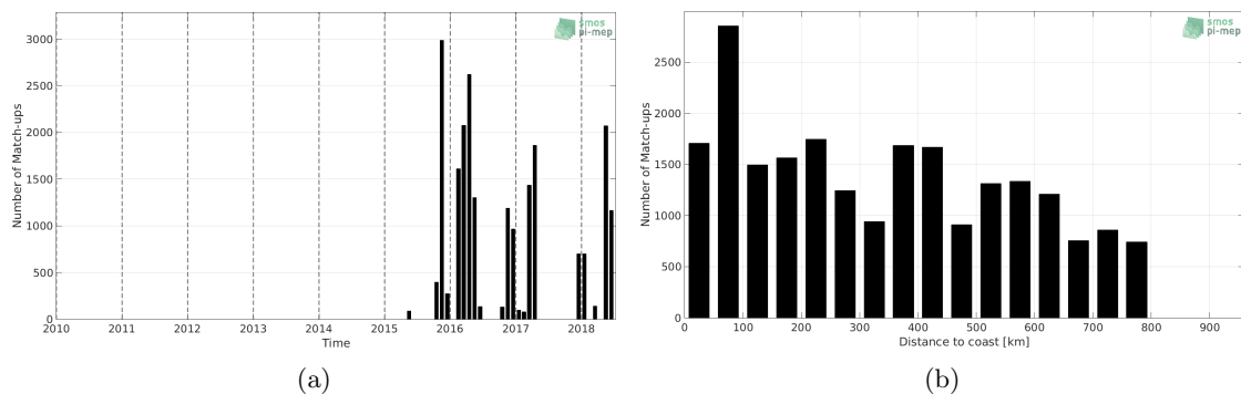
Figure 1: Number of match-ups between TSG-POLARSTERN and SMAP-L3-JPL-V4.2-MONTHLY-60KM SSS as a function of time (a) and as function of the distance to coast (b) over the SMOS coastal zone ( \approx 800 km) 60N-60S Pi-MEP region and for the full satellite product period.
