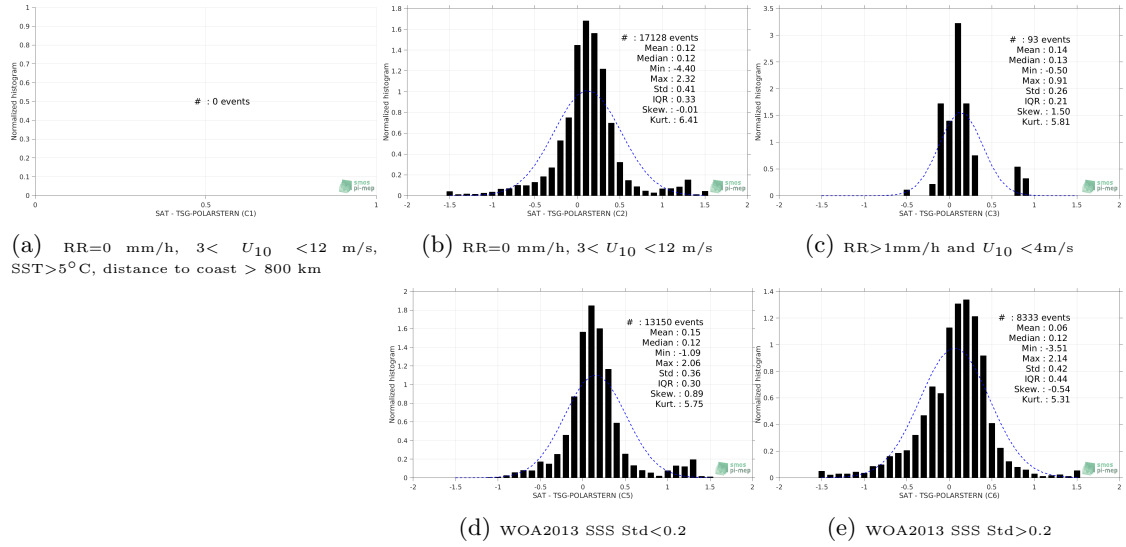
Figure 13: Normalized histogram of \Delta SSS (SMAP-L3-JPL-V4.2-MONTHLY-60KM - TSG-POLARSTERN) for 5 different subdatasets corresponding to: RR=0 mm/h, 3 < U_{10} < 12 m/s, SST > 5°C, distance to coast > 800 km (a), RR=0 mm/h, 3 < U_{10} < 12 m/s (b), RR > 1mm/h and U_{10} < 4 m/s (c), WOA2013 SSS Std < 0.2 (d), WOA2013 SSS Std > 0.2 (e).
