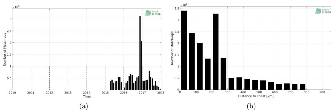
Figure 1: Number of match-ups between TSG-GOSUD-Research-vessel and SMAP-L3-JPL-V4.2-MONTHLY-60KM SSS as a function of time (a) and as function of the distance to coast (b) over the SMOS coastal zone ( \approx 800 km) 60N-60S Pi-MEP region and for the full satellite product period.
