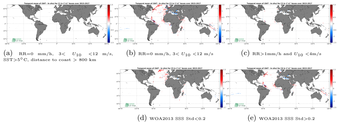
Figure 12: Temporal mean gridded over spatial boxes of size 1^\circ \times 1^\circ of \Delta SSS (SMAP-L3-JPL-V4.2-MONTHLY-60KM - TSG-GOSUD-Research-vessel) for 5 different subdatasets corresponding to:RR=0 mm/h, 3 < U_{10} < 12 m/s, SST >5^\circ C, distance to coast > 800 km (a), RR=0 mm/h, 3 < U_{10} < 12 m/s (b), RR >1 mm/h and U_{10} < 4 m/s (c), WOA2013 SSS Std <0.2 (d), WOA2013 SSS Std >0.2 (e).
