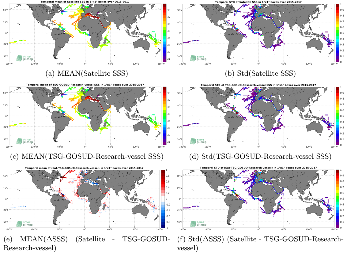
Figure 6: Temporal mean (left) and Std (right) of SSS from SMAP-L3-JPL-V4.2-MONTHLY-60KM (top), TSG-GOSUD-Research-vessel (middle), and of \Delta SSS (Satellite - TSG-GOSUD-Research-vessel). Only match-up pairs are used to generate these maps.
