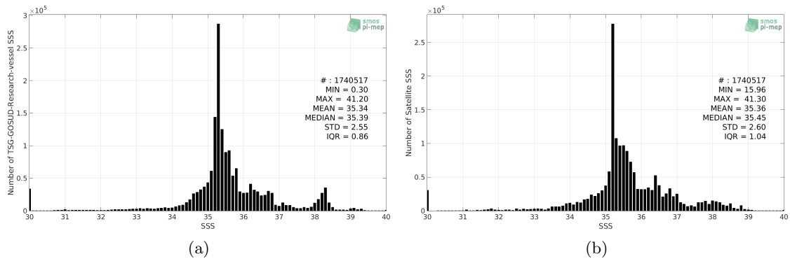
Figure 2: Histograms of SSS from TSG-GOSUD-Research-vessel (a) and SMAP-L3-JPL-V4.2-MONTHLY-60KM (b) considering all match-up pairs per bins of 0.1 over the SMOS coastal zone ( \pm 800 km) 60N-60S Pi-MEP region and for the full satellite product period.
