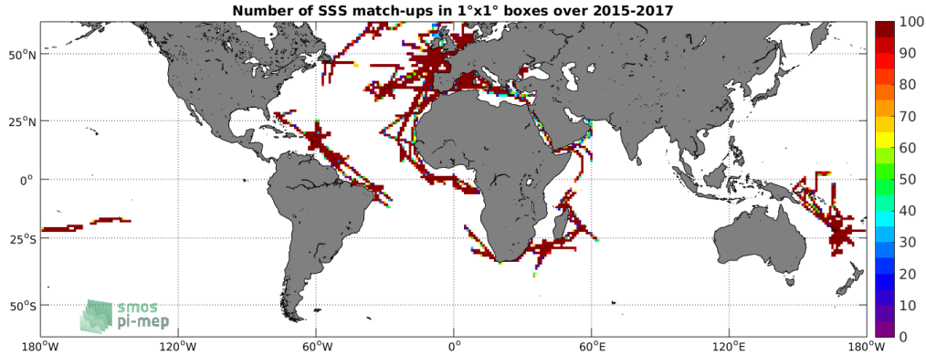
Figure 4: Number of SSS match-ups between TSG-GOSUD-Research-vessel SSS and the SMAP-L3-JPL-V4.2-MONTHLY-60KM SSS product for the SMOS coastal zone ( \pm 800\text{km} ) 60N-60S Pi-MEP region over 1^\circ \times 1^\circ boxes and for the full satellite product period.
