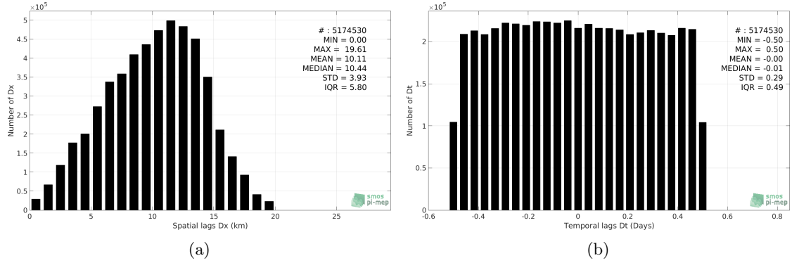
Figure 5: Histograms of the spatial (a) and temporal (b) lags between the time of the TSG-SAMOS measurements and the date of the corresponding SMAP-L3-JPL-V4-8DAY-RUNNING-60KM SSS product.
