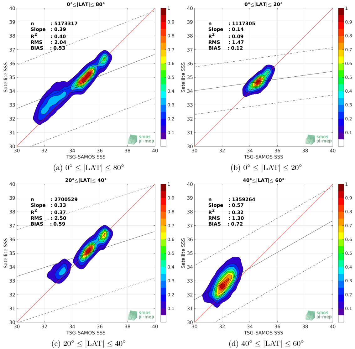
Figure 9: Contour maps of the concentration of SMAP-L3-JPL-V4-8DAY-RUNNING-60KM SSS (y-axis) versus TSG-SAMOS SSS (x-axis) at match-up pairs for different latitude bands. For each plot, the red line shows x=y . The black thin and dashed lines indicate a linear fit through the data cloud and the \pm 95\% confidence levels, respectively. The number match-up pairs n , the slope and R^2 coefficient of the linear fit, the root mean square (RMS) and the mean bias between satellite and in situ data are indicated for each latitude band in each plots.
