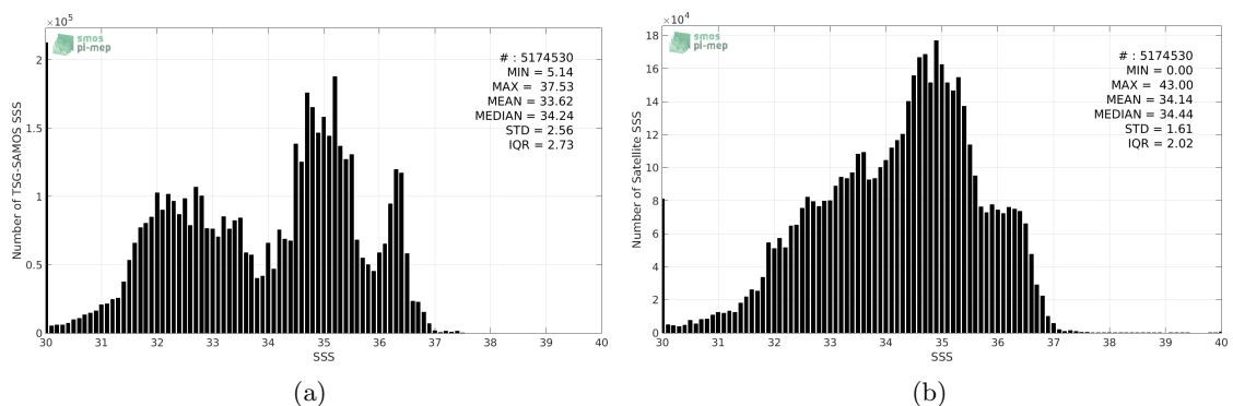
Figure 2: Histograms of SSS from TSG-SAMOS (a) and SMAP-L3-JPL-V4-8DAY-RUNNING-60KM (b) considering all match-up pairs per bins of 0.1 over the SMOS coastal zone ( \approx 800 km) 60N-60S Pi-MEP region and for the full satellite product period.
