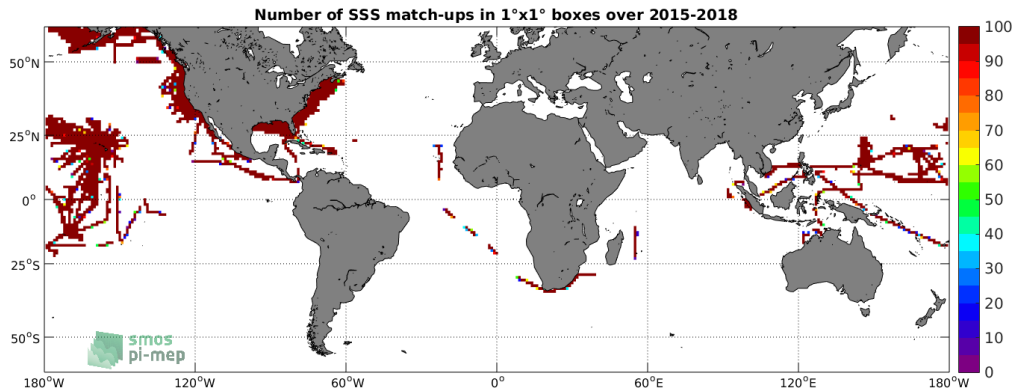
Figure 4: Number of SSS match-ups between TSG-SAMOS SSS and the SMAP-L3-JPL-V4-8DAY-RUNNING-60KM SSS product for the SMOS coastal zone ( \pm 800\text{km} ) 60N-60S Pi-MEP region over 1^\circ \times 1^\circ boxes and for the full satellite product period.
