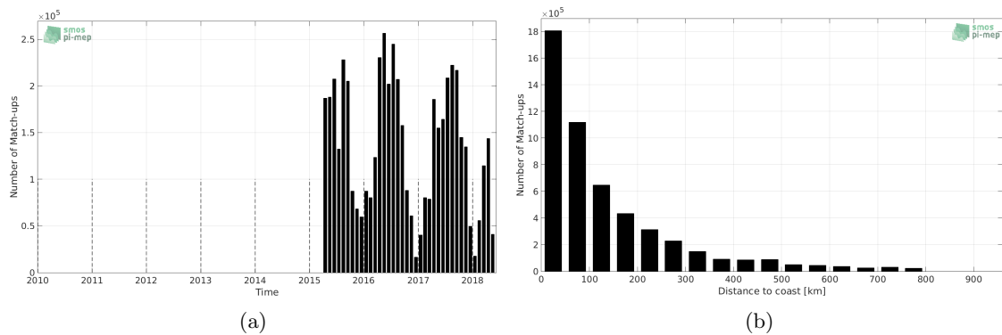
Figure 1: Number of match-ups between TSG-SAMOS and SMAP-L3-JPL-V4-8DAY-RUNNING-60KM SSS as a function of time (a) and as function of the distance to coast (b) over the SMOS coastal zone ( \approx 800 km) 60N-60S Pi-MEP region and for the full satellite product period.
