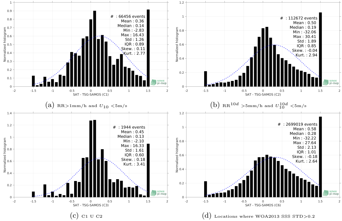
Figure 13: Normalized histogram of \Delta SSS (SMAP-L3-JPL-V4-8DAY-RUNNING-60KM - TSG-SAMOS) for 6 different subdatasets corresponding to: RR > 1\text{mm/h} and U_{10} < 5\text{m/s} (a), RR^{10d} > 5\text{mm/h} and U_{10}^{10d} < 5\text{m/s} (b), C1 U C2 (c), Locations where WOA2013 SSS STD > 0.2 (d).
