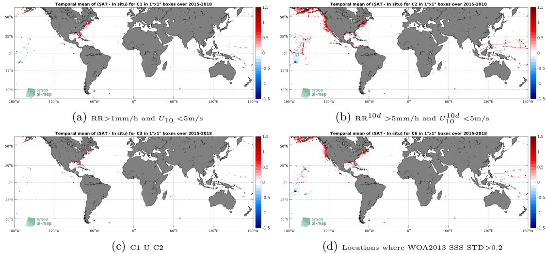
Figure 12: Temporal mean gridded over spatial boxes of size 1^\circ \times 1^\circ of \Delta SSS (SMAP-L3-JPL-V4-8DAY-RUNNING-60KM - TSG-SAMOS) for 4 different subdatasets corresponding to: RR > 1\text{mm/h} and U_{10} < 5\text{m/s} (a), RR^{10d} > 5\text{mm/h} and U_{10}^{10d} < 5\text{m/s} (b), C1 U C2 (c), Locations where WOA2013 SSS STD > 0.2 (d).
