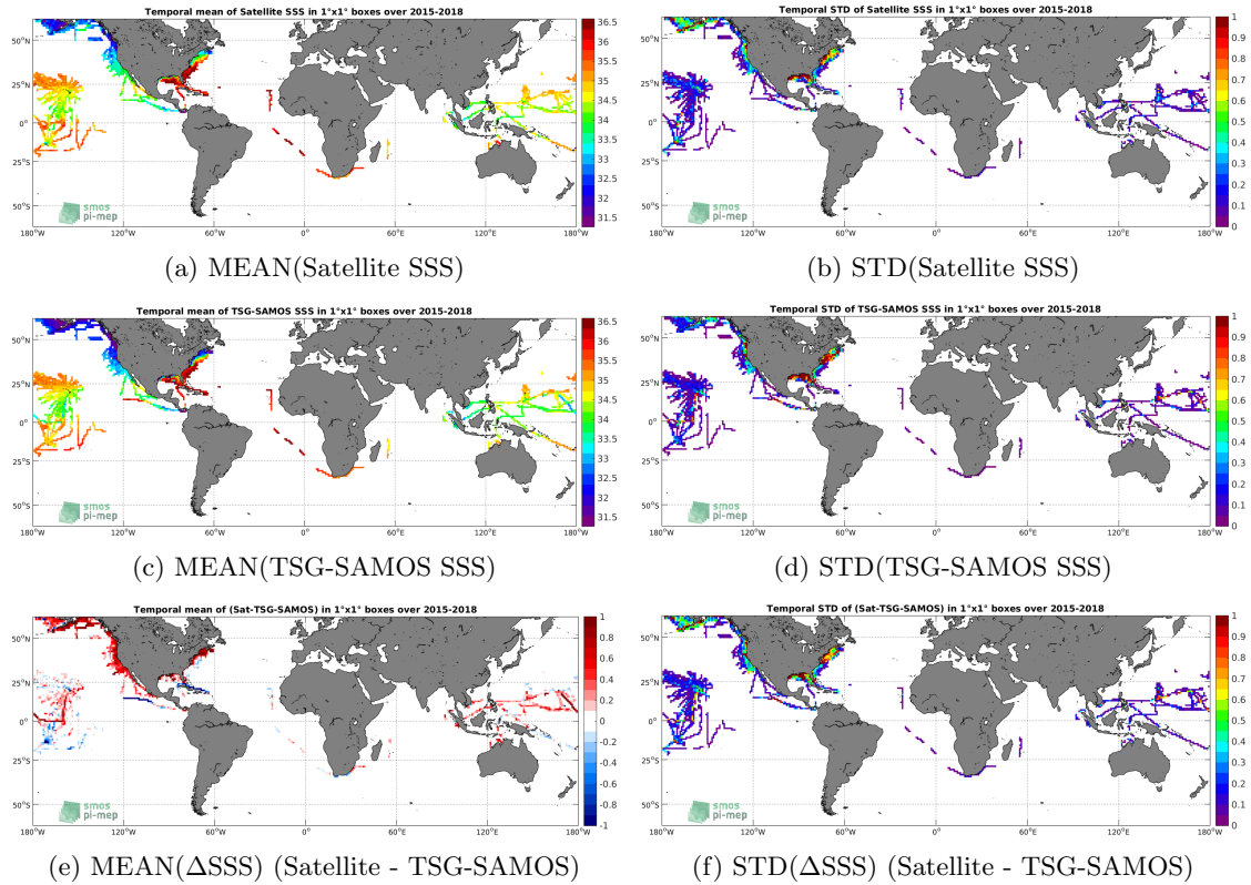
Figure 6: Temporal mean (left) and STD (right) of SSS from SMAP-L3-JPL-V4-8DAY-RUNNING-60KM (top), TSG-SAMOS (middle), and of \Delta SSS (Satellite - TSG-SAMOS). Only match-up pairs are used to generate these maps.
