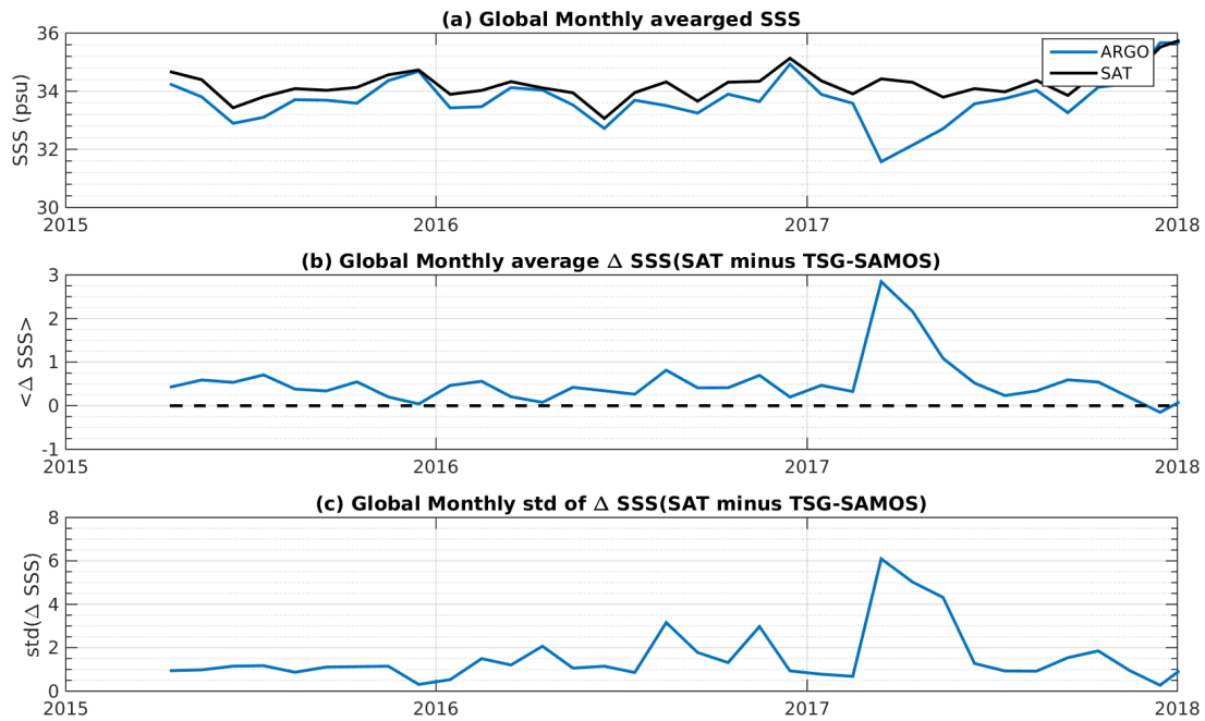
Figure 7: Time series of the monthly averaged mean SSS (top), mean \Delta SSS (Satellite - TSG-SAMOS) and STD of \Delta SSS (Satellite - TSG-SAMOS) over the SMOS coastal zone ( \approx 800 km) 60N-60S Pi-MEP region considering all match-ups collected by the Pi-MEP platform.
