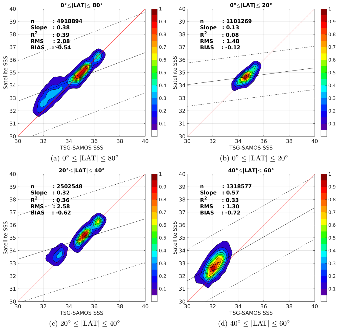
Figure 9: Contour maps of the concentration of SMAP-L3-JPL-V4-8DAY-RUNNING-60KM SSS (y-axis) versus TSG-SAMOS SSS (x-axis) at match-up pairs for different latitude bands. For each plot, the red line shows x=y . The black thin and dashed lines indicate a linear fit through the data cloud and the \pm 95\% confidence levels, respectively. The number match-up pairs n , the slope and R^2 coefficient of the linear fit, the root mean square (RMS) and the mean bias between satellite and in situ data are indicated for each latitude band in each plots.
