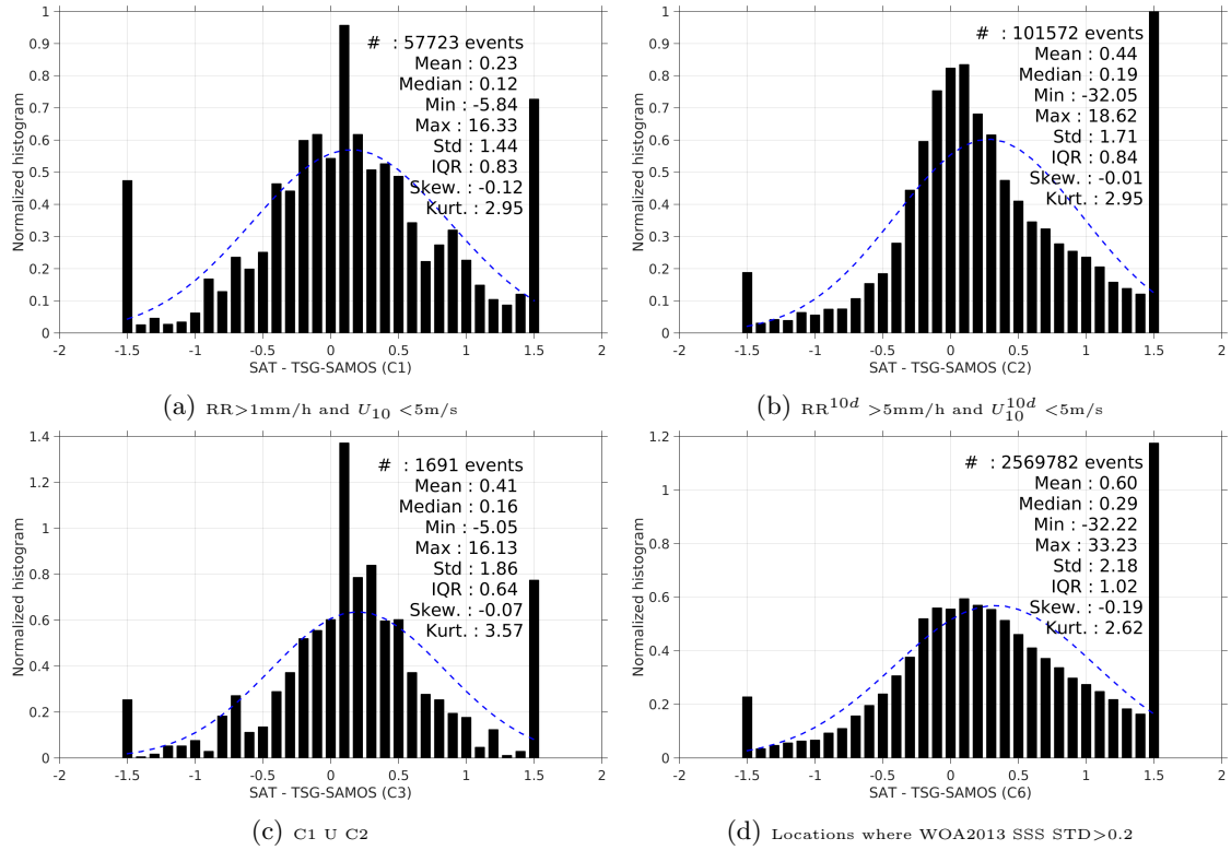
Figure 13: Normalized histogram of \Delta\text{SSS} (SMAP-L3-JPL-V4-8DAY-RUNNING-60KM - TSG-SAMOS) for 6 different subdatasets corresponding to: \text{RR} > 1\text{mm/h} and U_{10} < 5\text{m/s} (a), \text{RR}^{10d} > 5\text{mm/h} and U_{10}^{10d} < 5\text{m/s} (b), C1 U C2 (c), Locations where WOA2013 SSS STD > 0.2 (d).
