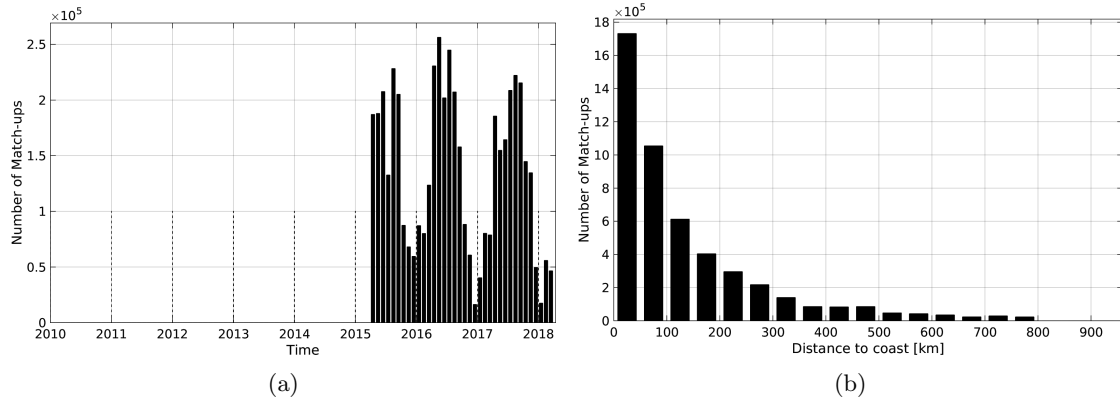
Figure 1: Number of match-ups between TSG-SAMOS and SMAP-L3-JPL-V4-8DAY-RUNNING-60KM SSS as a function of time (a) and as function of the distance to coast (b) over the SMOS coastal zone ( \approx 800 km) 60N-60S Pi-MEP region and for the full satellite product period.
