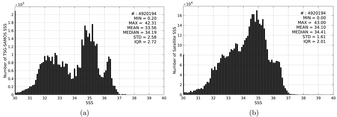
Figure 2: Histograms of SSS from TSG-SAMOS (a) and SMAP-L3-JPL-V4-8DAY-RUNNING-60KM (b) considering all match-up pairs per bins of 0.1 over the SMOS coastal zone ( \approx 800 km) 60N-60S Pi-MEP region and for the full satellite product period.
