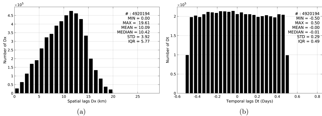
Figure 5: Histograms of the spatial (a) and temporal (b) lags between the time of the TSG-SAMOS measurements and the date of the corresponding SMAP-L3-JPL-V4-8DAY-RUNNING-60KM SSS product.
