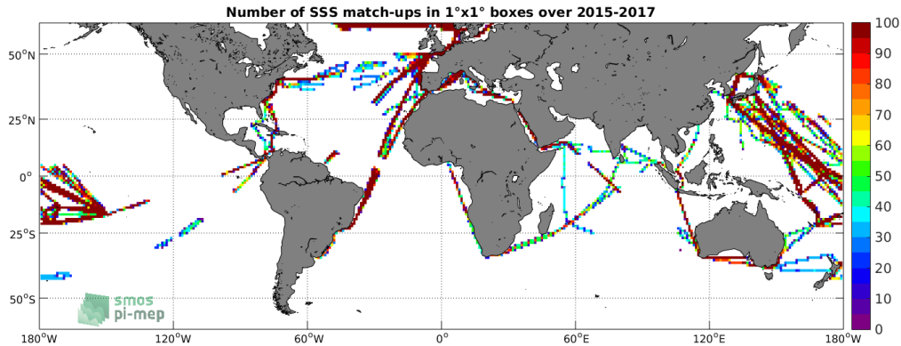
Figure 4: Number of SSS match-ups between TSG-LEGOS-DM SSS and the SMAP-L3-JPL-V4-8DAY-RUNNING-60KM SSS product for the SMOS coastal zone ( \approx 800\text{km} ) 60N-60S Pi-MEP region over 1^\circ \times 1^\circ boxes and for the full satellite product period.
