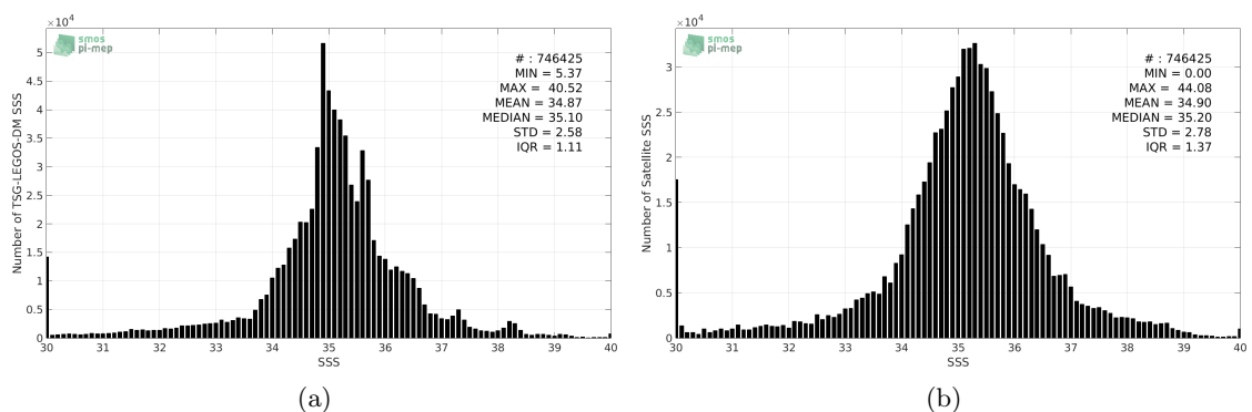
Figure 2: Histograms of SSS from TSG-LEGOS-DM (a) and SMAP-L3-JPL-V4-8DAY-RUNNING-60KM (b) considering all match-up pairs per bins of 0.1 over the SMOS coastal zone ( \approx 800 km) 60N-60S Pi-MEP region and for the full satellite product period.
