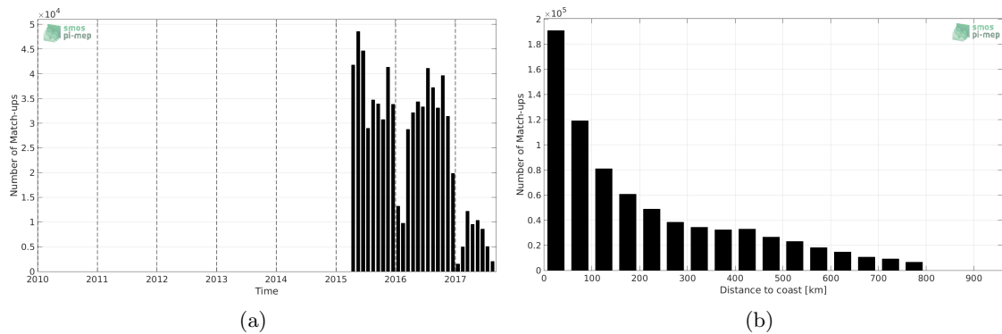
Figure 1: Number of match-ups between TSG-LEGOS-DM and SMAP-L3-JPL-V4-8DAY-RUNNING-60KM SSS as a function of time (a) and as function of the distance to coast (b) over the SMOS coastal zone ( \approx 800 km) 60N-60S Pi-MEP region and for the full satellite product period.
