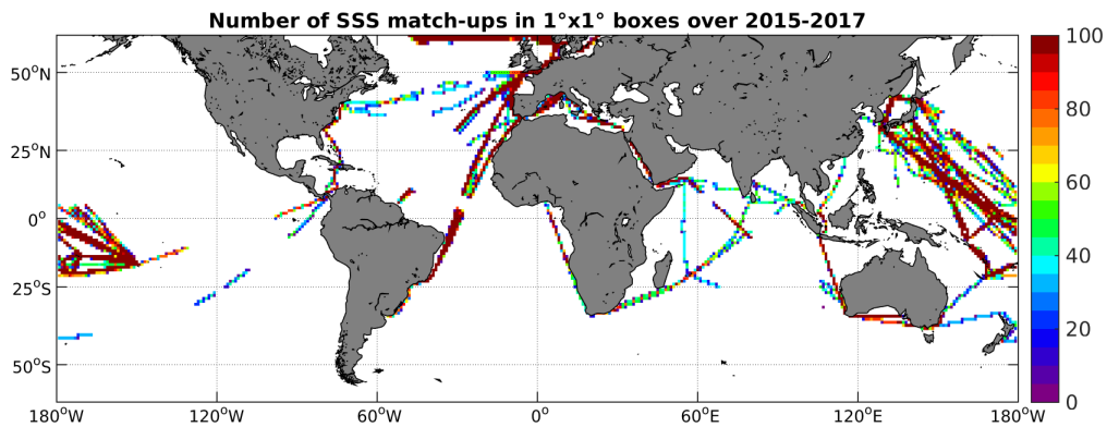
Figure 4: Number of SSS match-ups between TSG-LEGOS-DM SSS and the SMAP-L3-JPL-V4-8DAY-RUNNING-60KM SSS product for the SMOS coastal zone ( \pm 800\text{km} ) 60N-60S Pi-MEP region over 1^\circ \times 1^\circ boxes and for the full satellite product period.
