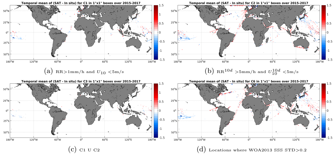
Figure 12: Temporal mean gridded over spatial boxes of size 1^\circ \times 1^\circ of \Delta SSS (SMAP-L3-JPL-V4-8DAY-RUNNING-60KM - TSG-LEGOS-DM) for 4 different subdatasets corresponding to: RR > 1\text{mm/h} and U_{10} < 5\text{m/s} (a), RR^{10d} > 5\text{mm/h} and U_{10}^{10d} < 5\text{m/s} (b), C1 U C2 (c), Locations where WOA2013 SSS STD > 0.2 (d).
