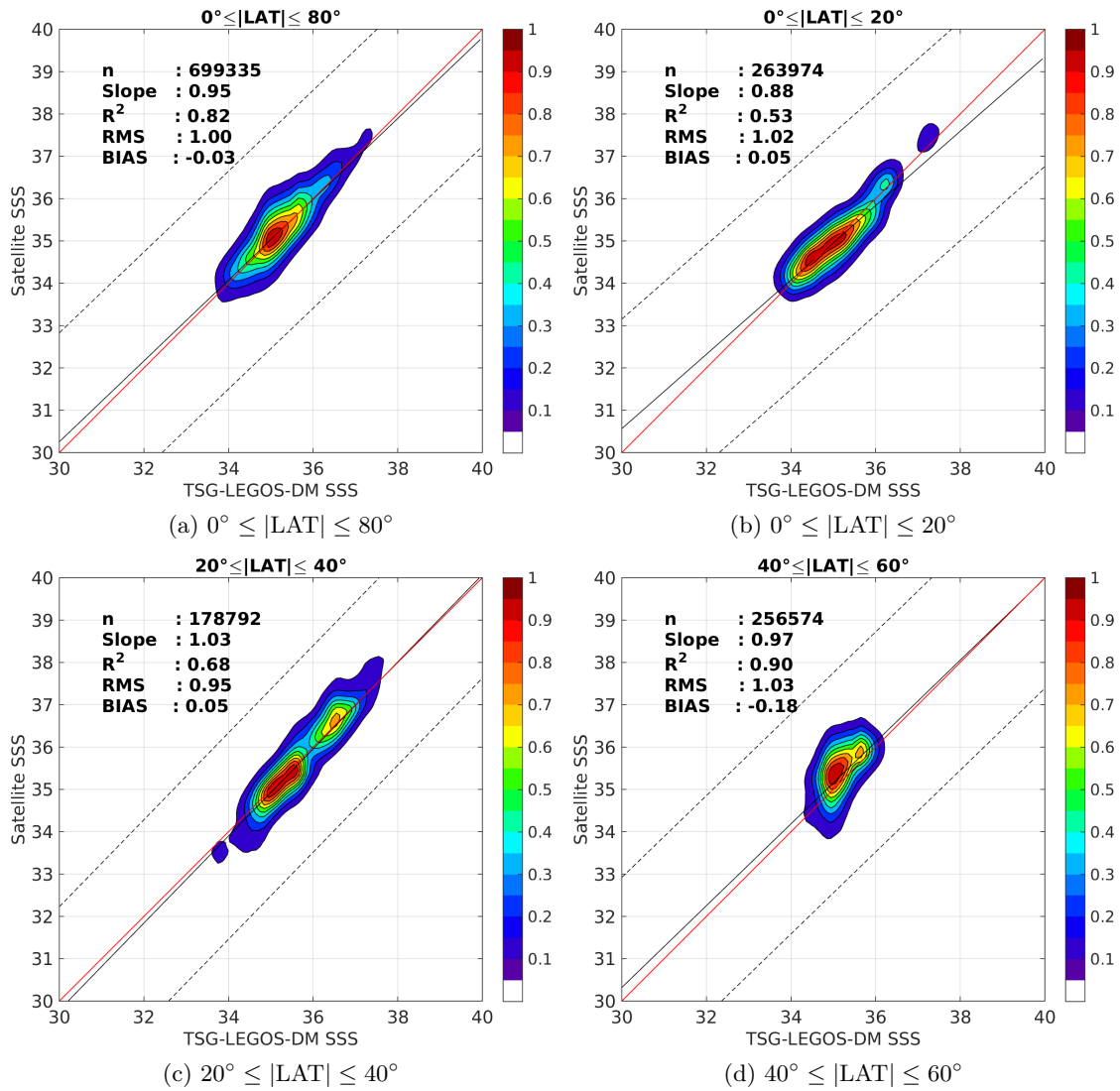
Figure 9: Contour maps of the concentration of SMAP-L3-JPL-V4-8DAY-RUNNING-60KM SSS (y-axis) versus TSG-LEGOS-DM SSS (x-axis) at match-up pairs for different latitude bands. For each plot, the red line shows x=y . The black thin and dashed lines indicate a linear fit through the data cloud and the \pm 95\% confidence levels, respectively. The number match-up pairs n , the slope and R^2 coefficient of the linear fit, the root mean square (RMS) and the mean bias between satellite and in situ data are indicated for each latitude band in each plots.
