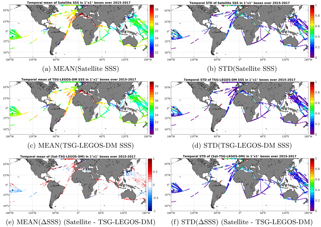
Figure 6: Temporal mean (left) and STD (right) of SSS from SMAP-L3-JPL-V4-8DAY-RUNNING-60KM (top), TSG-LEGOS-DM (middle), and of \Delta SSS (Satellite - TSG-LEGOS-DM). Only match-up pairs are used to generate these maps.
