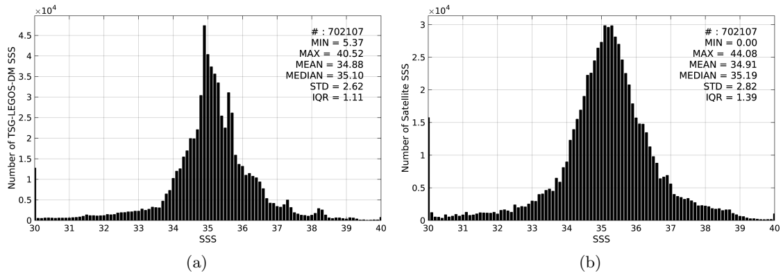
Figure 2: Histograms of SSS from TSG-LEGOS-DM (a) and SMAP-L3-JPL-V4-8DAY-RUNNING-60KM (b) considering all match-up pairs per bins of 0.1 over the SMOS coastal zone ( \approx 800 km) 60N-60S Pi-MEP region and for the full satellite product period.
