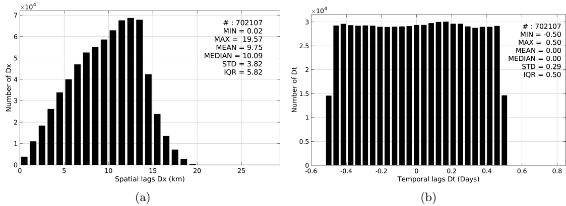
Figure 5: Histograms of the spatial (a) and temporal (b) lags between the time of the TSG-LEGOS-DM measurements and the date of the corresponding SMAP-L3-JPL-V4-8DAY-RUNNING-60KM SSS product.
