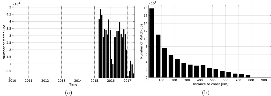
Figure 1: Number of match-ups between TSG-LEGOS-DM and SMAP-L3-JPL-V4-8DAY-RUNNING-60KM SSS as a function of time (a) and as function of the distance to coast (b) over the SMOS coastal zone ( \approx 800 km) 60N-60S Pi-MEP region and for the full satellite product period.
