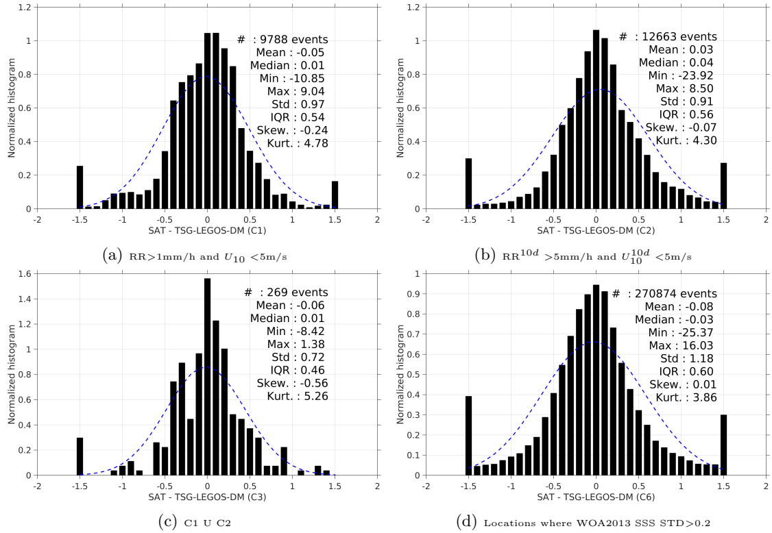
Figure 13: Normalized histogram of \Delta\text{SSS} (SMAP-L3-JPL-V4-8DAY-RUNNING-60KM - TSG-LEGOS-DM) for 6 different subdatasets corresponding to: RR > 1mm/h and U_{10} < 5\text{m/s} (a), \text{RR}^{10d} > 5\text{mm/h} and U_{10}^{10d} < 5\text{m/s} (b), C1 U C2 (c), Locations where WOA2013 SSS STD > 0.2 (d).
