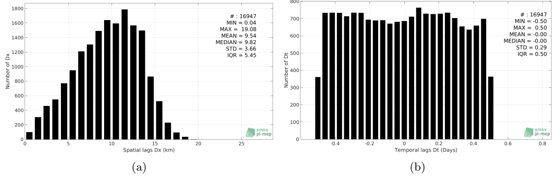
Figure 5: Histograms of the spatial (a) and temporal (b) lags between the time of the TSG-GOSUD-Sailing-ship measurements and the date of the corresponding SMAP-L3-JPL-V4-8DAY-RUNNING-60KM SSS product.
