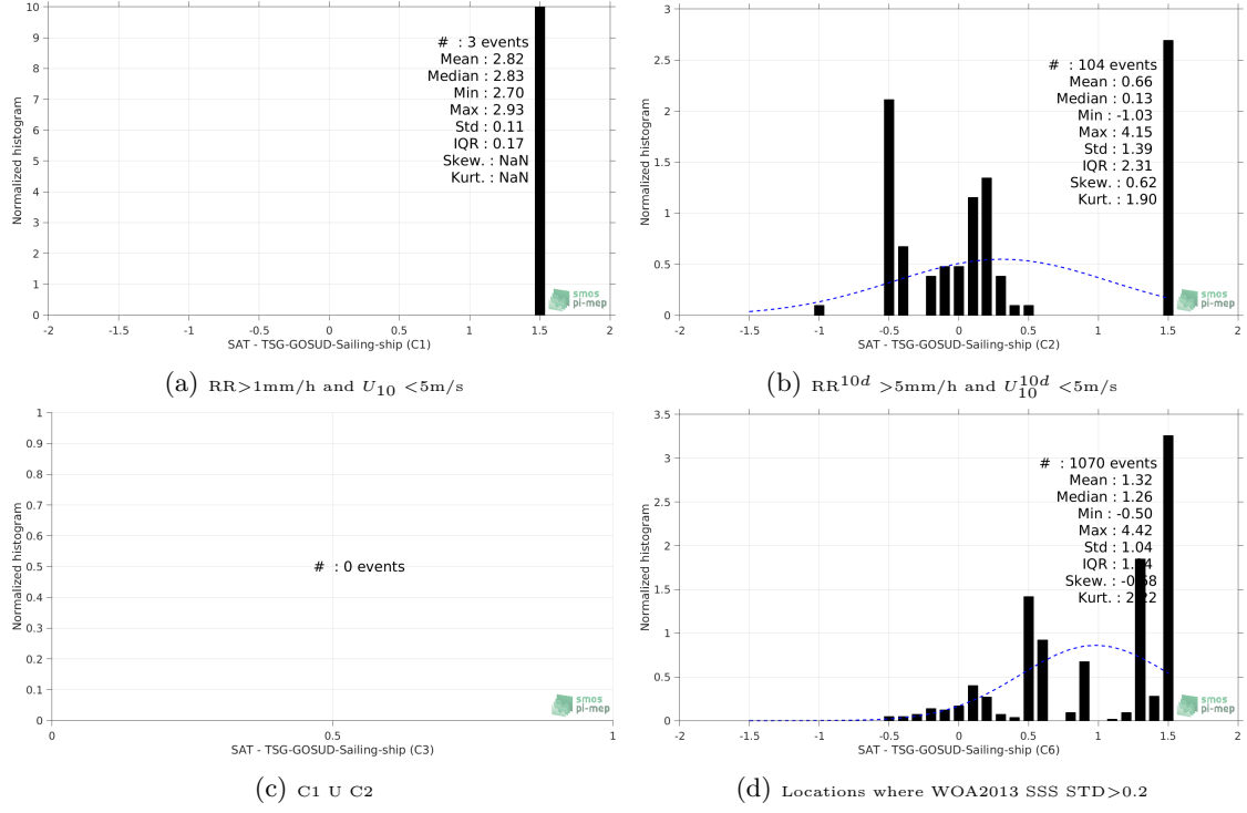
Figure 13: Normalized histogram of \Delta SSS (SMAP-L3-JPL-V4-8DAY-RUNNING-60KM - TSG-GOSUD-Sailing-ship) for 6 different subdatasets corresponding to: RR > 1\text{mm/h} and U_{10} < 5\text{m/s} (a), RR^{10d} > 5\text{mm/h} and U_{10}^{10d} < 5\text{m/s} (b), C1 U C2 (c), Locations where WOA2013 SSS STD > 0.2 (d).
