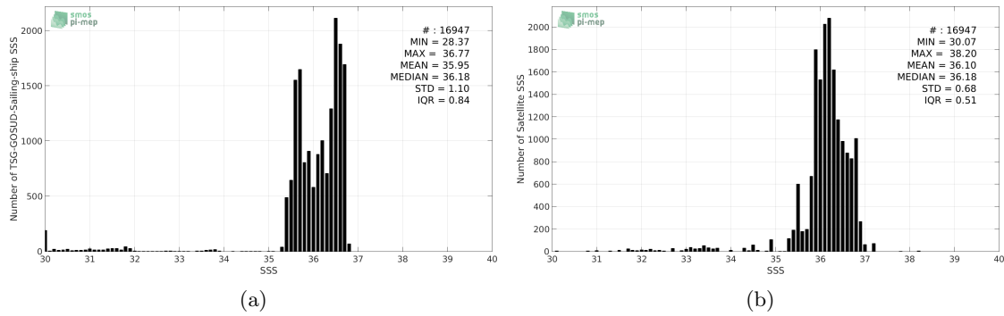
Figure 2: Histograms of SSS from TSG-GOSUD-Sailing-ship (a) and SMAP-L3-JPL-V4-8DAY-RUNNING-60KM (b) considering all match-up pairs per bins of 0.1 over the SMOS coastal zone ( \leq 800 km) 60N-60S Pi-MEP region and for the full satellite product period.
