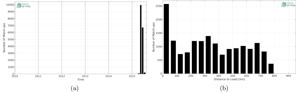
Figure 1: Number of match-ups between TSG-GOSUD-Sailing-ship and SMAP-L3-JPL-V4-8DAY-RUNNING-60KM SSS as a function of time (a) and as function of the distance to coast (b) over the SMOS coastal zone ( \leq 800 km) 60N-60S Pi-MEP region and for the full satellite product period.
