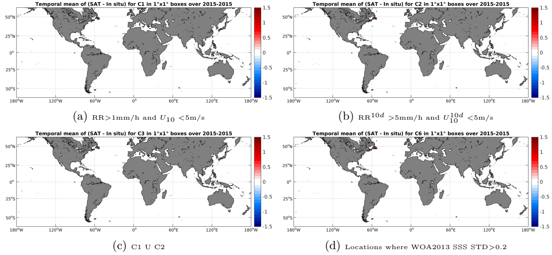
Figure 12: Temporal mean gridded over spatial boxes of size 1^\circ \times 1^\circ of \Delta SSS (SMAP-L3-JPL-V4-8DAY-RUNNING-60KM - TSG-GOSUD-Sailing-ship) for 4 different subdatasets corresponding to: RR > 1mm/h and U_{10} < 5 m/s (a), RR^{10d} > 5 mm/h and U_{10}^{10d} < 5 m/s (b), C1 U C2 (c), Locations where WOA2013 SSS STD > 0.2 (d).
