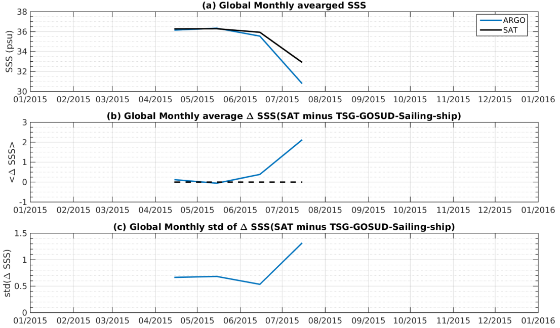
Figure 7: Time series of the monthly averaged mean SSS (top), mean \Delta SSS (Satellite - TSG-GOSUD-Sailing-ship) and STD of \Delta SSS (Satellite - TSG-GOSUD-Sailing-ship) over the SMOS coastal zone ( \approx 800\text{km} ) 60N-60S Pi-MEP region considering all match-ups collected by the Pi-MEP platform.
