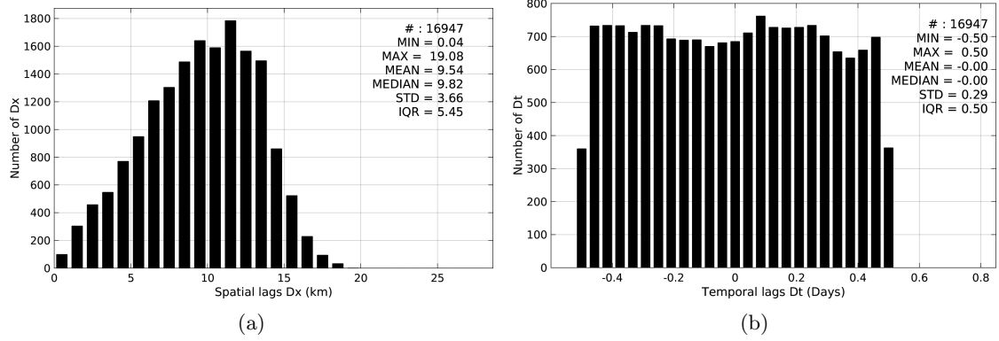
Figure 5: Histograms of the spatial (a) and temporal (b) lags between the time of the TSG-GOSUD-Sailing-ship measurements and the date of the corresponding SMAP-L3-JPL-V4-8DAY-RUNNING-60KM SSS product.
