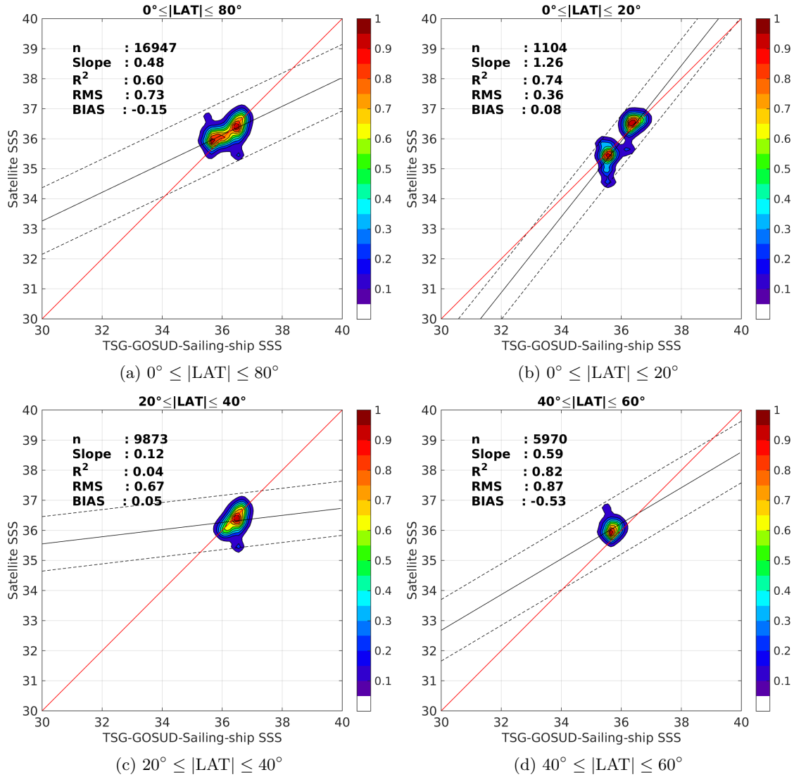
Figure 9: Contour maps of the concentration of SMAP-L3-JPL-V4-8DAY-RUNNING-60KM SSS (y-axis) versus TSG-GOSUD-Sailing-ship SSS (x-axis) at match-up pairs for different latitude bands. For each plot, the red line shows x=y . The black thin and dashed lines indicate a linear fit through the data cloud and the \pm 95\% confidence levels, respectively. The number match-up pairs n , the slope and R^2 coefficient of the linear fit, the root mean square (RMS) and the mean bias between satellite and in situ data are indicated for each latitude band in each plots.
