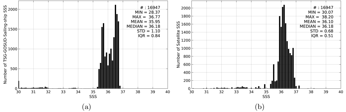
Figure 2: Histograms of SSS from TSG-GOSUD-Sailing-ship (a) and SMAP-L3-JPL-V4-8DAY-RUNNING-60KM (b) considering all match-up pairs per bins of 0.1 over the SMOS coastal zone ( \geq 800 km) 60N-60S Pi-MEP region and for the full satellite product period.
