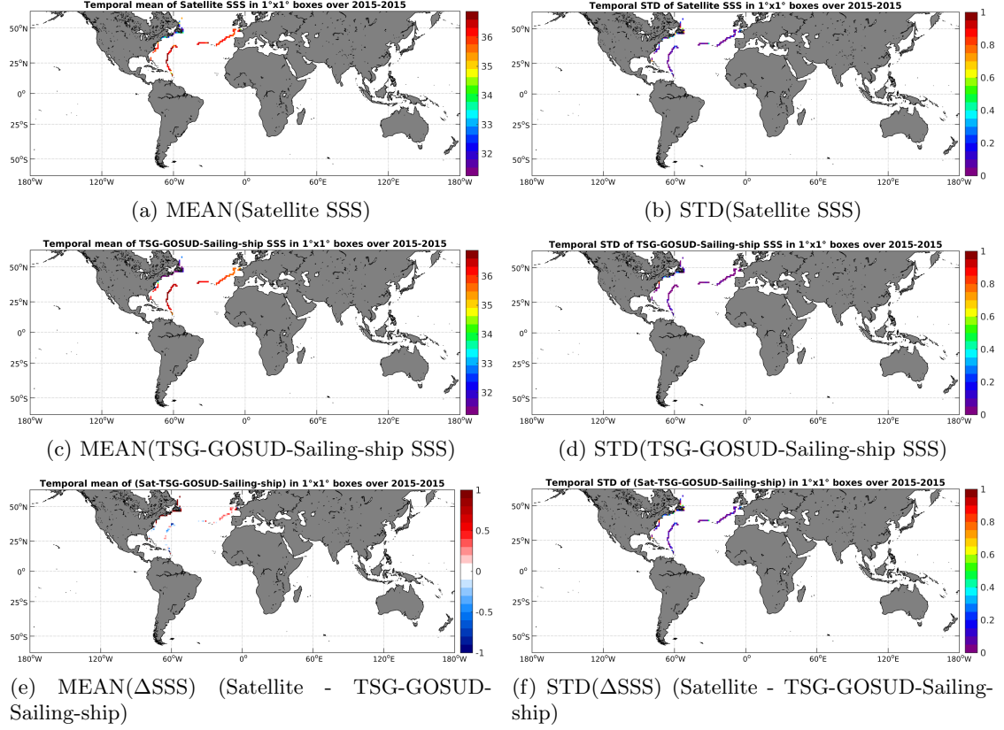
Figure 6: Temporal mean (left) and STD (right) of SSS from SMAP-L3-JPL-V4-8DAY-RUNNING-60KM (top), TSG-GOSUD-Sailing-ship (middle), and of \Delta SSS (Satellite - TSG-GOSUD-Sailing-ship). Only match-up pairs are used to generate these maps.
