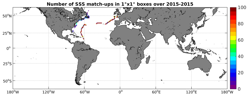
Figure 4: Number of SSS match-ups between TSG-GOSUD-Sailing-ship SSS and the SMAP-L3-JPL-V4-8DAY-RUNNING-60KM SSS product for the SMOS coastal zone ( \pm 800\text{km} ) 60N-60S Pi-MEP region over 1^\circ \times 1^\circ boxes and for the full satellite product period.
