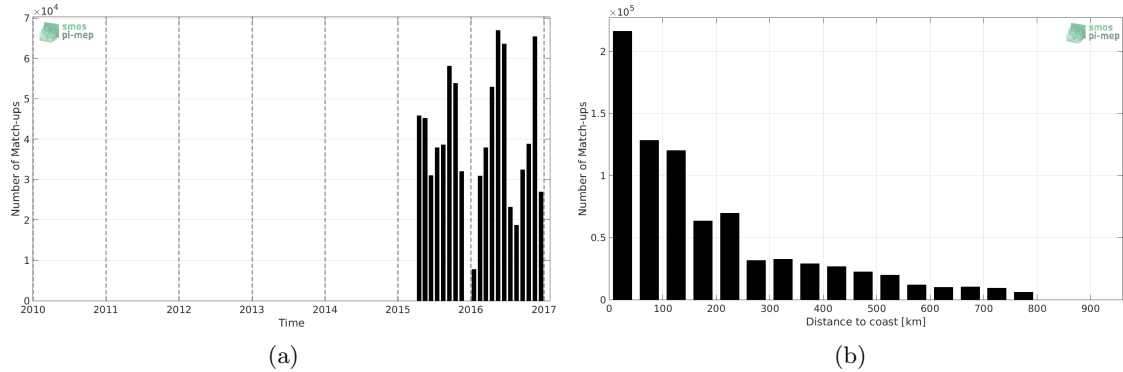
Figure 1: Number of match-ups between TSG-GOSUD-Research-vessel and SMAP-L3-JPL-V4-8DAY-RUNNING-60KM SSS as a function of time (a) and as function of the distance to coast (b) over the SMOS coastal zone ( \pm 800 km) 60N-60S Pi-MEP region and for the full satellite product period.
