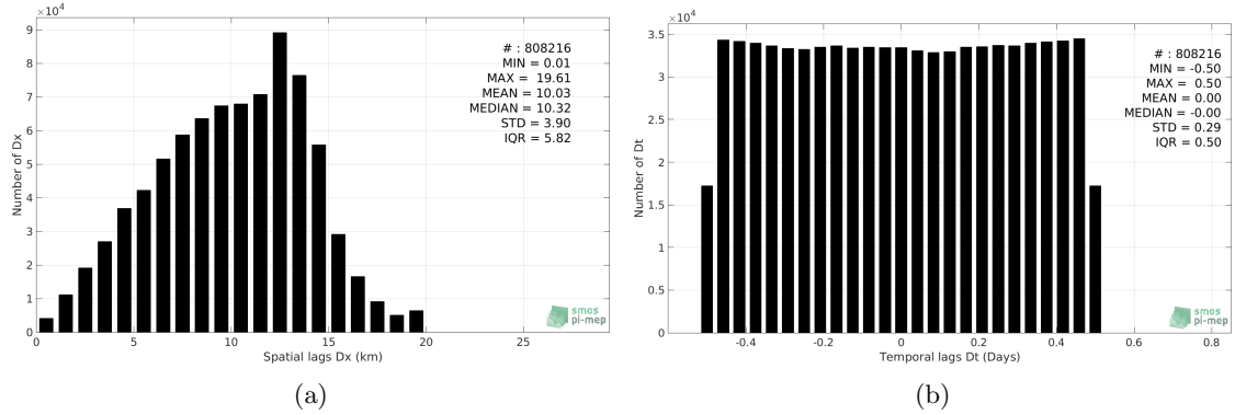
Figure 5: Histograms of the spatial (a) and temporal (b) lags between the time of the TSG-GOSUD-Research-vessel measurements and the date of the corresponding SMAP-L3-JPL-V4-8DAY-RUNNING-60KM SSS product.
