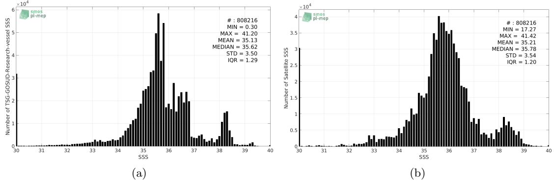
Figure 2: Histograms of SSS from TSG-GOSUD-Research-vessel (a) and SMAP-L3-JPL-V4-8DAY-RUNNING-60KM (b) considering all match-up pairs per bins of 0.1 over the SMOS coastal zone ( \pm 800\text{km} ) 60N-60S Pi-MEP region and for the full satellite product period.
