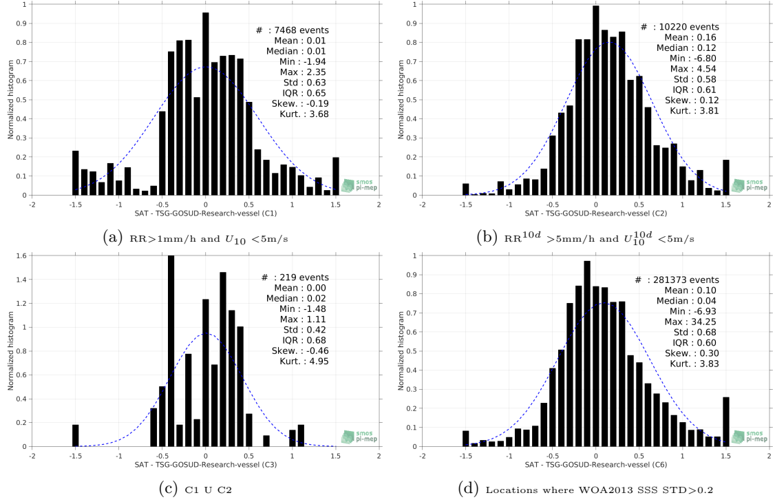
Figure 13: Normalized histogram of \Delta SSS (SMAP-L3-JPL-V4-8DAY-RUNNING-60KM - TSG-GOSUD-Research-vessel) for 6 different subdatasets corresponding to: RR > 1\text{mm/h} and U_{10} < 5\text{m/s} (a), RR^{10d} > 5\text{mm/h} and U_{10}^{10d} < 5\text{m/s} (b), C1 U C2 (c), Locations where WOA2013 SSS STD > 0.2 (d).
