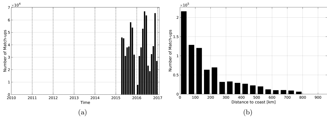
Figure 1: Number of match-ups between TSG-GOSUD-Research-vessel and SMAP-L3-JPL-V4-8DAY-RUNNING-60KM SSS as a function of time (a) and as function of the distance to coast (b) over the SMOS coastal zone ( \pm 800 km) 60N-60S Pi-MEP region and for the full satellite product period.
