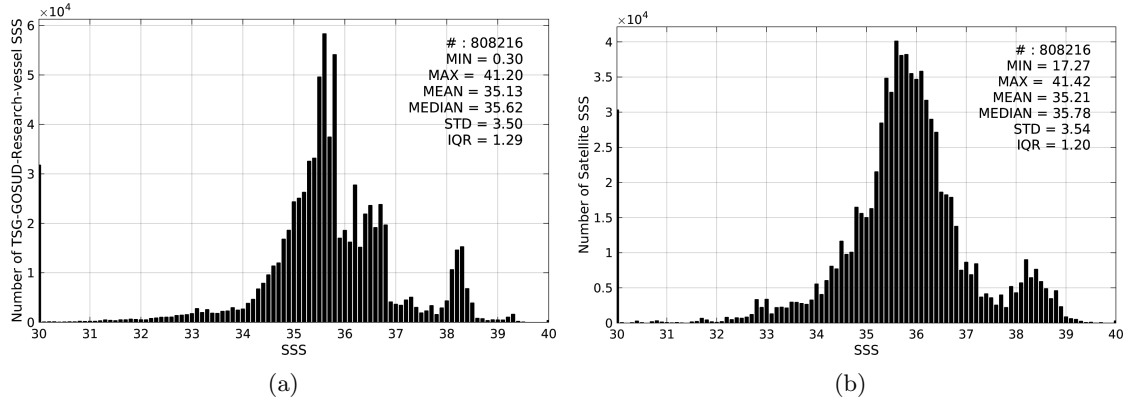
Figure 2: Histograms of SSS from TSG-GOSUD-Research-vessel (a) and SMAP-L3-JPL-V4-8DAY-RUNNING-60KM (b) considering all match-up pairs per bins of 0.1 over the SMOS coastal zone ( \pm 800\text{km} ) 60N-60S Pi-MEP region and for the full satellite product period.
