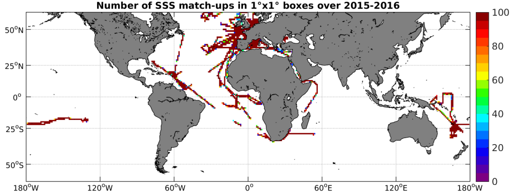
Figure 4: Number of SSS match-ups between TSG-GOSUD-Research-vessel SSS and the SMAP-L3-JPL-V4-8DAY-RUNNING-60KM SSS product for the SMOS coastal zone ( \pm 800\text{km} ) 60N-60S Pi-MEP region over 1^\circ \times 1^\circ boxes and for the full satellite product period.
