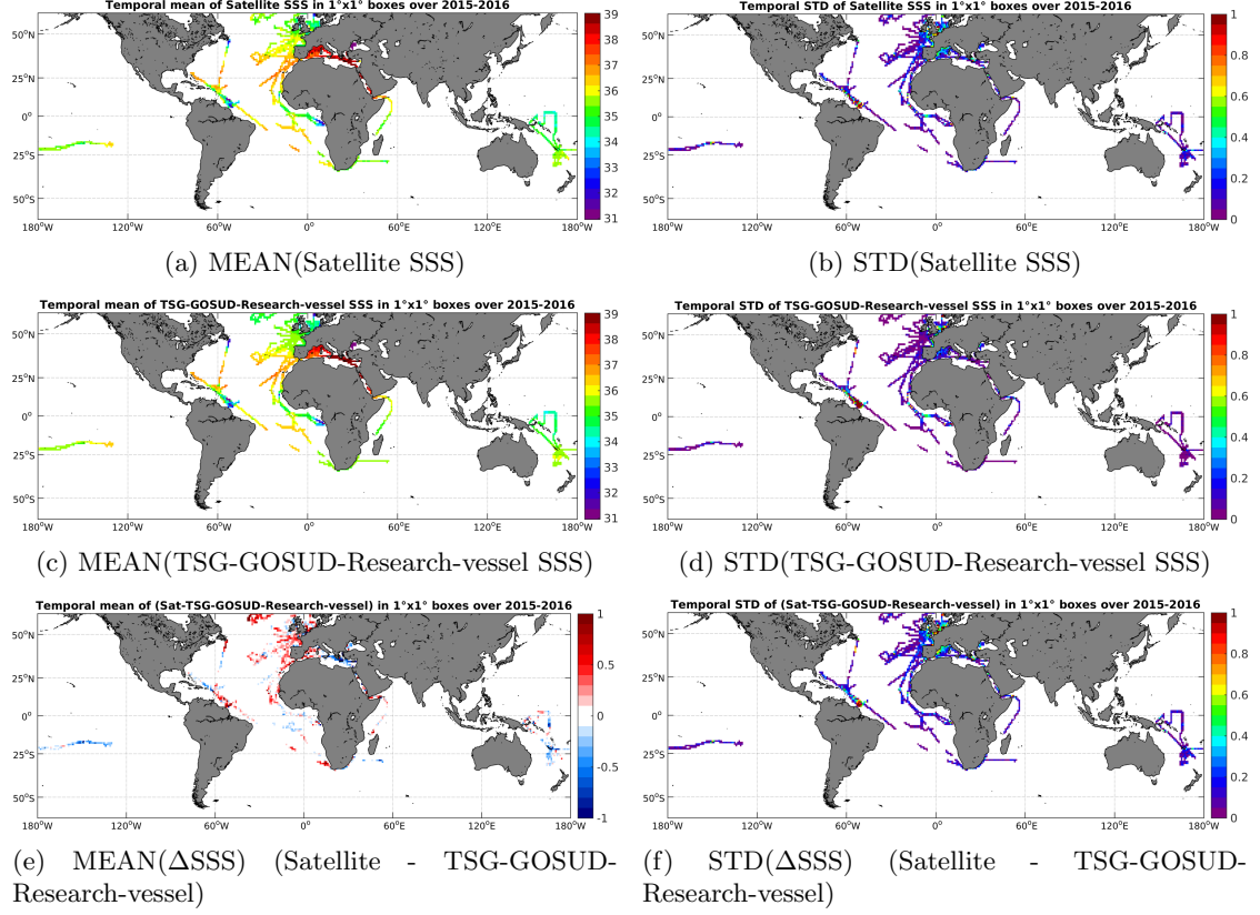
Figure 6: Temporal mean (left) and STD (right) of SSS from SMAP-L3-JPL-V4-8DAY-RUNNING-60KM (top), TSG-GOSUD-Research-vessel (middle), and of \Delta SSS (Satellite - TSG-GOSUD-Research-vessel). Only match-up pairs are used to generate these maps.
