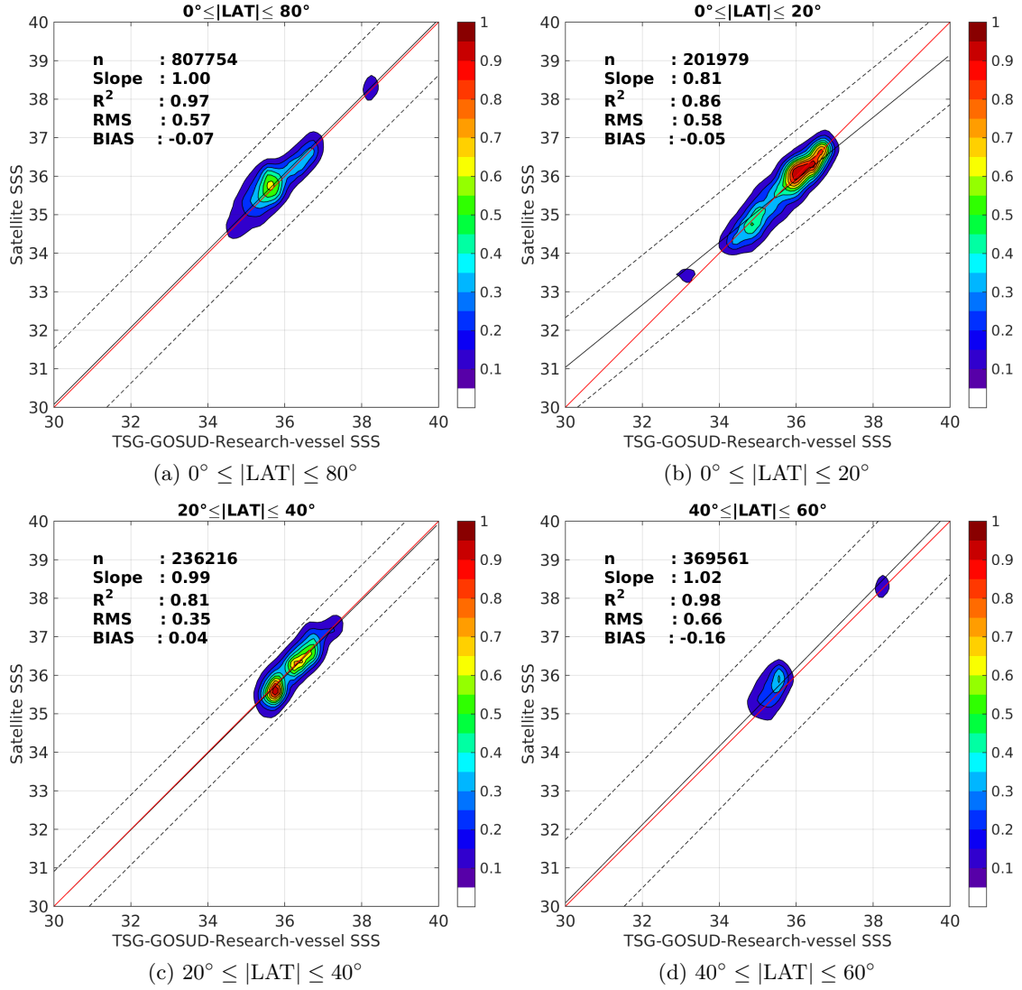
Figure 9: Contour maps of the concentration of SMAP-L3-JPL-V4-8DAY-RUNNING-60KM SSS (y-axis) versus TSG-GOSUD-Research-vessel SSS (x-axis) at match-up pairs for different latitude bands. For each plot, the red line shows x=y . The black thin and dashed lines indicate a linear fit through the data cloud and the \pm 95\% confidence levels, respectively. The number match-up pairs n , the slope and R^2 coefficient of the linear fit, the root mean square (RMS) and the mean bias between satellite and in situ data are indicated for each latitude band in each plots.
