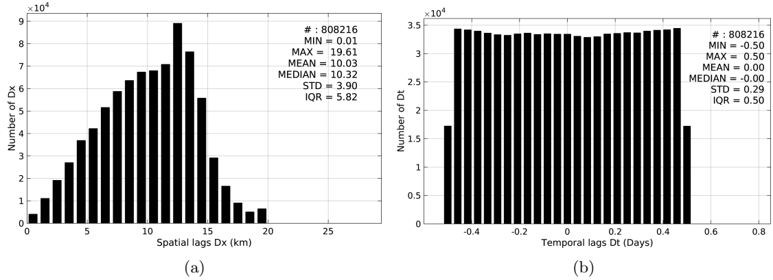
Figure 5: Histograms of the spatial (a) and temporal (b) lags between the time of the TSG-GOSUD-Research-vessel measurements and the date of the corresponding SMAP-L3-JPL-V4-8DAY-RUNNING-60KM SSS product.
