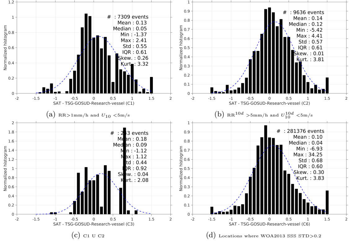
Figure 13: Normalized histogram of \Delta SSS (SMAP-L3-JPL-V4-8DAY-RUNNING-60KM - TSG-GOSUD-Research-vessel) for 6 different subdatasets corresponding to: RR > 1\text{mm/h} and U_{10} < 5\text{m/s} (a), RR^{10d} > 5\text{mm/h} and U_{10}^{10d} < 5\text{m/s} (b), C1 U C2 (c), Locations where WOA2013 SSS STD > 0.2 (d).
