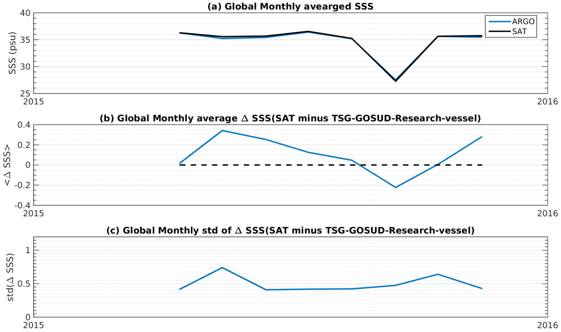
Figure 7: Time series of the monthly averaged mean SSS (top), mean \Delta \text{SSS} (Satellite - TSG-GOSUD-Research-vessel) and STD of \Delta \text{SSS} (Satellite - TSG-GOSUD-Research-vessel) over the SMOS coastal zone ( \pm 800\text{km} ) 60N-60S Pi-MEP region considering all match-ups collected by the Pi-MEP platform.
