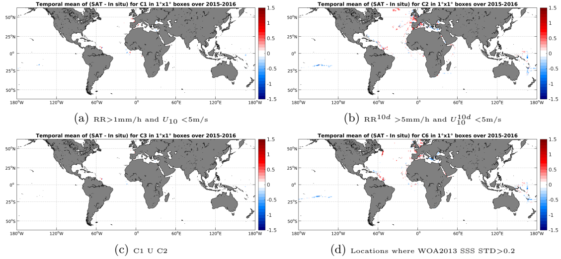
Figure 12: Temporal mean gridded over spatial boxes of size 1^\circ \times 1^\circ of \Delta SSS (SMAP-L3-JPL-V4-8DAY-RUNNING-60KM - TSG-GOSUD-Research-vessel) for 4 different subdatasets corresponding to: RR > 1 mm/h and U_{10} < 5 m/s (a), RR^{10d} > 5 mm/h and U_{10}^{10d} < 5 m/s (b), C1 U C2 (c), Locations where WOA2013 SSS STD > 0.2 (d).
