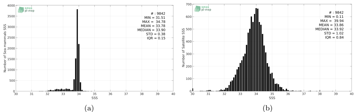
Figure 2: Histograms of SSS from Sea mammals (a) and SMAP-L3-JPL-V4-8DAY-RUNNING-60KM (b) considering all match-up pairs per bins of 0.1 over the SMOS coastal zone ( \approx 800 km) 60N-60S Pi-MEP region and for the full satellite product period.
