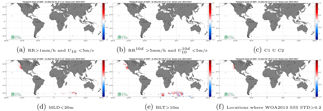
Figure 12: Temporal mean gridded over spatial boxes of size 1^\circ \times 1^\circ of \Delta SSS (SMAP-L3-JPL-V4-8DAY-RUNNING-60KM - Sea mammals) for 6 different subdatasets corresponding to: RR>1mm/h and U_{10} < 5m/s (a), RR^{10d} > 5mm/h and U_{10}^{10d} < 5m/s (b), C1 U C2 (c),MLD<20m (d),BLT>10m (e),Locations where WOA2013 SSS STD>0.2 (f).
