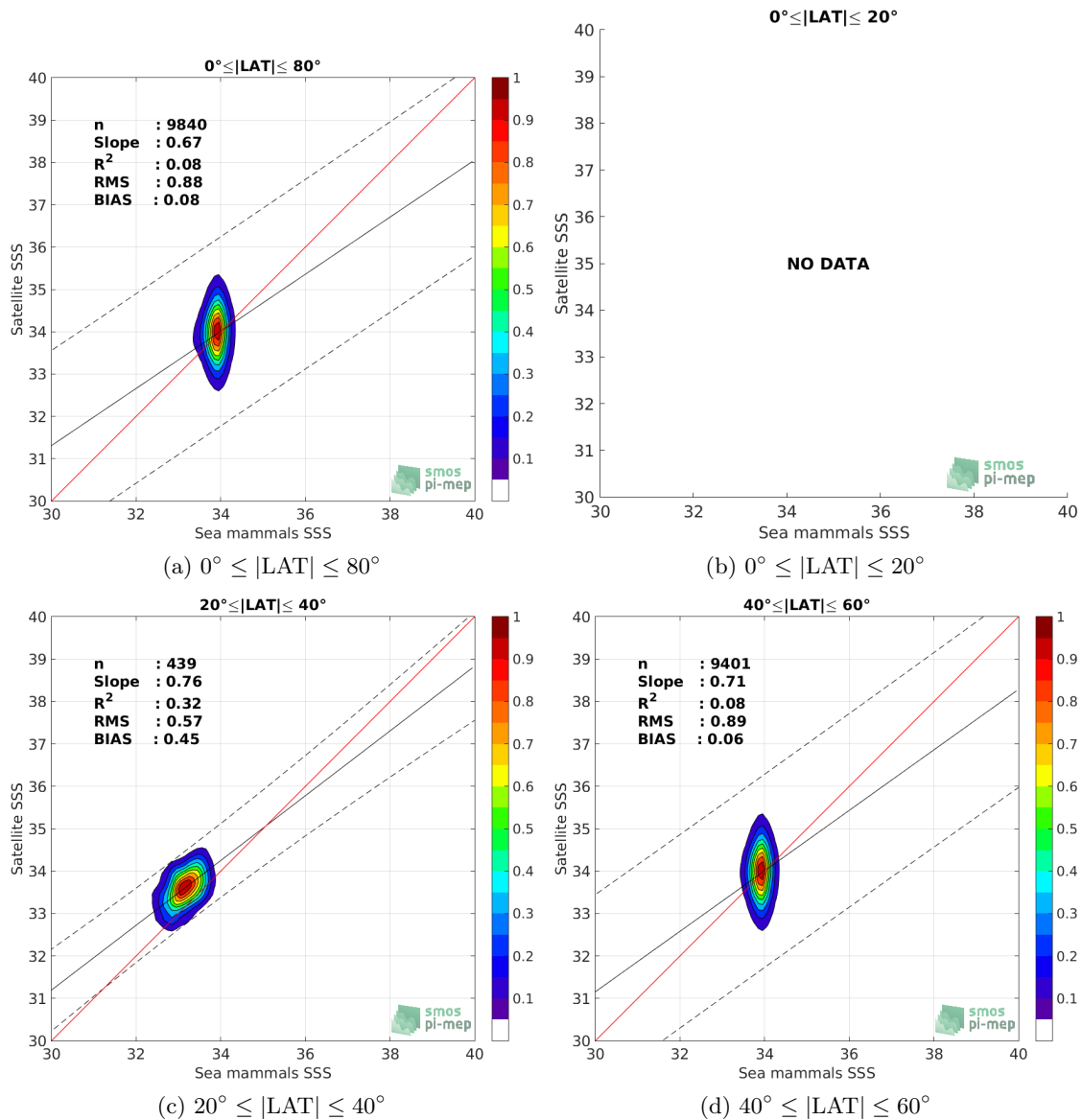
Figure 9: Contour maps of the concentration of SMAP-L3-JPL-V4-8DAY-RUNNING-60KM SSS (y-axis) versus Sea mammals SSS (x-axis) at match-up pairs for different latitudinal bands. For each plot, the red line shows x=y . The black thin and dashed lines indicate a linear fit through the data cloud and the \pm 95\% confidence levels, respectively. The number match-up pairs n , the slope and R^2 coefficient of the linear fit, the root mean square (RMS) and the mean bias between satellite and in situ data are indicated for each latitude band in each plots.
