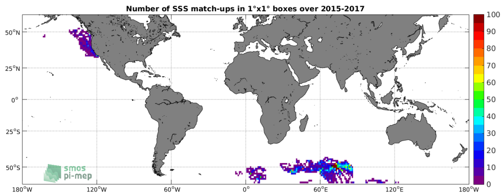
Figure 4: Number of SSS match-ups between Sea mammals SSS and the SMAP-L3-JPL-V4-8DAY-RUNNING-60KM SSS product for the SMOS coastal zone ( \approx 800\text{km} ) 60N-60S Pi-MEP region over 1^\circ \times 1^\circ boxes and for the full satellite product period.
