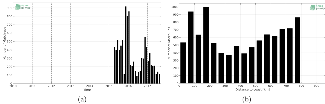
Figure 1: Number of match-ups between Sea mammals and SMAP-L3-JPL-V4-8DAY-RUNNING-60KM SSS as a function of time (a) and as function of the distance to coast (b) over the SMOS coastal zone ( \approx 800 km) 60N-60S Pi-MEP region and for the full satellite product period.
