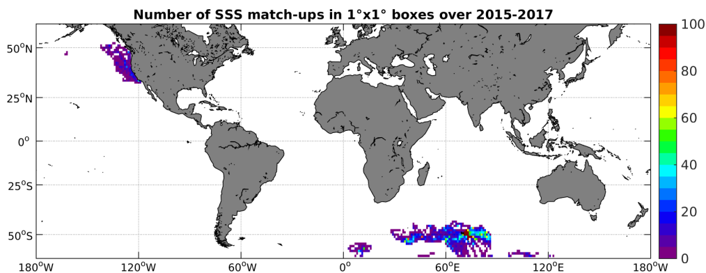
Figure 4: Number of SSS match-ups between Sea mammals SSS and the SMAP-L3-JPL-V4-8DAY-RUNNING-60KM SSS product for the SMOS coastal zone ( \pm 800\text{km} ) 60N-60S Pi-MEP region over 1^\circ \times 1^\circ boxes and for the full satellite product period.
