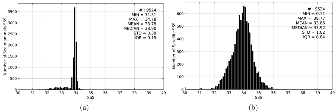
Figure 2: Histograms of SSS from Sea mammals (a) and SMAP-L3-JPL-V4-8DAY-RUNNING-60KM (b) considering all match-up pairs per bins of 0.1 over the SMOS coastal zone ( \approx 800\text{km} ) 60N-60S Pi-MEP region and for the full satellite product period.
