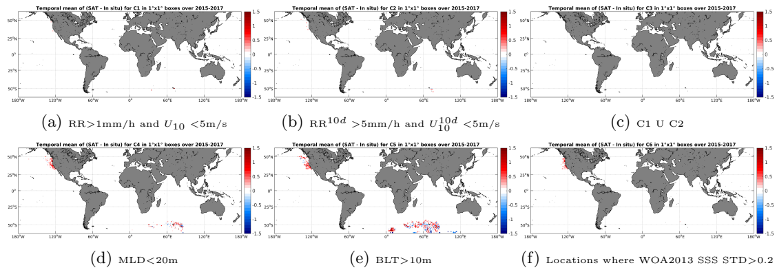
Figure 12: Temporal mean gridded over spatial boxes of size 1^\circ \times 1^\circ of \Delta SSS (SMAP-L3-JPL-V4-8DAY-RUNNING-60KM - Sea mammals) for 6 different subdatasets corresponding to: RR > 1mm/h and U_{10} < 5 m/s (a), RR^{10d} > 5 mm/h and U_{10}^{10d} < 5 m/s (b), C1 U C2 (c), MLD < 20m (d), BLT > 10m (e), Locations where WOA2013 SSS STD > 0.2 (f).
