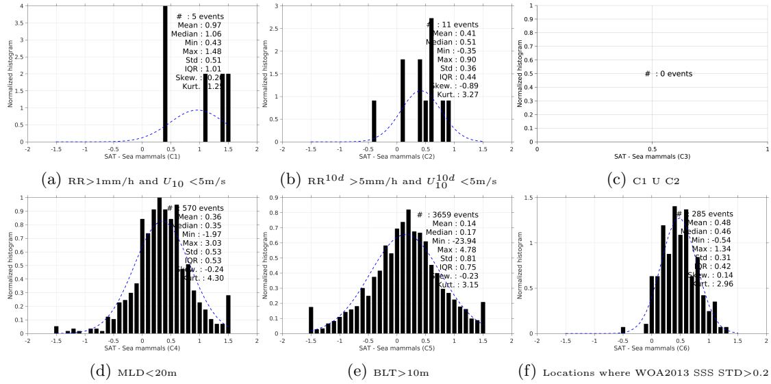
Figure 13: Normalized histogram of \Delta SSS (SMAP-L3-JPL-V4-8DAY-RUNNING-60KM - Sea mammals) for 6 different subdatasets corresponding to: RR>1mm/h and U_{10} < 5\text{m/s} (a), RR^{10d} > 5\text{mm/h} and U_{10}^{10d} < 5\text{m/s} (b), C1 U C2 (c), MLD<20m (d), BLT>10m (e), Locations where WOA2013 SSS STD>0.2 (f).
