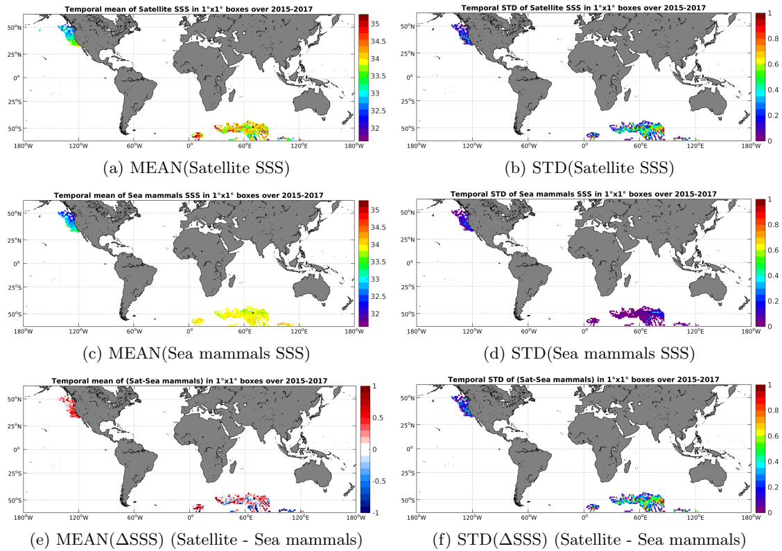
Figure 6: Temporal mean (left) and STD (right) of SSS from SMAP-L3-JPL-V4-8DAY-RUNNING-60KM (top), Sea mammals (middle), and of \Delta SSS (Satellite - Sea mammals). Only match-up pairs are used to generate these maps.
