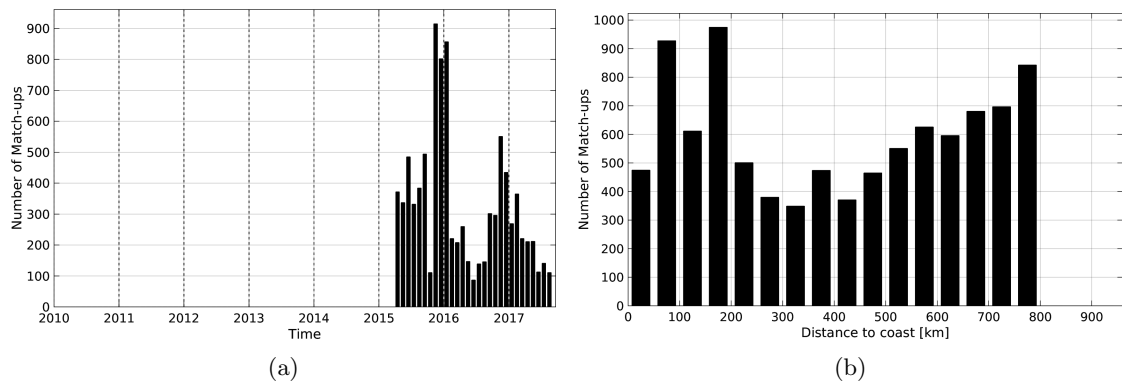
Figure 1: Number of match-ups between Sea mammals and SMAP-L3-JPL-V4-8DAY-RUNNING-60KM SSS as a function of time (a) and as function of the distance to coast (b) over the SMOS coastal zone ( \approx 800\text{km} ) 60N-60S Pi-MEP region and for the full satellite product period.
