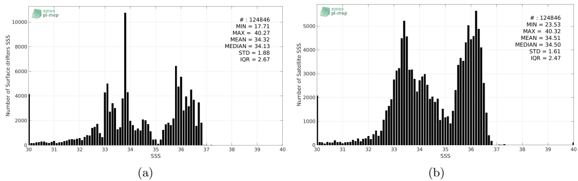
Figure 2: Histograms of SSS from Surface drifters (a) and SMAP-L3-JPL-V4-8DAY-RUNNING-60KM (b) considering all match-up pairs per bins of 0.1 over the SMOS coastal zone ( \approx 800\text{km} ) 60N-60S Pi-MEP region and for the full satellite product period.
