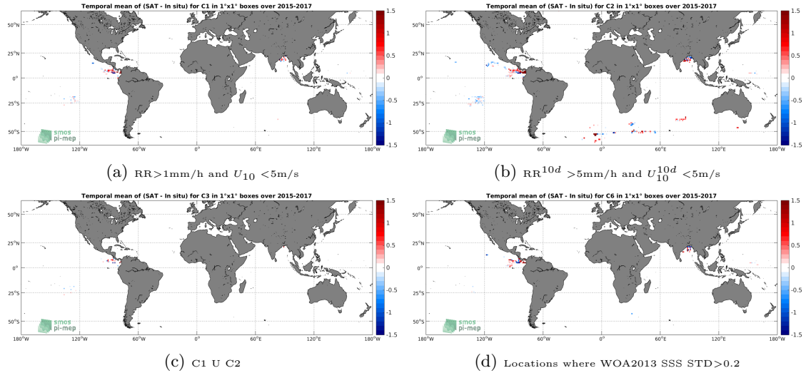
Figure 11: Temporal mean gridded over spatial boxes of size 1^\circ \times 1^\circ of \Delta SSS (SMAP-L3-JPL-V4-8DAY-RUNNING-60KM - Surface drifters) for 4 different subdatasets corresponding to: RR > 1\text{mm/h} and U_{10} < 5\text{m/s} (a), RR^{10d} > 5\text{mm/h} and U_{10}^{10d} < 5\text{m/s} (b), C1 U C2 (c), Locations where WOA2013 SSS STD > 0.2 (d).
