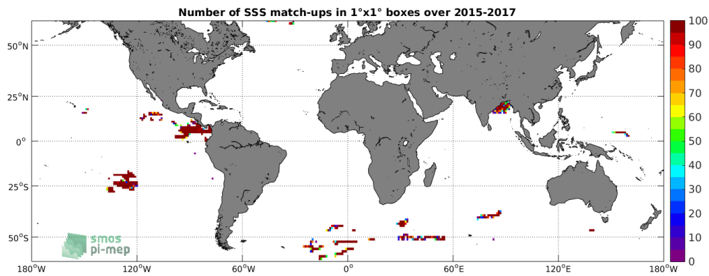
Figure 3: Number of SSS match-ups between Surface drifters SSS and the SMAP-L3-JPL-V4-8DAY-RUNNING-60KM SSS product for the SMOS coastal zone ( \approx 800\text{km} ) 60N-60S Pi-MEP region over 1^\circ \times 1^\circ boxes and for the full satellite product period.
