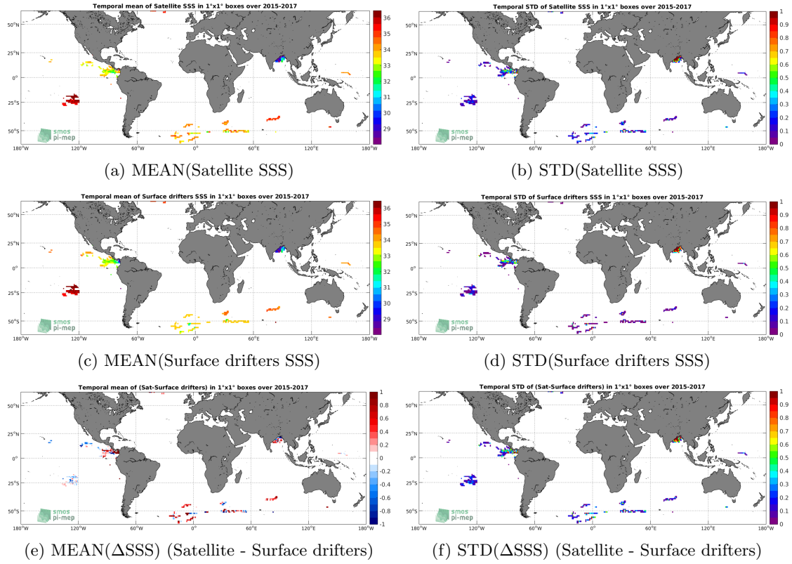
Figure 5: Temporal mean (left) and STD (right) of SSS from SMAP-L3-JPL-V4-8DAY-RUNNING-60KM (top), Surface drifters (middle), and of \Delta SSS (Satellite - Surface drifters). Only match-up pairs are used to generate these maps.
