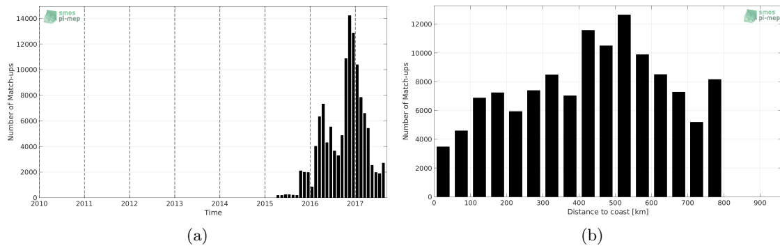
Figure 1: Number of match-ups between Surface drifters and SMAP-L3-JPL-V4-8DAY-RUNNING-60KM SSS as a function of time (a) and as function of the distance to coast (b) over the SMOS coastal zone ( \pm 800 km) 60N-60S Pi-MEP region and for the full satellite product period.
