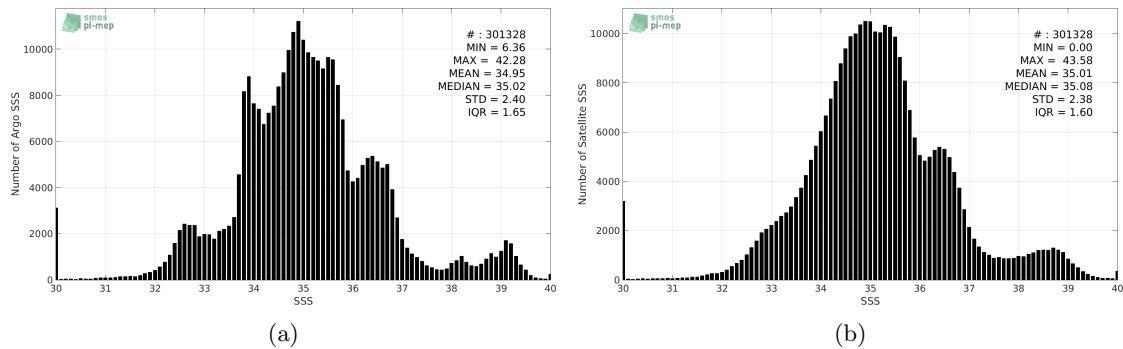
Figure 2: Histograms of SSS from Argo (a) and SMAP-L3-JPL-V4-8DAY-RUNNING-60KM (b) considering all match-up pairs per bins of 0.1 over the SMOS coastal zone ( \geq 800 km) 60N-60S Pi-MEP region and for the full satellite product period.
