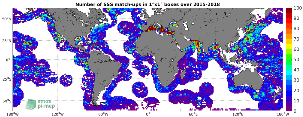
Figure 4: Number of SSS match-ups between Argo SSS and the SMAP-L3-JPL-V4-8DAY-RUNNING-60KM SSS product for the SMOS coastal zone ( \geq 800 km) 60N-60S Pi-MEP region over 1^\circ \times 1^\circ boxes and for the full satellite product period.
