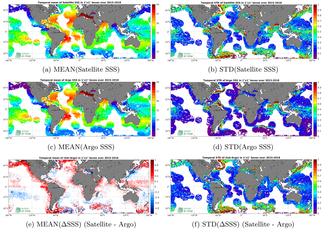
Figure 6: Temporal mean (left) and STD (right) of SSS from SMAP-L3-JPL-V4-8DAY-RUNNING-60KM (top), Argo (middle), and of \Delta SSS (Satellite - Argo). Only match-up pairs are used to generate these maps.
