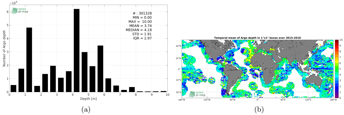
Figure 3: Histograms of the depth of the upper level SSS measurements from Argo in the Match-up DataBase for the SMOS coastal zone ( \geq 800 km) 60N-60S Pi-MEP region (a) and temporal mean spatial distribution of pressure of the in situ SSS data over 1^\circ \times 1^\circ boxes and for the full satellite product period (b).
