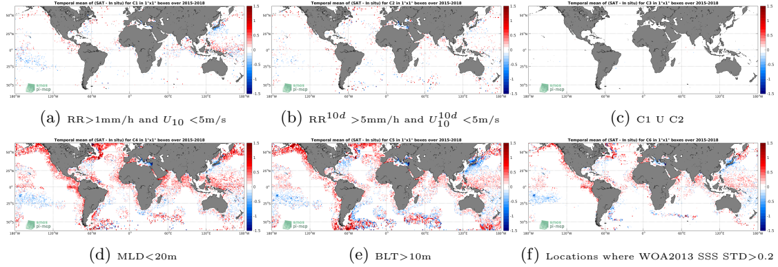
Figure 12: Temporal mean gridded over spatial boxes of size 1^\circ \times 1^\circ of \Delta SSS (SMAP-L3-JPL-V4-8DAY-RUNNING-60KM - Argo) for 6 different subdatasets corresponding to: RR>1mm/h and U_{10} < 5\text{m/s} (a), RR^{10d} > 5\text{mm/h} and U_{10}^{10d} < 5\text{m/s} (b), C1 U C2 (c), MLD<20m (d), BLT>10m (e), Locations where WOA2013 SSS STD>0.2 (f).
