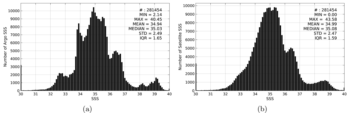
Figure 2: Histograms of SSS from Argo (a) and SMAP-L3-JPL-V4-8DAY-RUNNING-60KM (b) considering all match-up pairs per bins of 0.1 over the SMOS coastal zone ( \geq 800\text{km} ) 60N-60S Pi-MEP region and for the full satellite product period.
