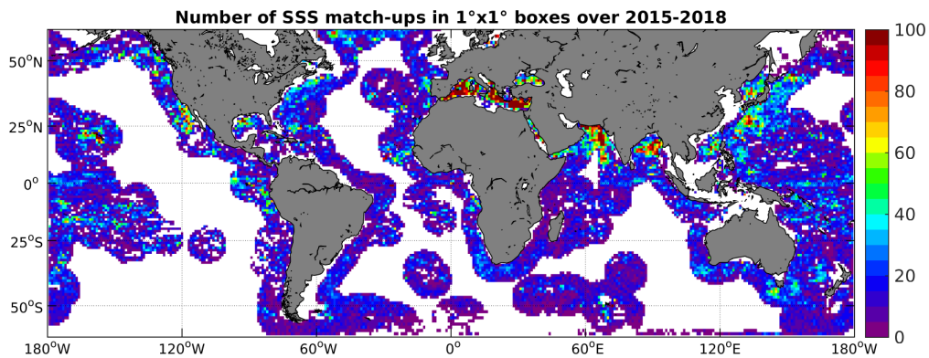
Figure 4: Number of SSS match-ups between Argo SSS and the SMAP-L3-JPL-V4-8DAY-RUNNING-60KM SSS product for the SMOS coastal zone ( \approx 800\text{km} ) 60N-60S Pi-MEP region over 1^\circ \times 1^\circ boxes and for the full satellite product period.
