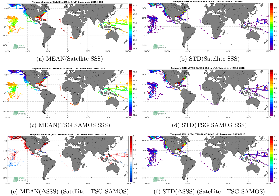
Figure 6: Temporal mean (left) and STD (right) of SSS from SMAP-L3-JPL-V4-MONTHLY-60KM (top), TSG-SAMOS (middle), and of \Delta SSS (Satellite - TSG-SAMOS). Only match-up pairs are used to generate these maps.
