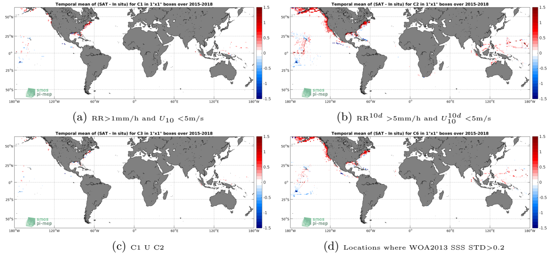
Figure 12: Temporal mean gridded over spatial boxes of size 1^\circ \times 1^\circ of \Delta SSS (SMAP-L3-JPL-V4-MONTHLY-60KM - TSG-SAMOS) for 4 different subdatasets corresponding to: RR > 1\text{mm/h} and U_{10} < 5\text{m/s} (a), RR^{10d} > 5\text{mm/h} and U_{10}^{10d} < 5\text{m/s} (b), C1 U C2 (c), Locations where WOA2013 SSS STD > 0.2 (d).
