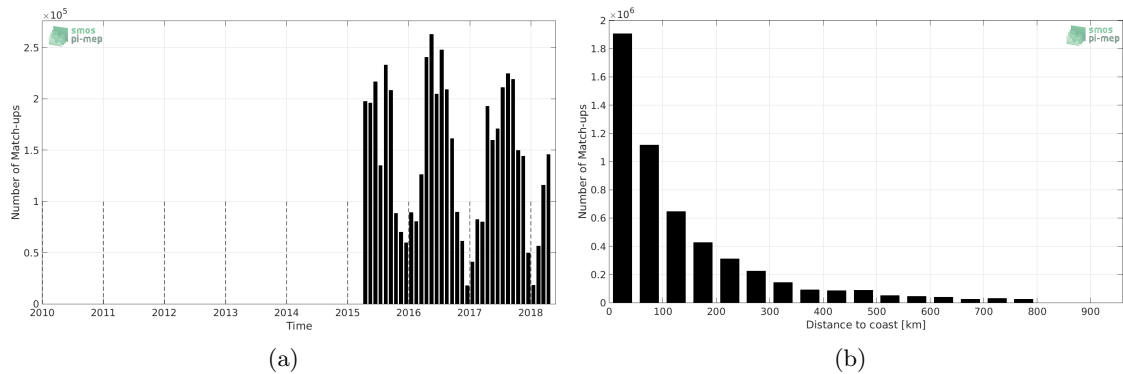
Figure 1: Number of match-ups between TSG-SAMOS and SMAP-L3-JPL-V4-MONTHLY-60KM SSS as a function of time (a) and as function of the distance to coast (b) over the SMOS coastal zone ( \leq 800 km) 60N-60S Pi-MEP region and for the full satellite product period.
