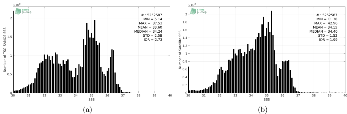
Figure 2: Histograms of SSS from TSG-SAMOS (a) and SMAP-L3-JPL-V4-MONTHLY-60KM (b) considering all match-up pairs per bins of 0.1 over the SMOS coastal zone ( \leq 800 km) 60N-60S Pi-MEP region and for the full satellite product period.
