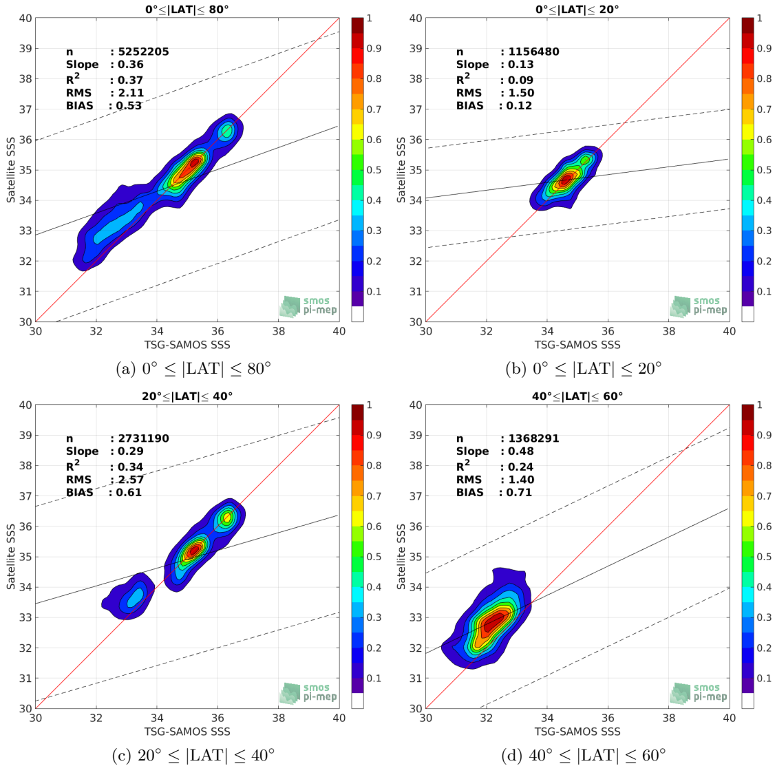
Figure 9: Contour maps of the concentration of SMAP-L3-JPL-V4-MONTHLY-60KM SSS (y-axis) versus TSG-SAMOS SSS (x-axis) at match-up pairs for different latitude bands. For each plot, the red line shows x=y . The black thin and dashed lines indicate a linear fit through the data cloud and the \pm 95\% confidence levels, respectively. The number match-up pairs n , the slope and R^2 coefficient of the linear fit, the root mean square (RMS) and the mean bias between satellite and in situ data are indicated for each latitude band in each plots.
