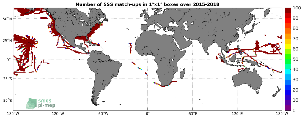
Figure 4: Number of SSS match-ups between TSG-SAMOS SSS and the SMAP-L3-JPL-V4-MONTHLY-60KM SSS product for the SMOS coastal zone ( \approx 800 km) 60N-60S Pi-MEP region over 1^\circ \times 1^\circ boxes and for the full satellite product period.
