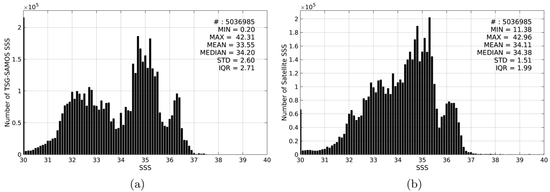
Figure 2: Histograms of SSS from TSG-SAMOS (a) and SMAP-L3-JPL-V4-MONTHLY-60KM (b) considering all match-up pairs per bins of 0.1 over the SMOS coastal zone ( \pm 800\text{km} ) 60N-60S Pi-MEP region and for the full satellite product period.
