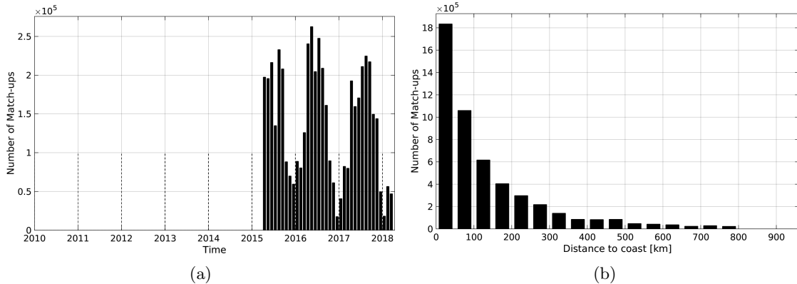
Figure 1: Number of match-ups between TSG-SAMOS and SMAP-L3-JPL-V4-MONTHLY-60KM SSS as a function of time (a) and as function of the distance to coast (b) over the SMOS coastal zone ( \pm 800\text{km} ) 60N-60S Pi-MEP region and for the full satellite product period.
